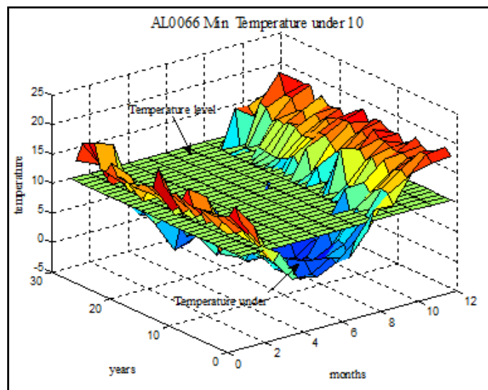
Figure (3f): The area profile of min. T < 10 for station AL0066
