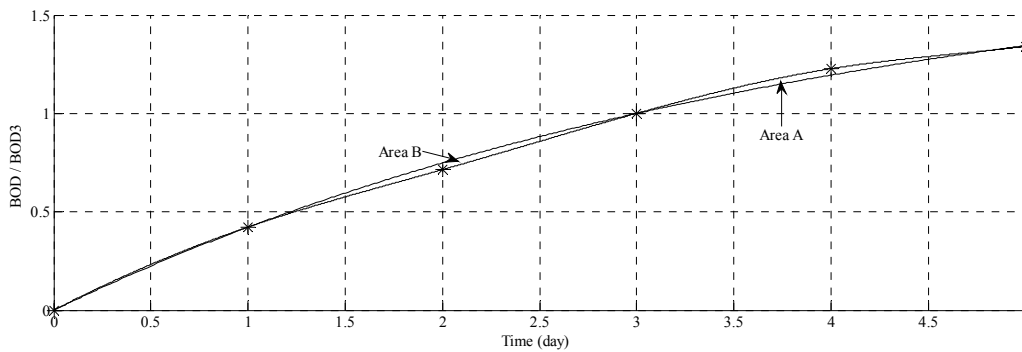
Figure (4): Cubic spline curve connecting the dimensionless BOD data based on BOD_3 (set no. 3 in Table 3) and the corresponding theoretical curve that has the same area under it. Area A and area B should be equal
