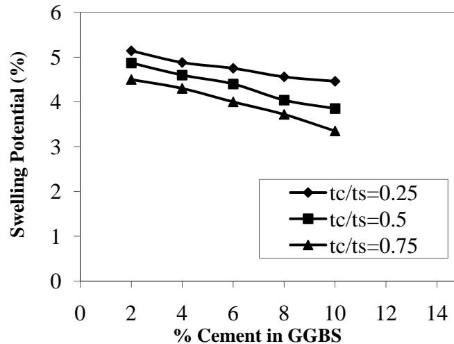
Figure (3): Variation of swelling potential with % of cement in GGBS
