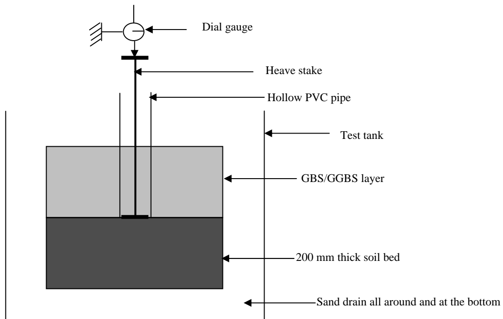
Figure (1): Experimental set-up for swelling studies
