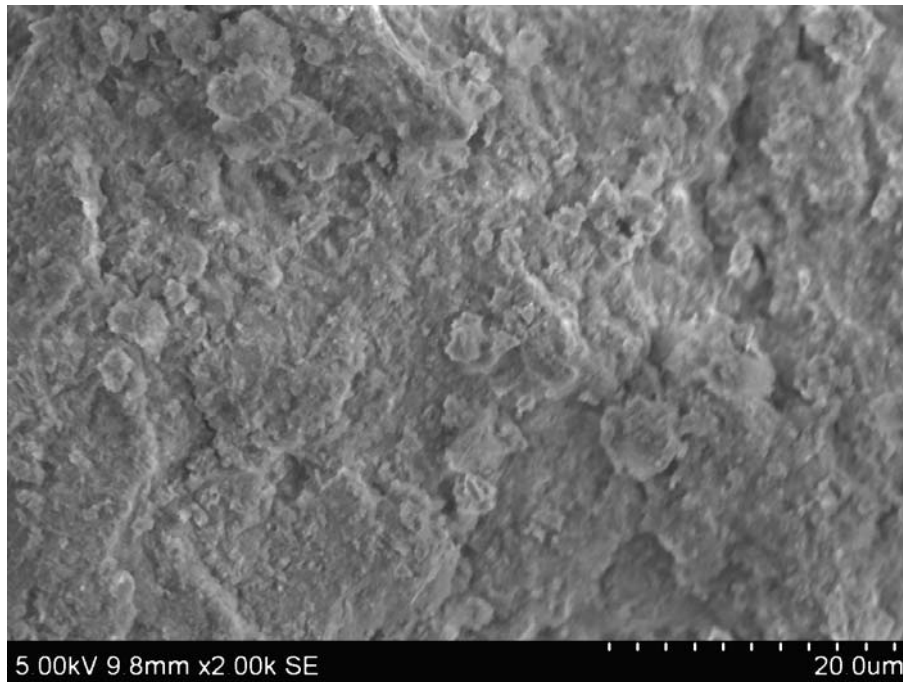
Figure (8): Scanning electron micrograph of GGBS stabilized with 4% cement
