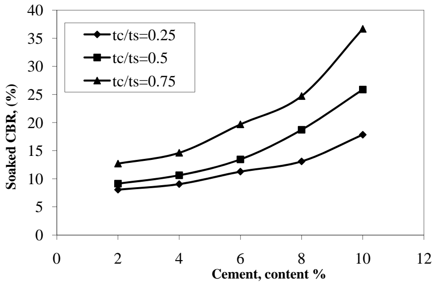
Figure (4): Variation of soaked CBR for different cement contents in GBS
