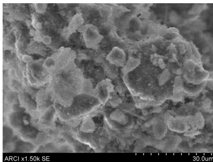
Figure (7): Scanning electron micrograph of GGBS stabilized with 2% cement
