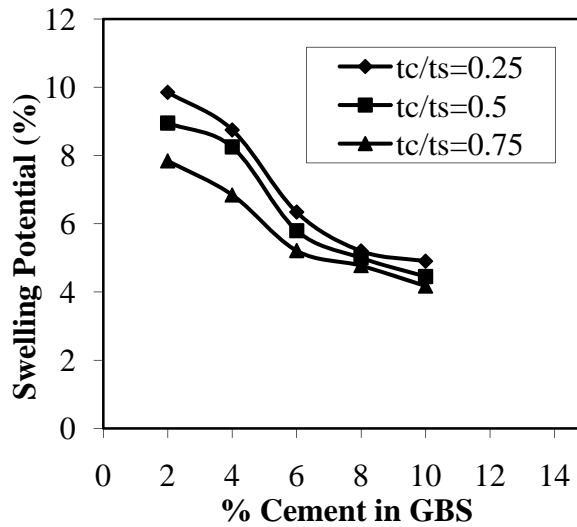
Figure (2): Variation of swelling potential with % of cement in GBS
