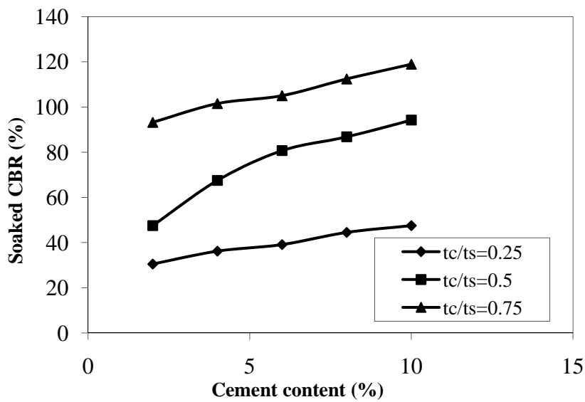
Figure (5): Variation of soaked CBR for different cement contents in GGBS
