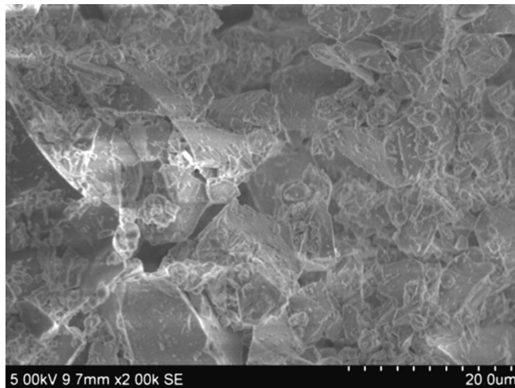
Figure (6): Scanning electron micrograph of GGBS
