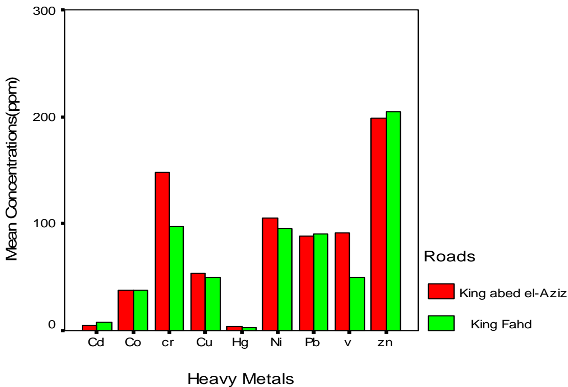
Figure 3: Mean Values of Heavy Metal Concentrations along Two Roads in Hail
