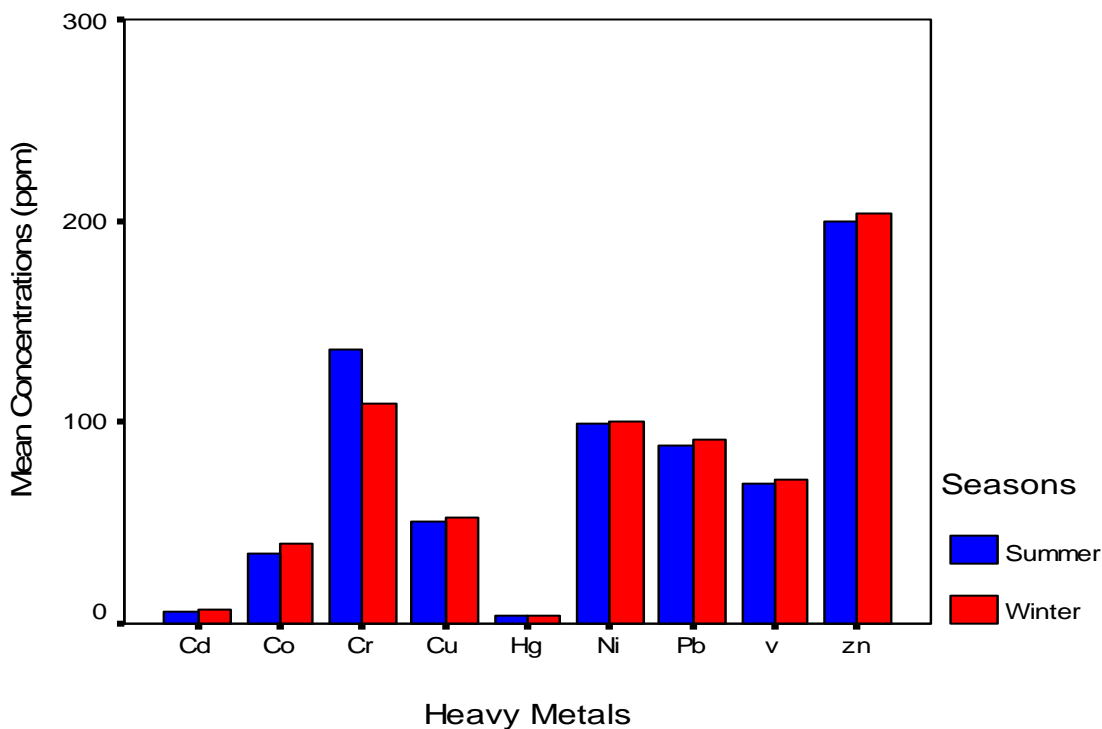
Figure 2: Mean Values of Heavy Metal Concentrations in Summer and Winter Seasons in Hail
