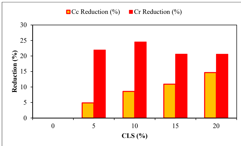
Figure (10): Reduction percentage in Cc and Cr values after utilizing CLS as a stabilizer for LPC soil
