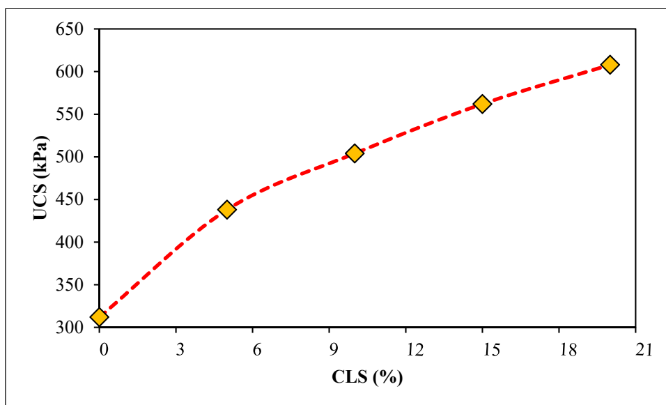
Figure (6): Effect of CLS content on the UCS value for the stabilized LPC soil
