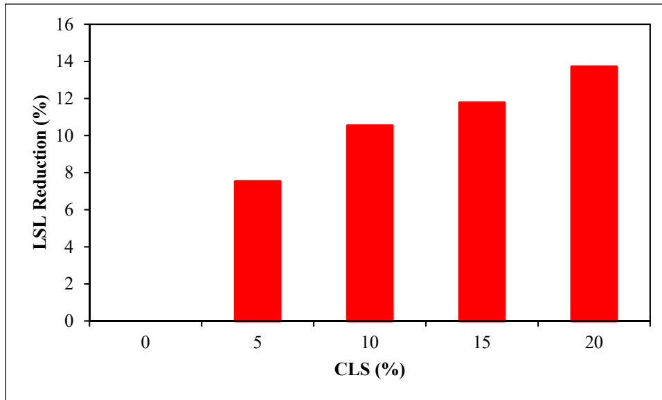
Figure (5): Reduction percentage in LSL value after utilizing CLS as a stabilizer for LPC soil
