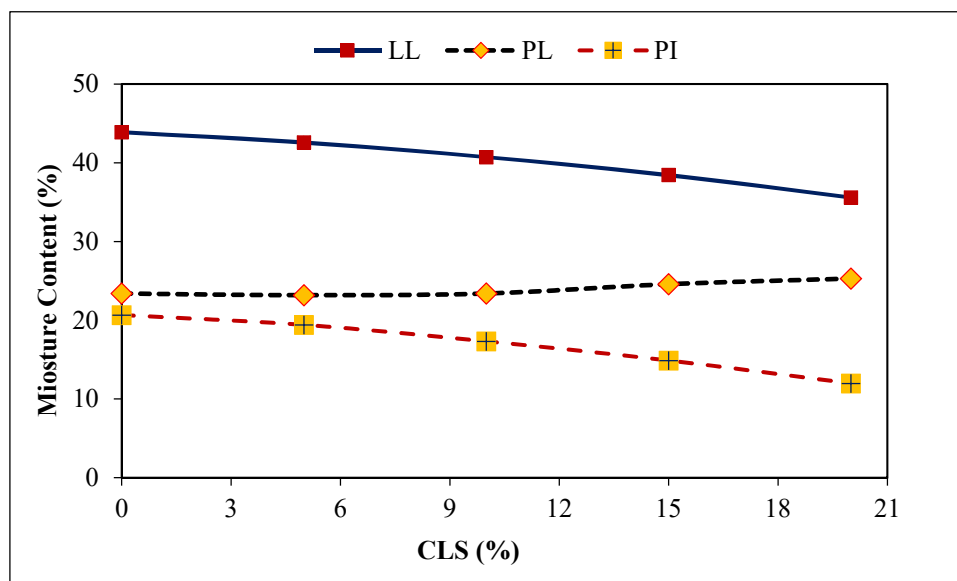
Figure (2): Effect of CLS content on the consistency parameters (LL, PL and PI) of the stabilized LPC soil
