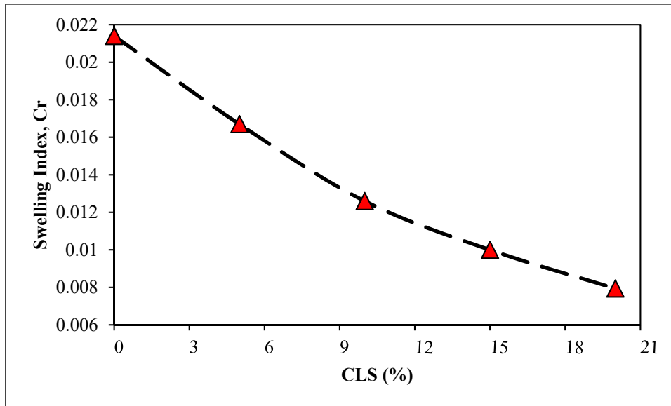
Figure (9): Effect of CLS content on the Cr value for the stabilized LPC soil
