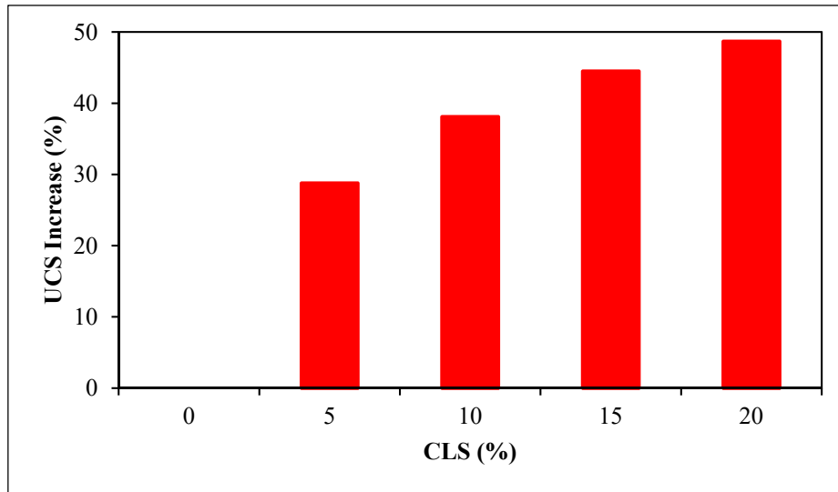
Figure (7): Increase percentage in UCS value after utilizing CLS as a stabilizer for LPC soil
