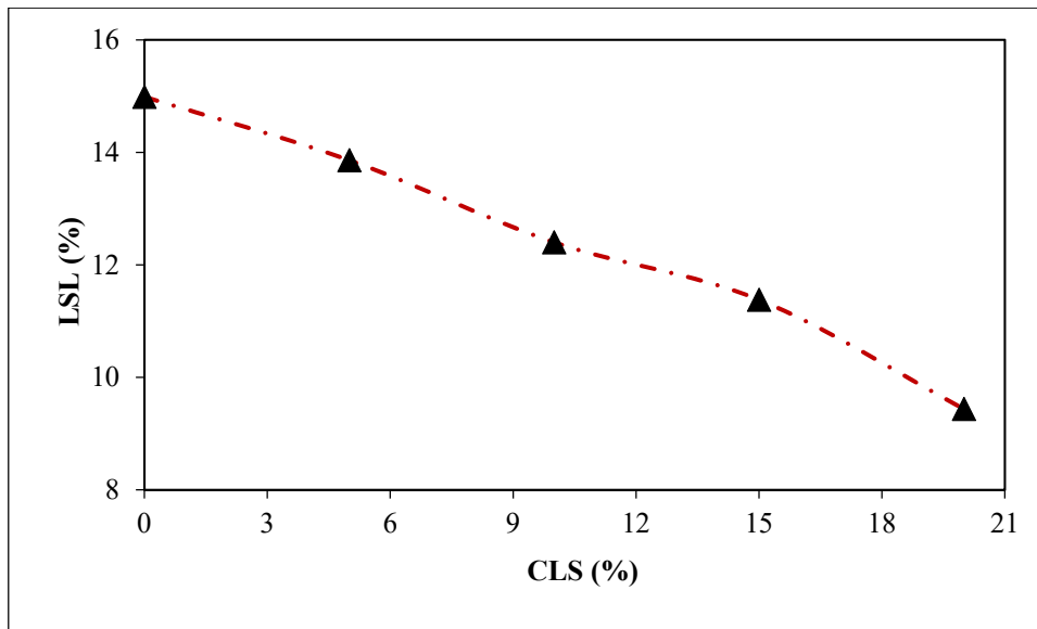
Figure (4): Effect of CLS content on the LSL value of the stabilized LPC soil
