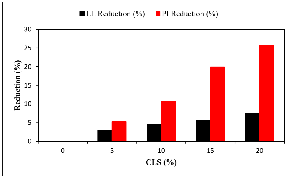
Figure (3): Reduction percentage in LL and PI values after utilizing CLS as a stabilizer for LPC soil
