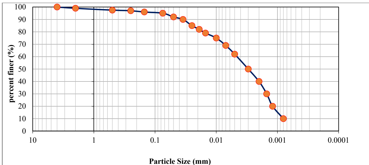
Figure (1): Grain-size distribution for the tested sample (Bakrajo LPC soil)
