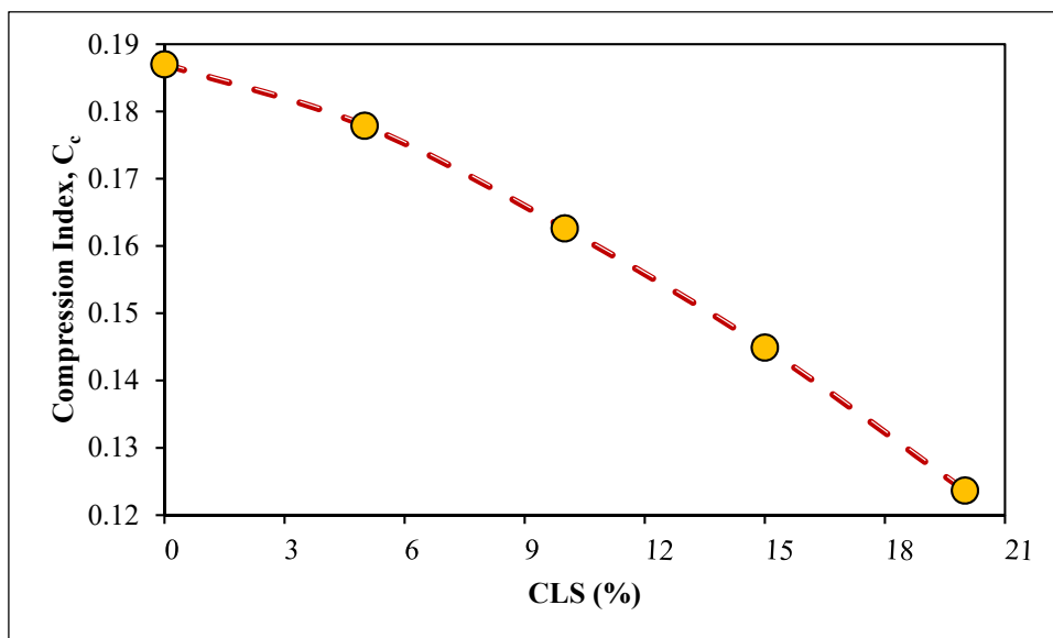
Figure (8): Effect of CLS content on the C_c value for the stabilized LPC soil
