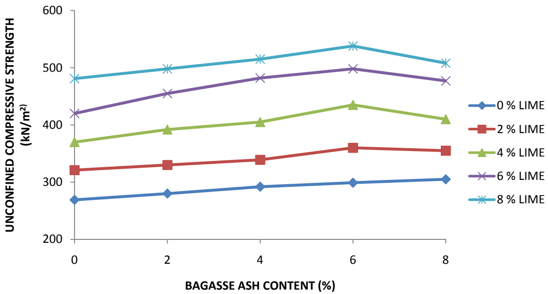
Figure (4): Variation of unconfined compressive strength of lime stabilized lateritic soil with bagasse ash content (7-day curing period)
