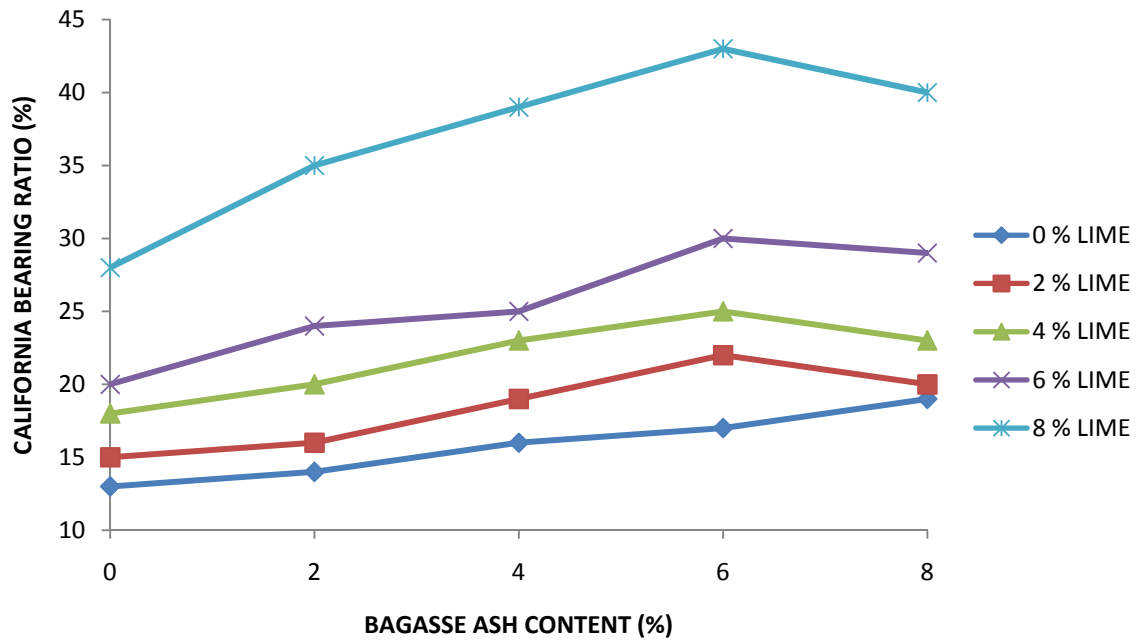
Figure (7): Variation of unsoaked California bearing ratio of lime stabilized lateritic soil with bagasse ash content
