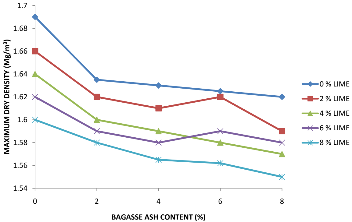
Figure (2): Variation of maximum dry density of lime stabilized lateritic soil with bagasse ash content
