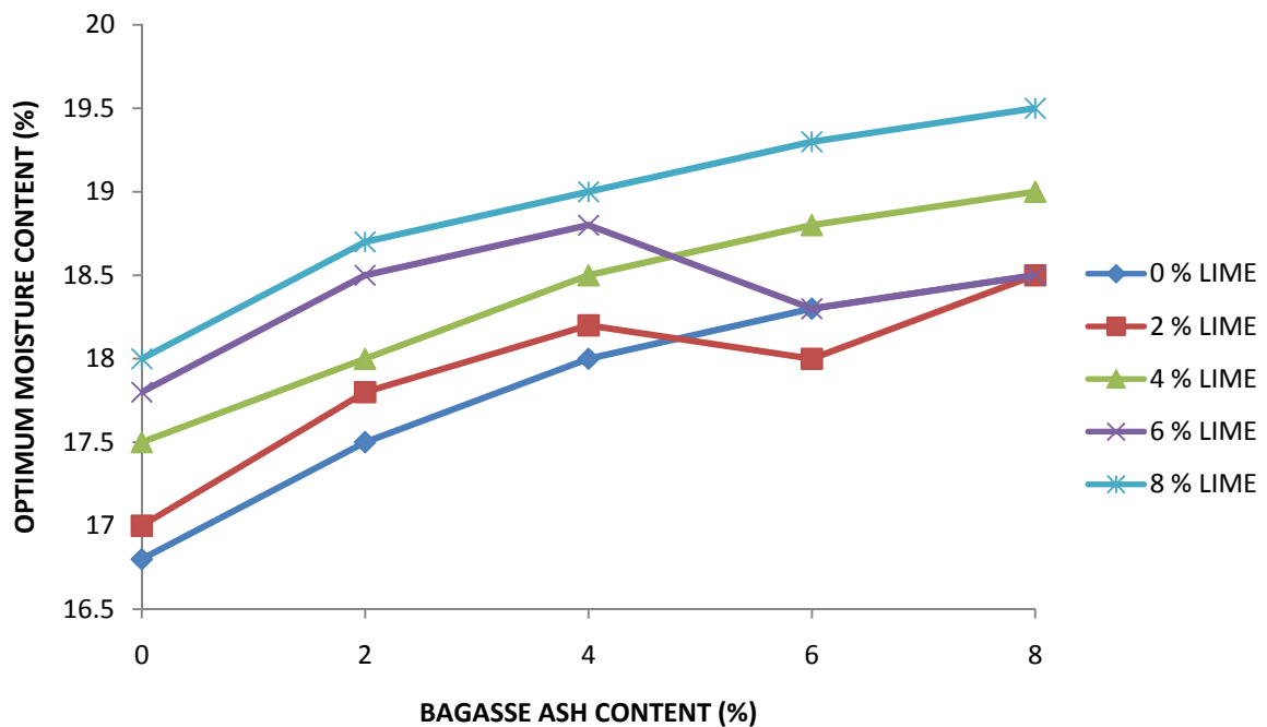
Figure (3): Variation of optimum moisture content of lime stabilized lateritic soil with bagasse ash content
