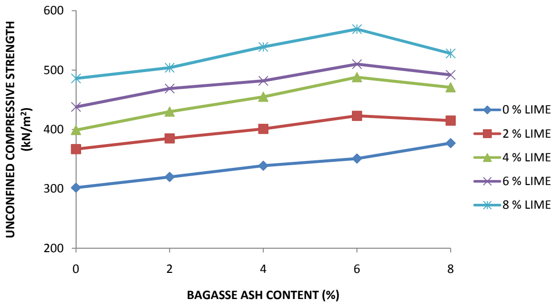
Figure (5): Variation of unconfined compressive strength of lime stabilized lateritic soil with bagasse ash content (14-day curing period)
