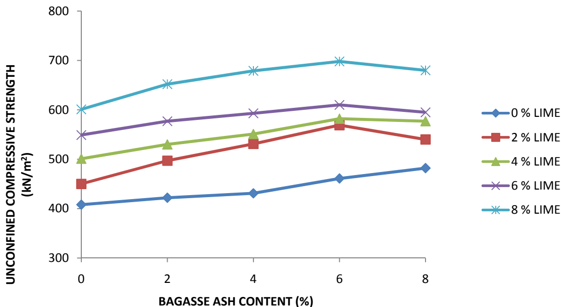
Figure (6): Variation of unconfined compressive strength of lime stabilized lateritic soil with bagasse ash content (28-day curing period)
