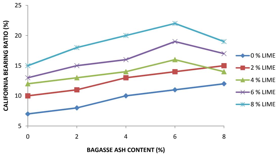
Figure (8): Variation of soaked California bearing ratio of lime stabilized lateritic soil with bagasse ash content
