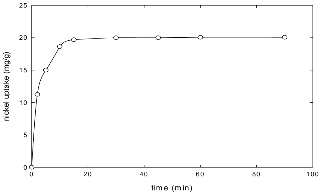
Fig. (5): Effects of shaking time on nickel removal (initial nickel ions concentration = 100 ppm, pH = 6.0 and mass of palm tree leaves = 0.08 g).
