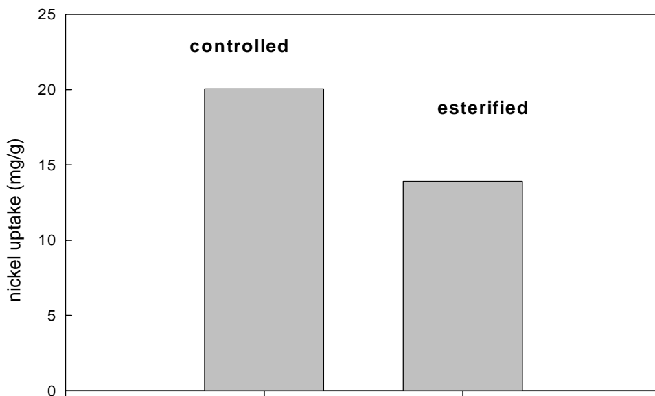
Fig. (8): Effect of blocking the carboxyl groups on the biosorption of nickel on palm tree leaves (initial nickel ions concentration = 100 ppm, pH = 6.0 and mass of palm tree leaves = 0.08 g).
