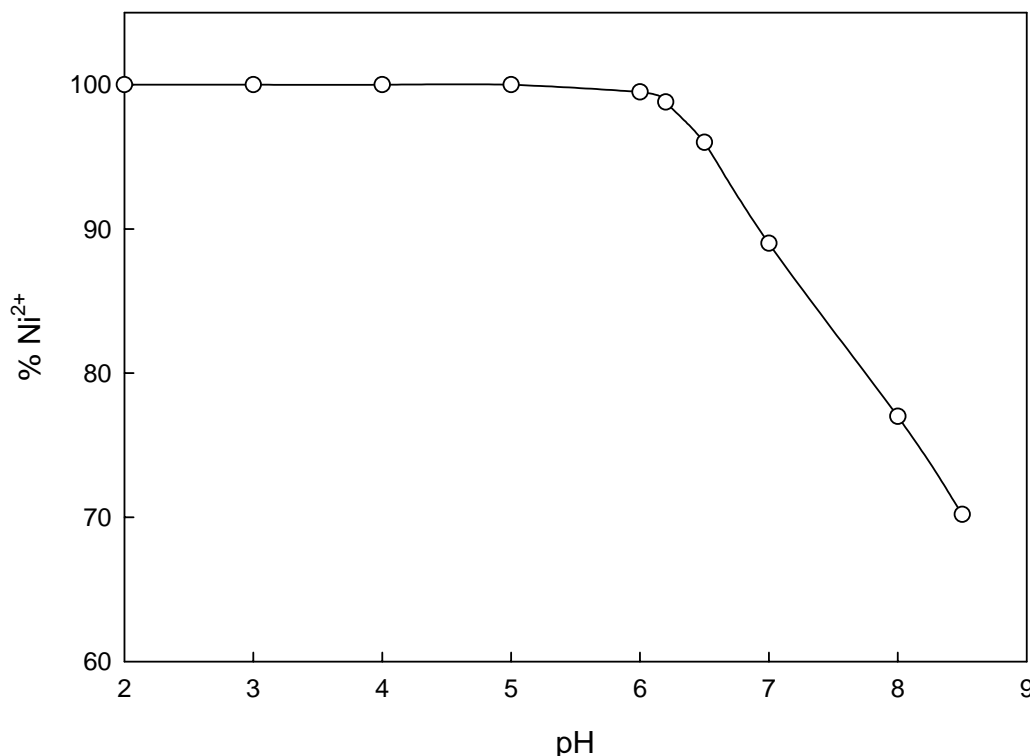
Fig. (1): Effect of pH on nickel speciation (initial nickel ions concentration = 100 ppm).
