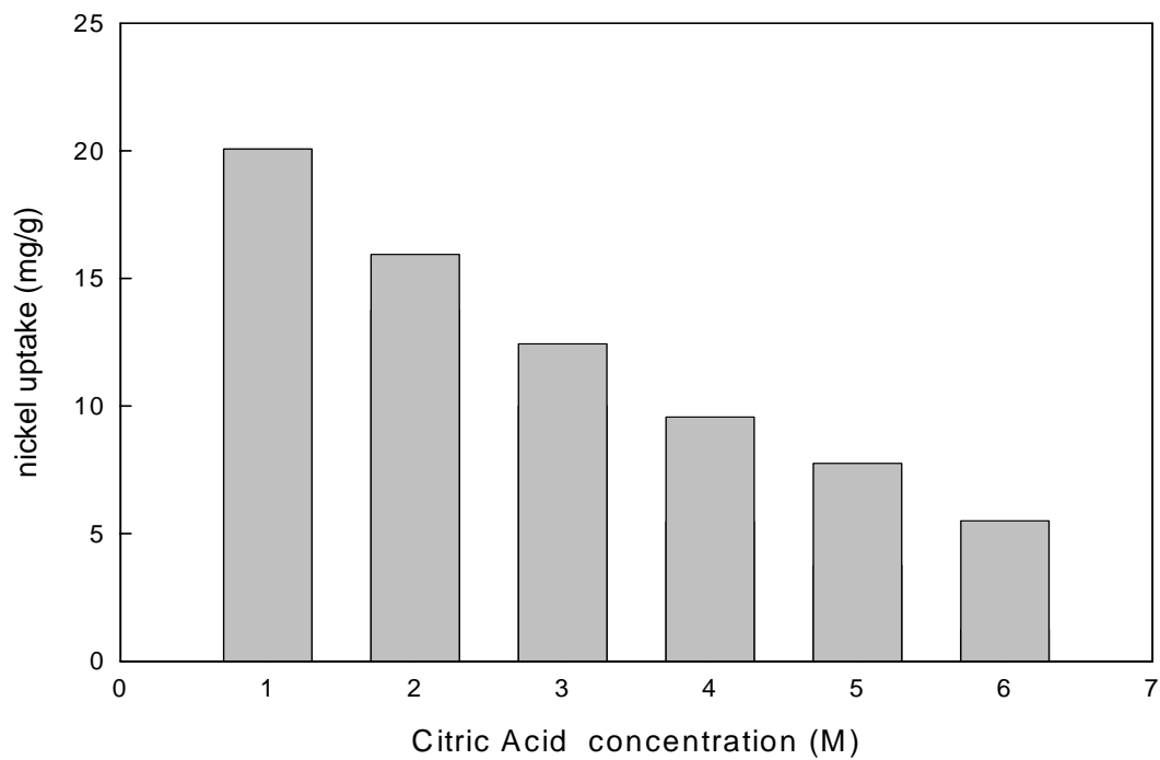
Fig. 10. Effect of citric acid on the biosorption of nickel on palm tree leaves (initial nickel ions concentration=100 ppm, pH = 6.0 and mass of palm tree leaves = 0.08 g).
