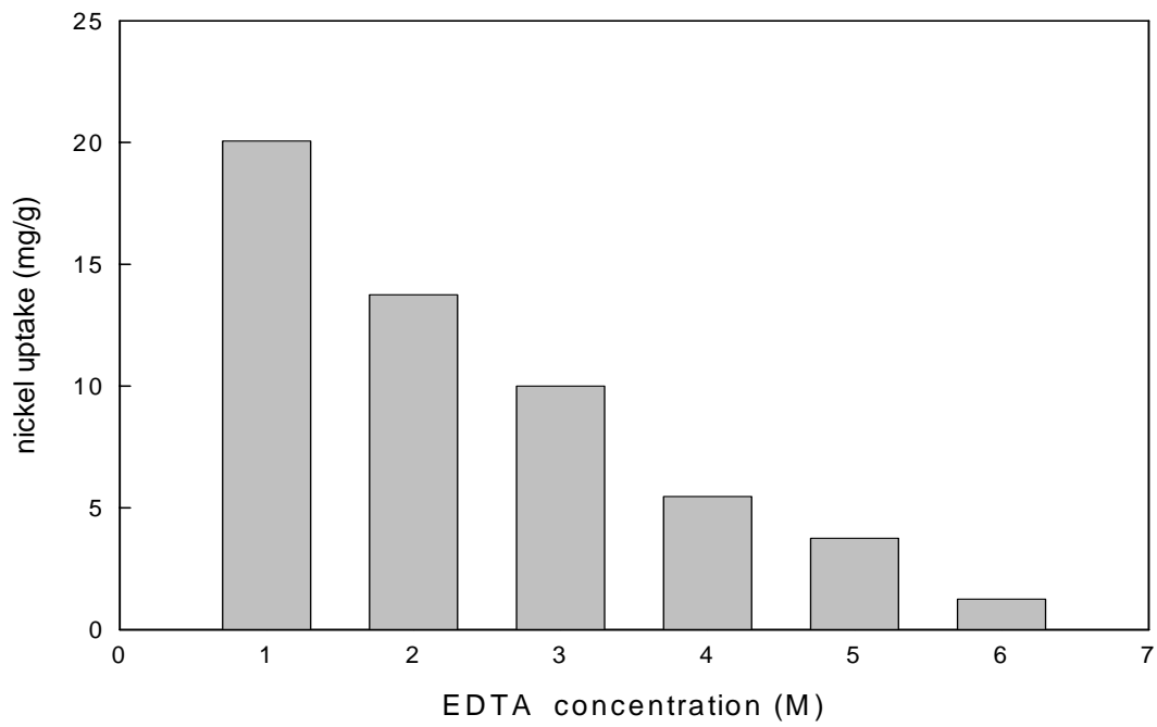
Fig. (9): Effect of EDTA on the biosorption of nickel on palm tree leaves (initial nickel ions concentration = 100 ppm, pH = 6.0 and mass of palm tree leaves = 0.08 g).
