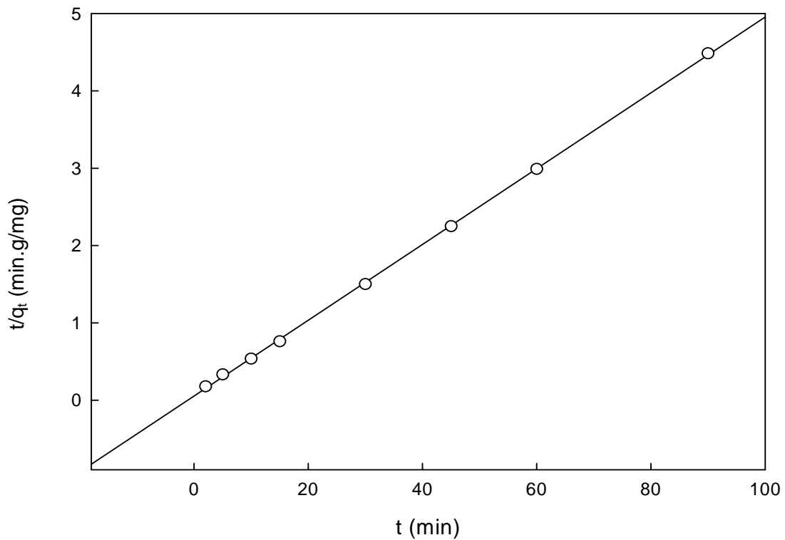
Fig. (6): Kinetics of biosorption of nickel on palm tree leaves (initial nickel ions concentration = 100 ppm, pH = 6.0 and mass of palm tree leaves = 0.08 g).
