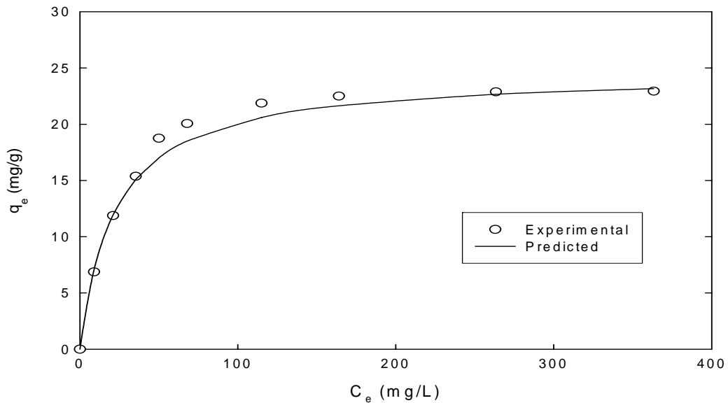
Fig. (4): Experimental and predicted isotherms of nickel ions biosorbed on palm tree leaves (pH = 6.0 and mass of palm tree leaves = 0.08 g).
