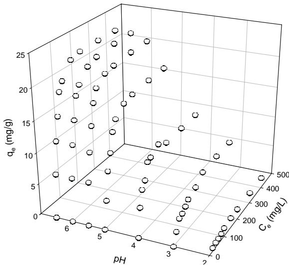
Fig. (3): Effect of pH on nickel removal (initial nickel ions concentration=100 ppm, mass of palm tree leaves=0.08g).
