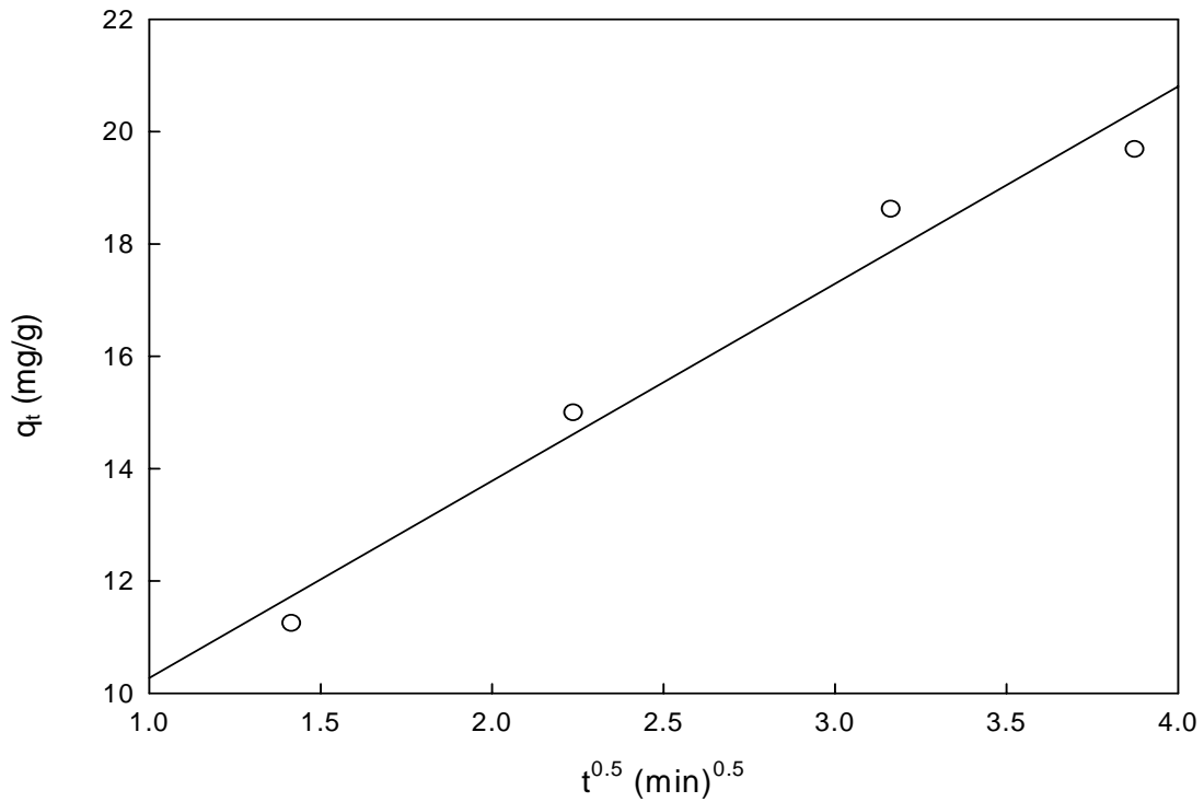
Fig. (7): Investigation of the contribution of intraparticle diffusion in the biosorption process of nickel on palm tree leaves: Application of the Weber and Morris equation (initial nickel ions concentration = 100 ppm, pH = 6.0 and mass of palm tree leaves = 0.08 g).
