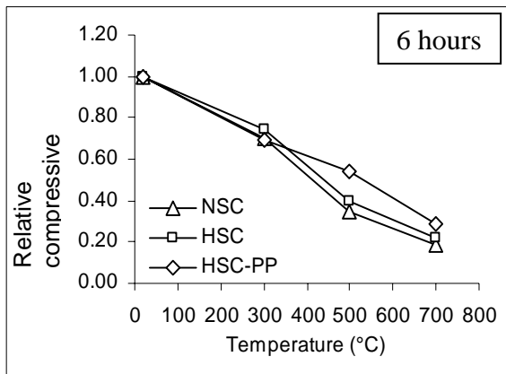
Figure (4-c): Relative Residual Compressive Strengths of Heated Concretes for 6 Hours.
