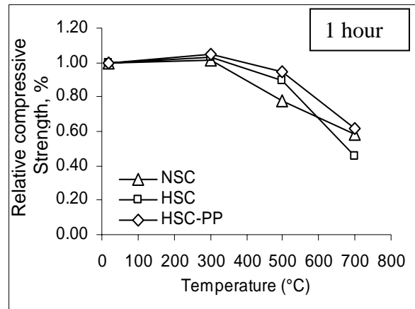
Figure (4-a): Relative Residual Compressive Strength of Heated Concretes for 1 Hour.
