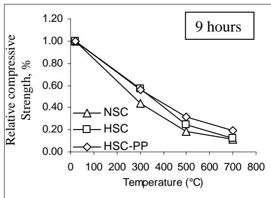
Figure (4-d): Relative Residual Compressive Strengths of Heated Concretes for 9 Hours.
