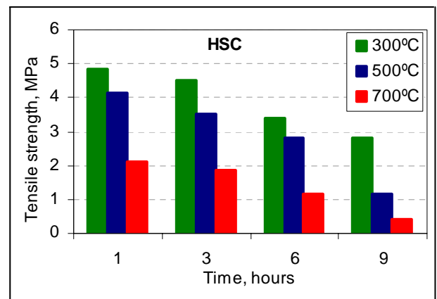
Figure (6-b): Residual Flexural Tensile Strength of HSC Heated Concretes.
