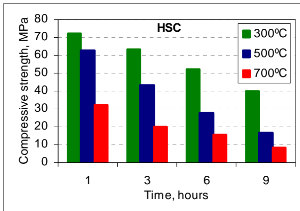
Figure (3-b): Residual Compressive Strengths of HSC Heated Concretes.
