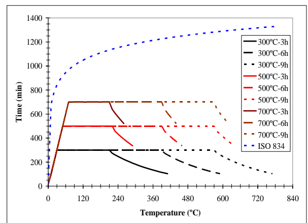
Figure (2): Experimental Time-Temperature Curve Compared with the ISO 834 Curve.
