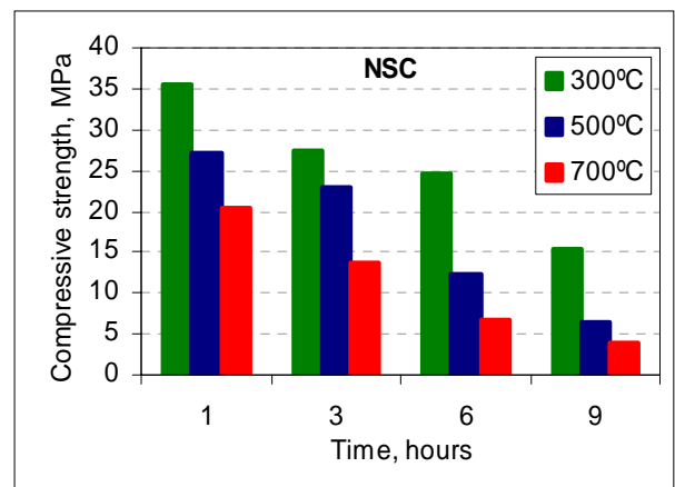
Figure (3-a): Residual Compressive Strengths of NSC Heated Concretes.
