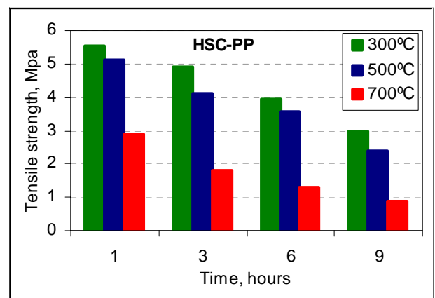
Figure (6-c): Residual Flexural Tensile Strength of HSC-PP Heated Concretes.
