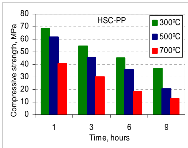
Figure (3-b): Residual Compressive Strengths of HSC Heated Concretes.
