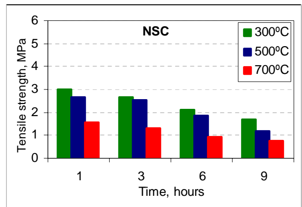
Figure (6-a): Residual Flexural Tensile Strength of NSC Heated Concretes.
