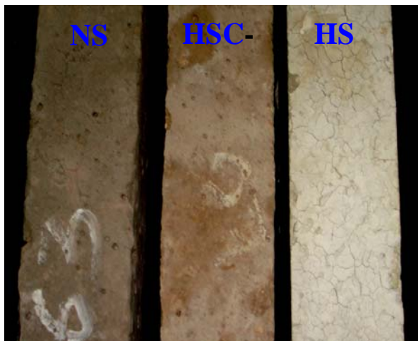
Figure (5): Surface Character of NSC, HSC and HSC-PP Heated at 700°C for 3 Hours.
