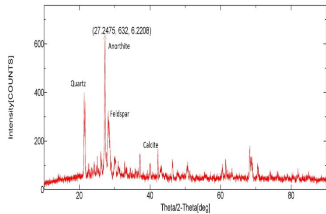
Figure (4): X-ray diffraction pattern of optimized quaternary blended concrete mix
