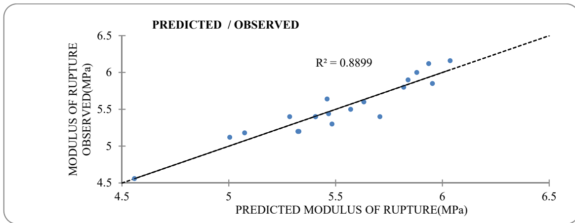
Figure (1): Goodness of fit for the non-linear regression model
