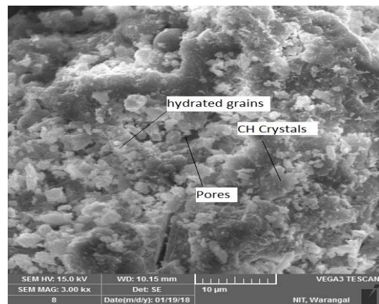
Figure (6): SEM image of cement hydration for optimized quaternary blended SCM mix
