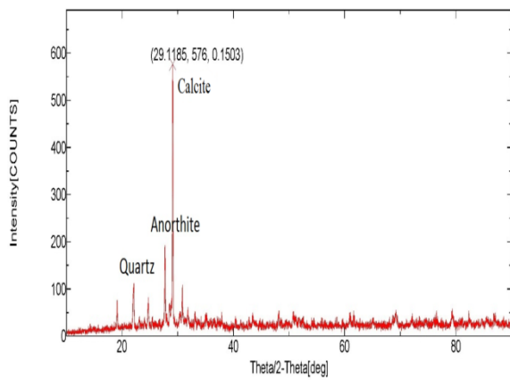
Figure (3): X-ray diffraction pattern of the control sample
