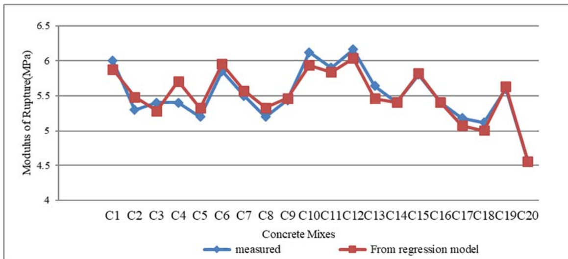
Figure (2): Modulus of rupture measured and computed from the model
