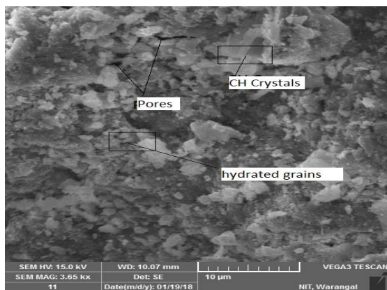
Figure (5): SEM image of cement hydration for the concrete control sample
