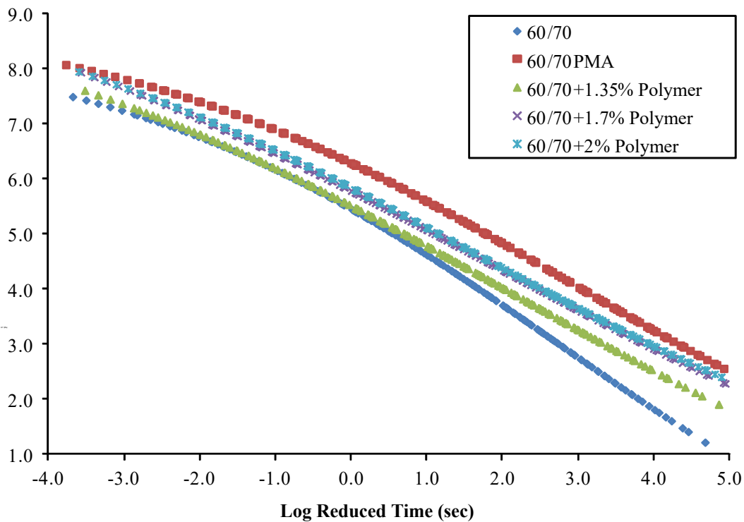
Figure (2): Master curves for Attock 60/70 and its PMA samples using Witzcak sigmoid function
