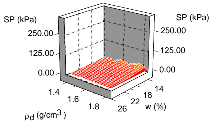
Figure 15: Swell pressure for treated JUST soil, 2% cement content and 7-day curing
