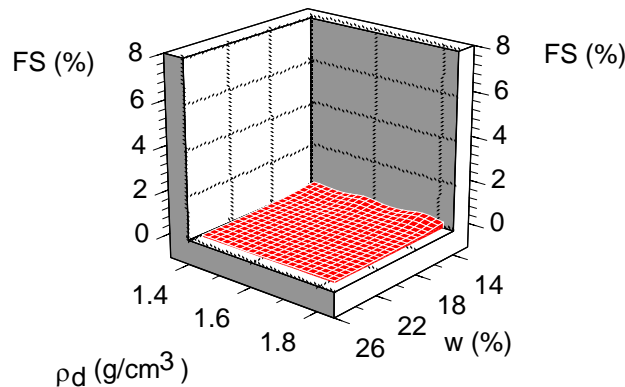
Figure 10: Free swell for treated JUST soil, 2% cement content and 28-day curing
