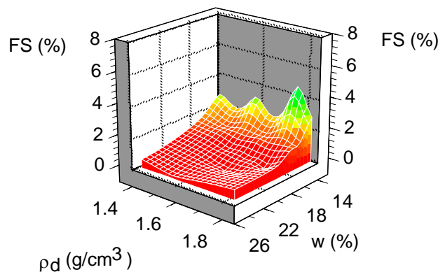
Figure 7: Free swell for treated JUST soil, 1% cement content and 7-day curing
