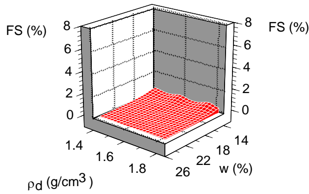
Figure 11: Free swell for treated JUST soil, 3% cement content and 7-day curing
