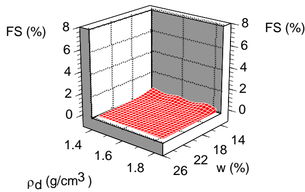
Figure 12: Free swell for treated JUST soil, 4% cement content and 7-day curing
