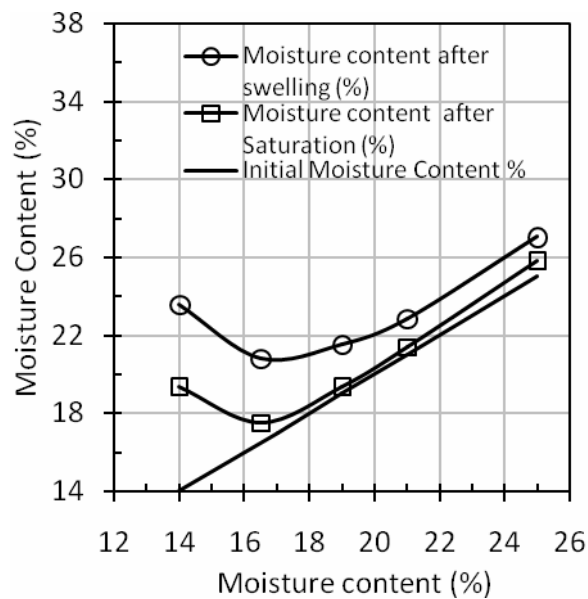
Figure 6: Moisture content at saturation and at the end of swelling for points corresponding to the modified compaction curve for JUST soil, (Al-Sharqi, 1993)
