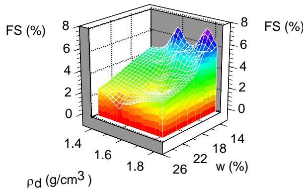
Figure 3: Free swell for natural JUST soil
