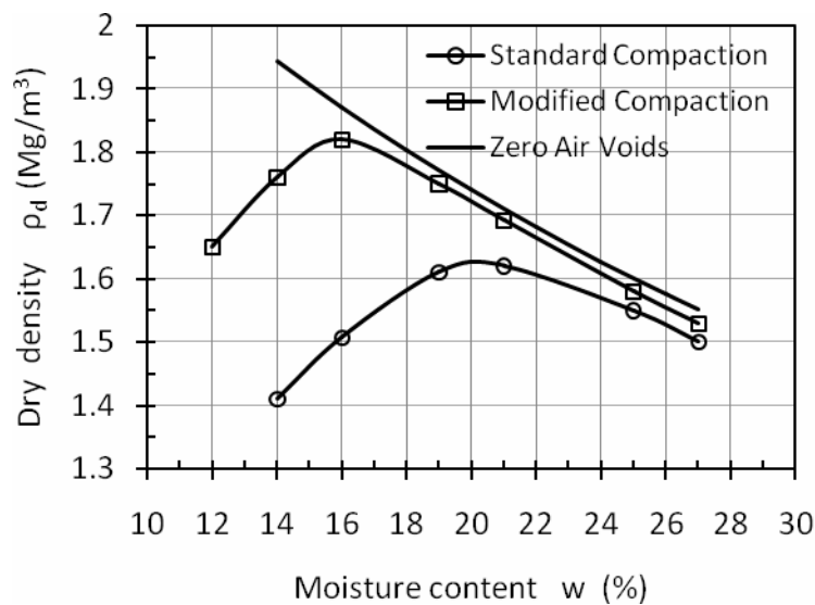
Figure 2: Dry density-moisture content relationship for “JUST” soil
