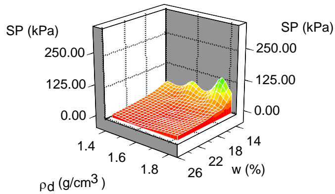
Figure 14: Swell pressure for treated JUST soil, 1% cement content and 28-day curing
