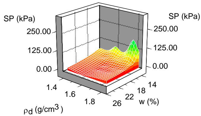
Figure 13: Swell pressure for treated JUST soil, 1% cement content and 7-day curing
