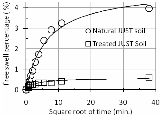
Figure 16: Free swell percentage versus square root of time relationship for JUST soil
