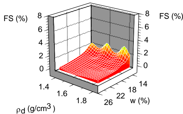
Figure 8: Free swell for treated JUST soil, 1% cement content and 28-day curing
