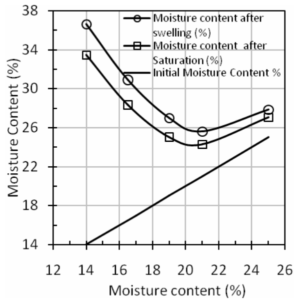
Figure 5: Moisture content at saturation and at the end of swelling for points corresponding to the standard compaction curve of JUST soil, (Al-Sharqi, 1993)
