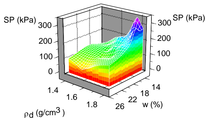
Figure 4: Potential swell pressure of natural JUST soil
