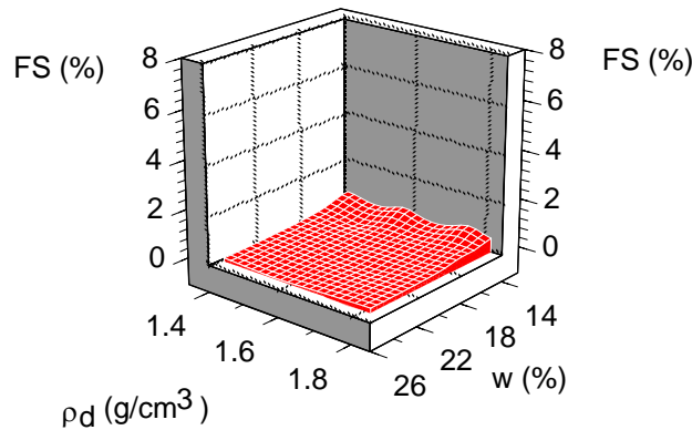
Figure 9: Free swell for treated JUST soil, 2% cement content and 7-day curing
