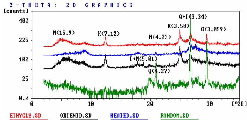
Figure 1: X-ray diffractograms for glycolated, random, heated and air dried JUST soil (K=kaolinite, I=illite, M=montmorillonite, Q=quartz, G=gypsum and ( ) d spacing in Å)
