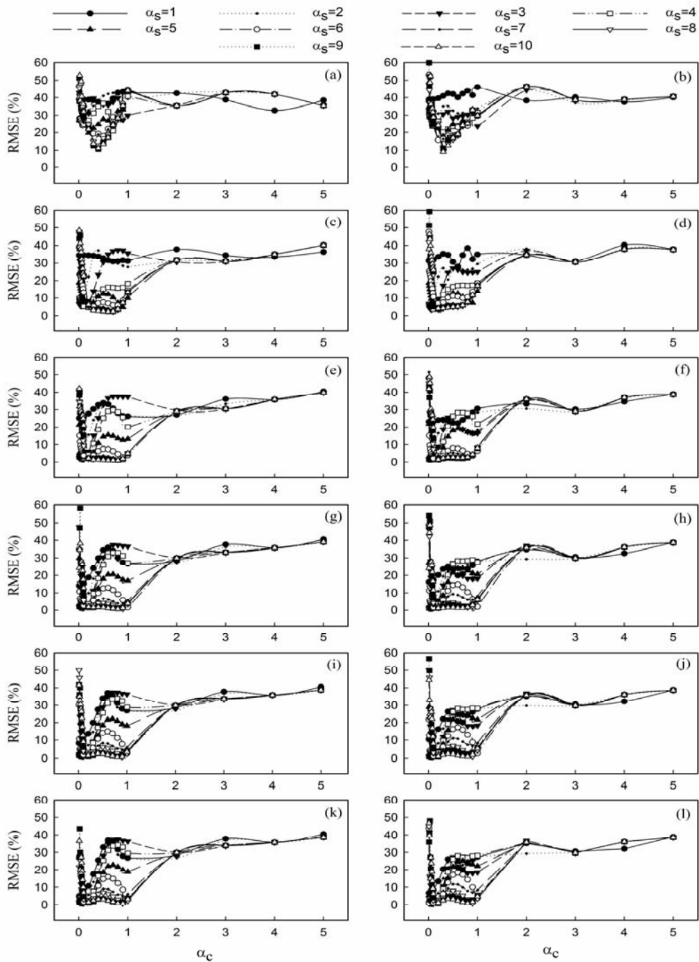
Figure (6): Variation of \alpha_c and \alpha_s relative to the number of nodes. (a) N_{nodes} = 50, S_1 (b) N_{nodes} = 50, S_2 (c) N_{nodes} = 100, S_1 (d) N_{nodes} = 100, S_2 (e) N_{nodes} = 200, S_1 (f) N_{nodes} = 200, S_2 (g) N_{nodes} = 300, S_1 (h) N_{nodes} = 300, S_2 (i) N_{nodes} = 400, S_1 (j) N_{nodes} = 400, S_2 (k) N_{nodes} = 500, S_1 (l) N_{nodes} = 500, S_2
