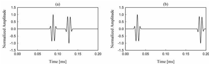
Figure (4): Normalized displacement response of healthy benchmark model captured in (a) S_1 , (b) S_2
