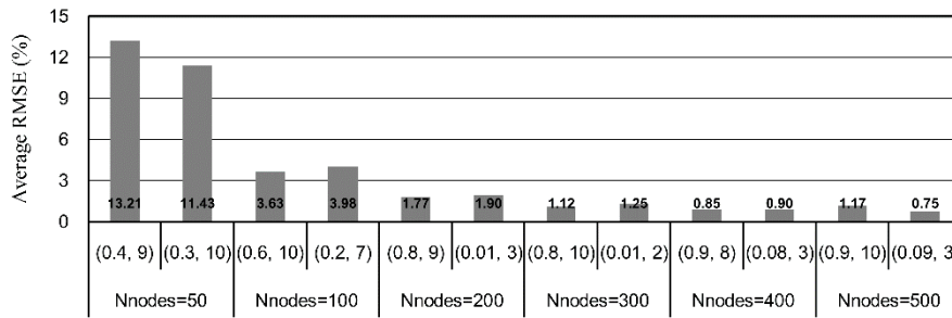
Figure (7): Variation of average RMSE between S_1 and S_2 relative to N_{nodes} and (\alpha_c, \alpha_s)
