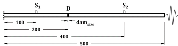
Figure (2): The configuration of the rod as a benchmark model
