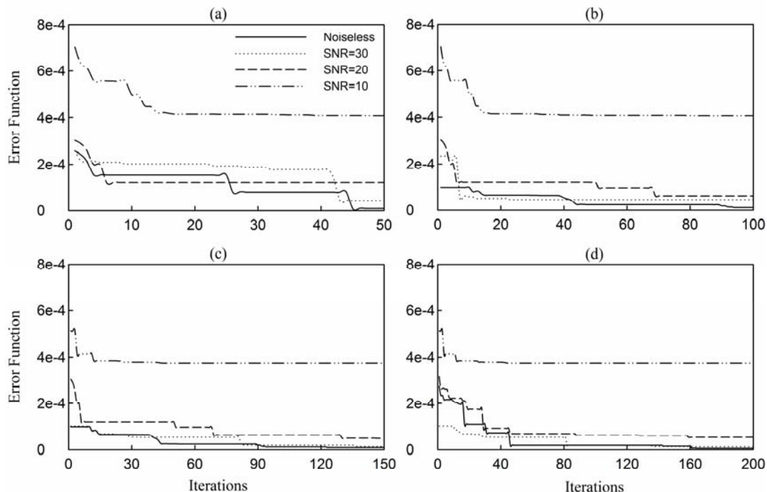
Figure (10): Results of optimization using ICA for number of iterations (a) 50 (b) 100 (c) 150 (d) 200
