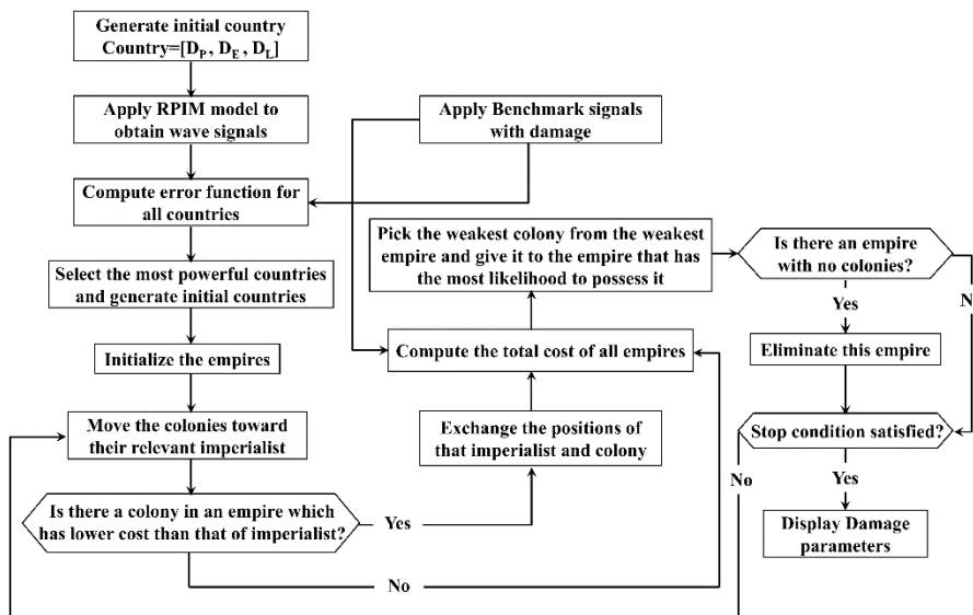
Figure (9): Flowchart of damage identification based on ICA
