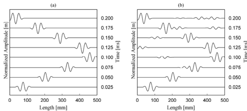
Figure (8): Wave propagation in the length of rod using RPIM (a) healthy state (b) damaged state
