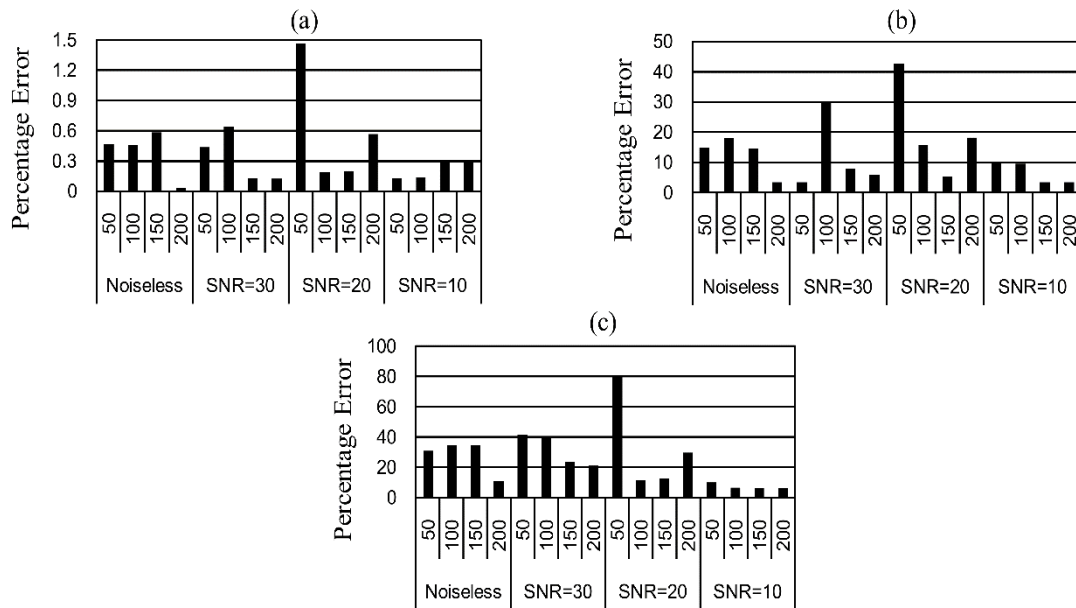
Figure (11): Results of relative errors (a) position (b) extent (c) length
