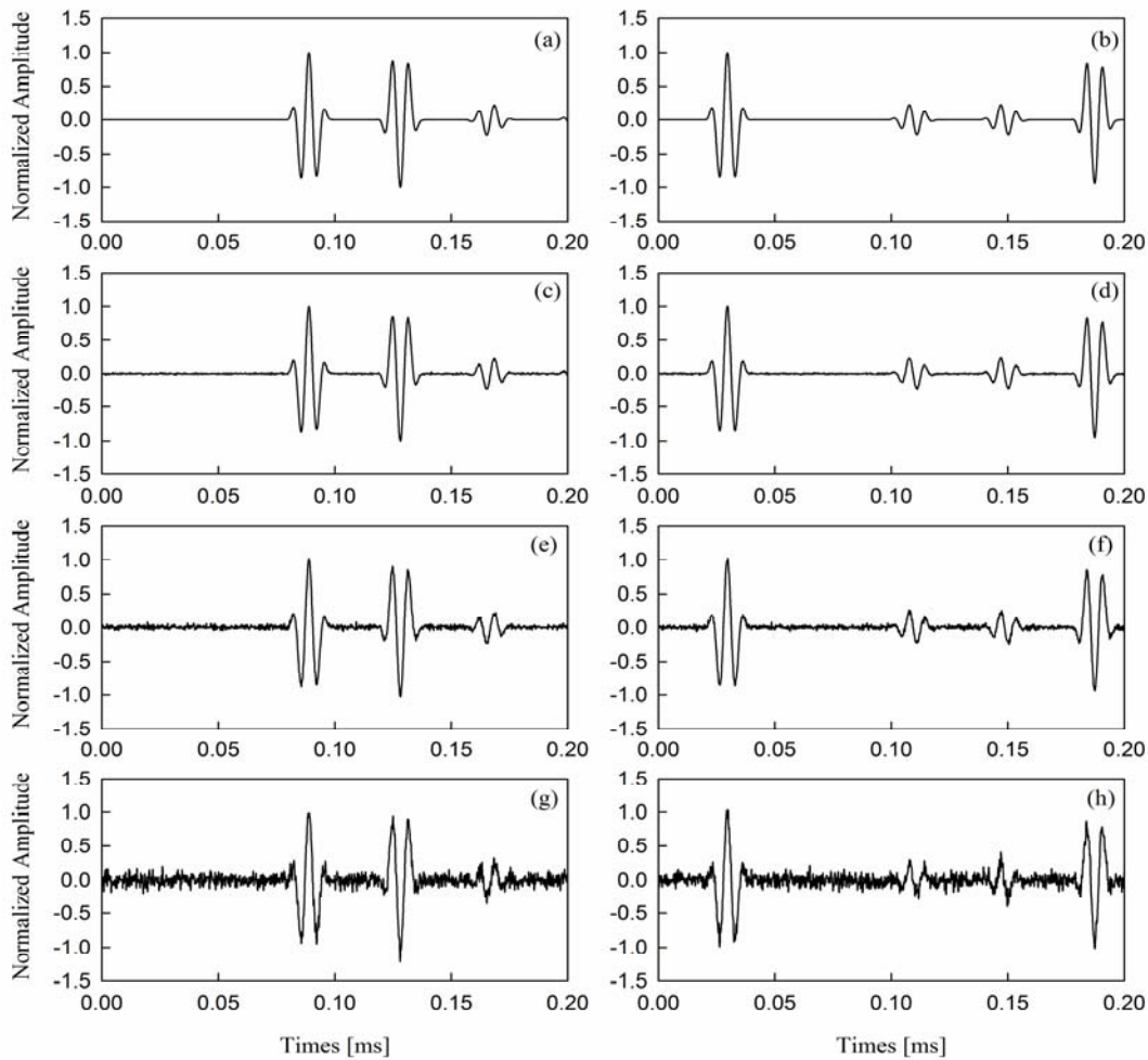
Figure (5): Normalized displacement response of damaged benchmark model captured in: (a) S_1 , noiseless (b) S_2 , noiseless (c) S_1 , SNR=30 (d) S_2 , SNR=30 (e) S_1 , SNR=20 (f) S_2 , SNR=20 (g) S_1 , SNR=10 (h) S_2 , SNR=10
