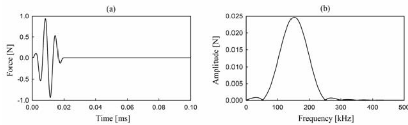
Figure (3): Form of an excitation signal in: (a) time domain, (b) frequency domain
