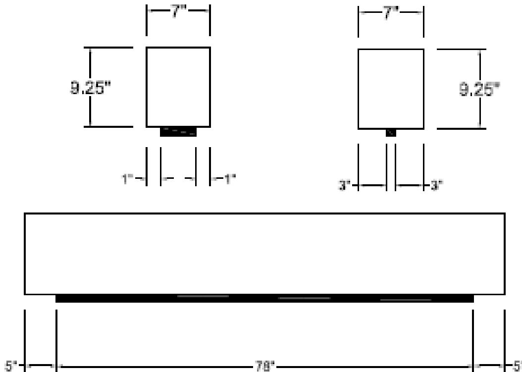
Figure (2): FRP Position with Respect to Beam Dimensions
