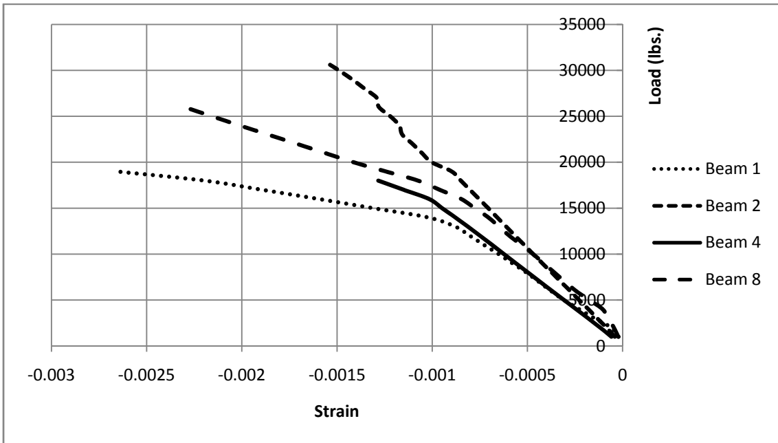
Figure (5):The Strain in Concrete at Mid-span for Typical Beams
