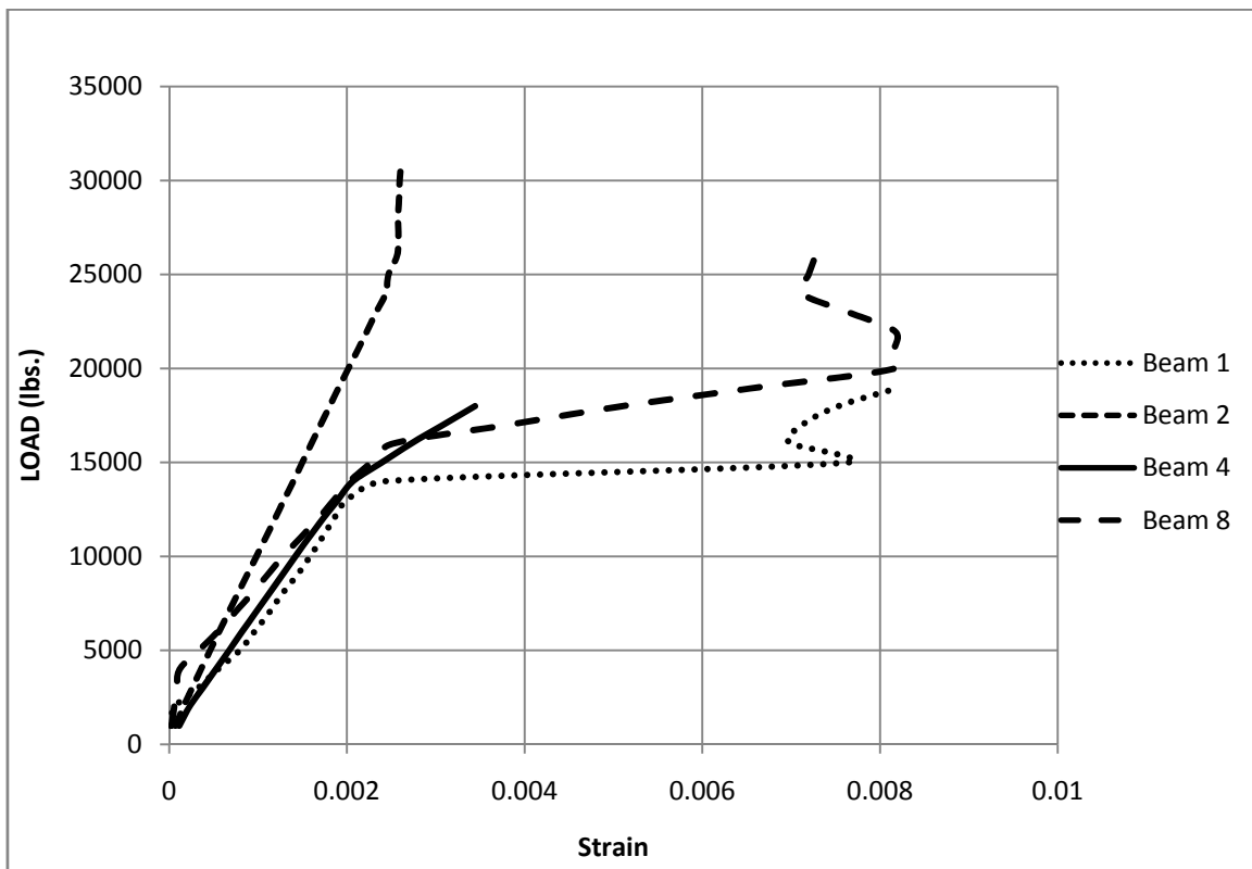
Figure (6):The Strain in Steel Bars at Mid-span for Typical Beams
