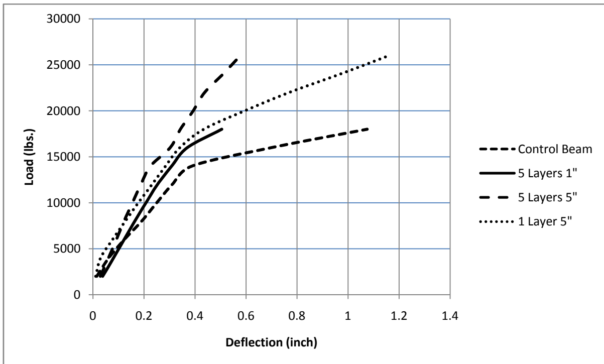
Figure (4): The Deflection at Mid-span for Typical Beams
