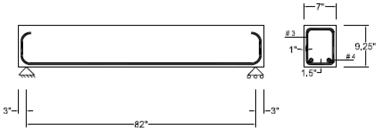
Figure (1): Longitudinal Section and Cross-section of R.C. Test Beam
