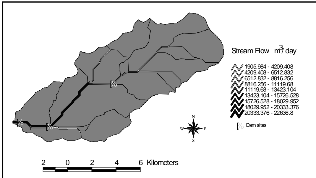
Figure 6: Flow Result in the Stream as m 3 /day.
