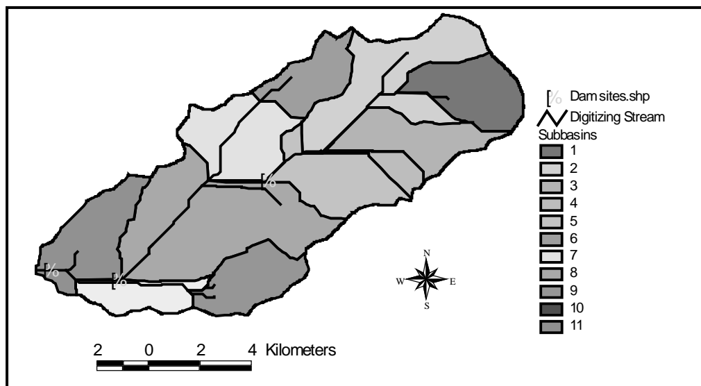
Figure 4: Subbasins' Map of Kufranja Watershed.
