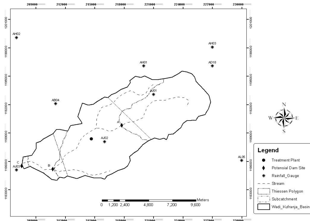
Figure 1: Kufranja Basin.
