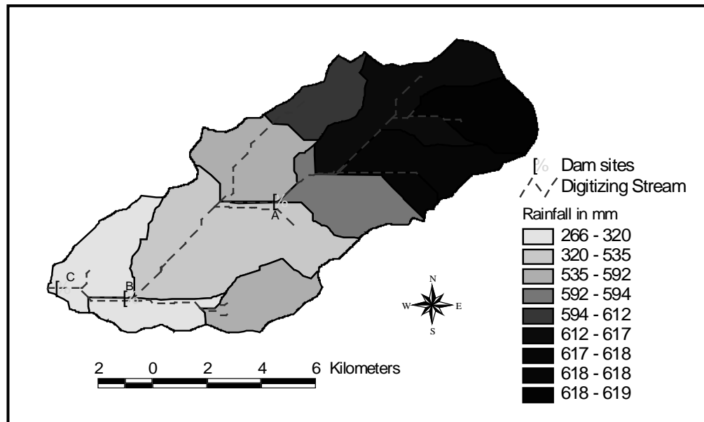
Figure 5: Spatial Distribution of Annual Rainfall Distribution.
