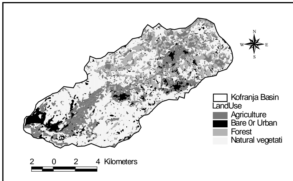
Figure 3: Land Use Map of Kufranja Watershed.
