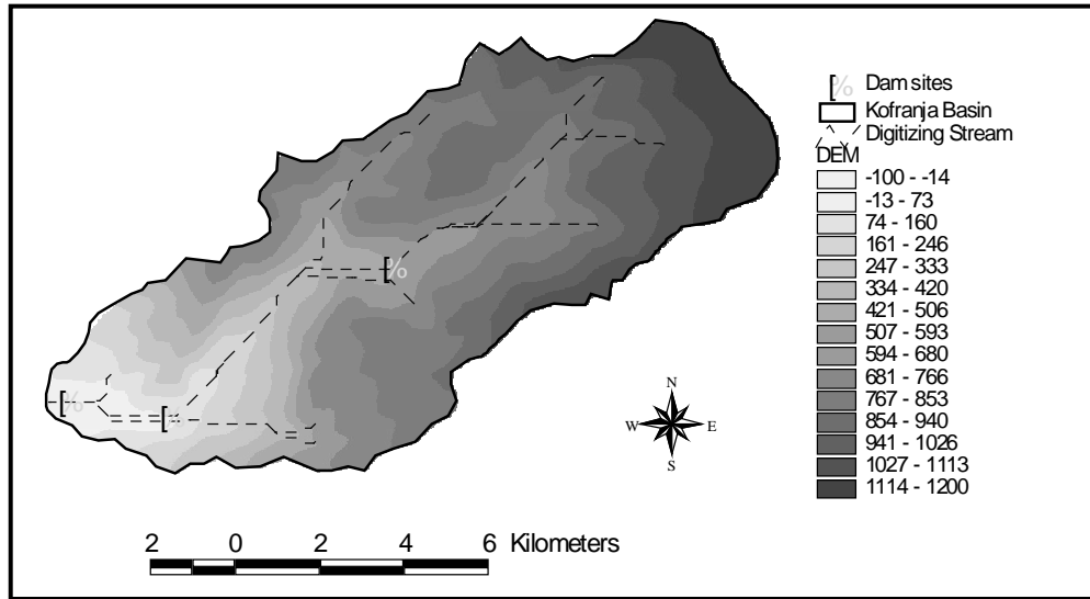
Figure 2: Digital Elevation Map (DEM) of Kufranja Watershed.
