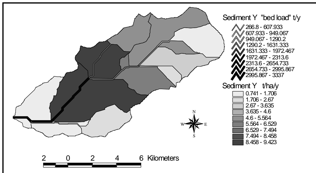
Figure 7: Sediment Yield Result.
