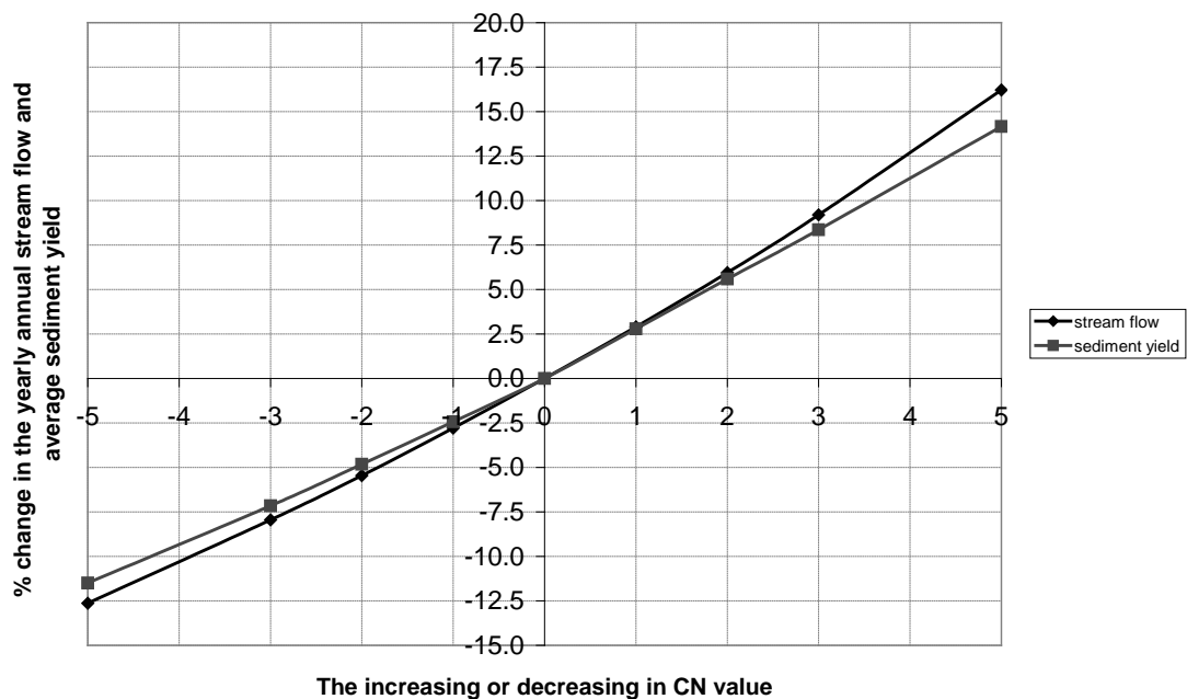
Figure 9: CN Parameter Effect on Streamflow and Sediment Yield.
