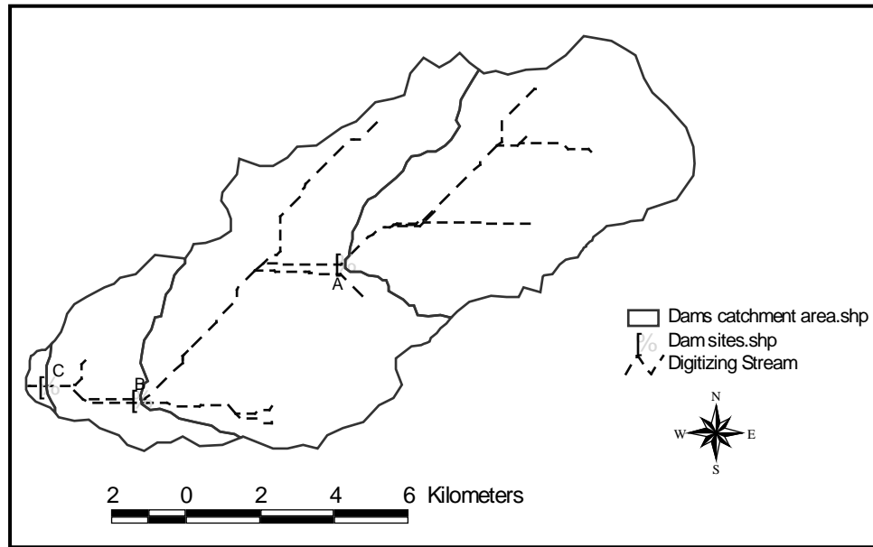
Figure 8: Dams Catchment Area.
