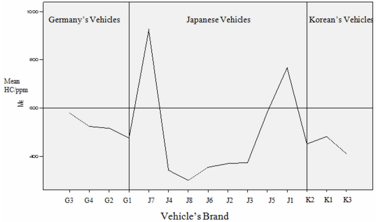
Figure 7: Average HC emission levels with reference to Jordanian standards
