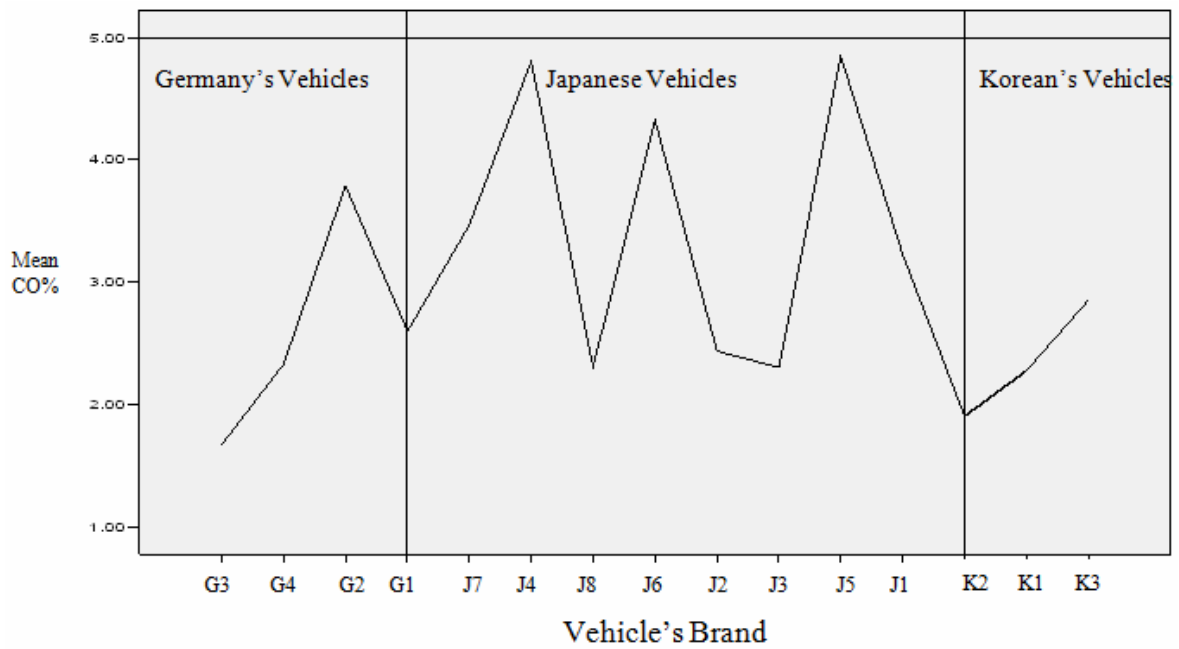
Figure 8: Average CO emission levels with reference to Jordanian standards
