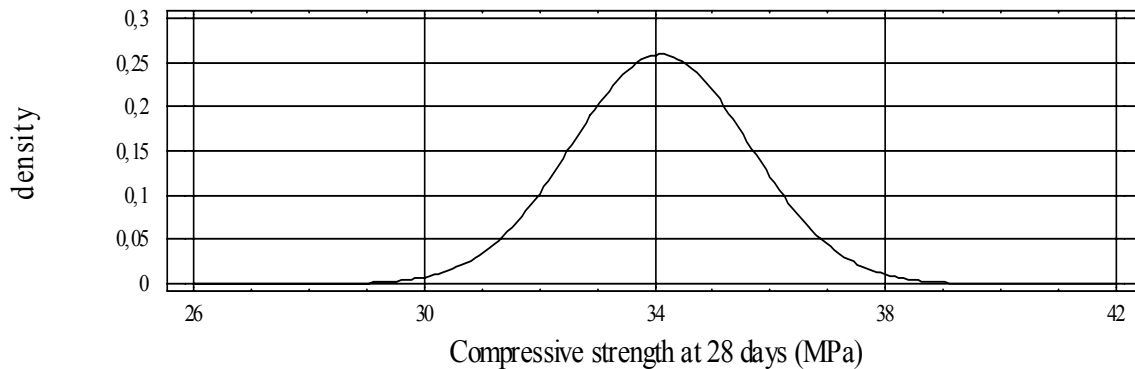
Figure (6): Distribution of strengths at 28 days according to the normal law (Djebel Abiod).
