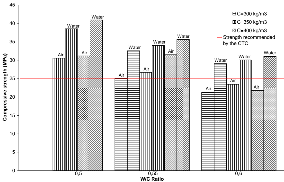
Figure (8): Concrete strengths at 28 days preserved in water and air for various water/cement ratios (Aggregates of Dhar El Mendjel).
