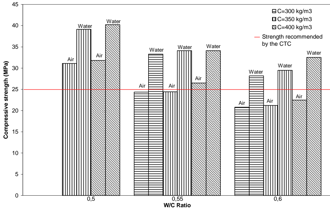
Figure (7): Concrete strengths at 28 days preserved in water and air for various water/cement ratios (Aggregates of Djebel Abiod).
