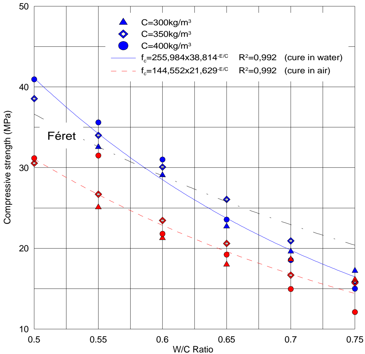
Figure (10): Relation between the compressive strength at 28 days and the water/cement ratio (Dhar El Mendjel).
