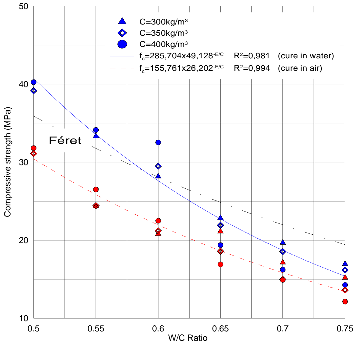
Figure (9): Relation between the compressive strength at 28 days and the water/cement ratio (Djebel Abiod).
