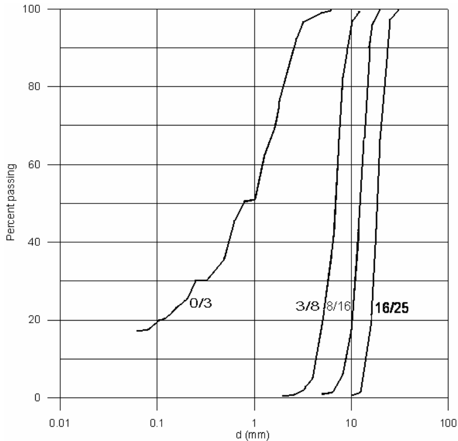
Figure (1): Grading curves of the aggregates of Djebel Abiod.
