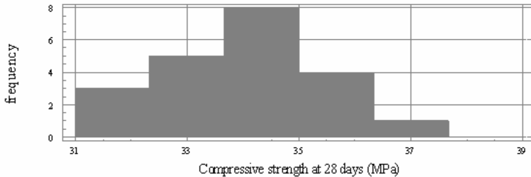
Figure (5): Histogram of distribution of strengths at 28 days (Djebel Abiod).
