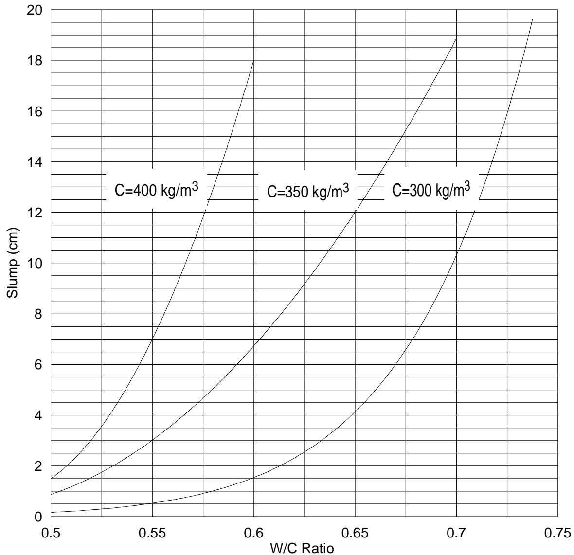
Figure (11): Abacus allowing to evaluate roughly the cement proportioning to be envisaged according to W/C ratio and of desired workability (slump in Abrams cone).
