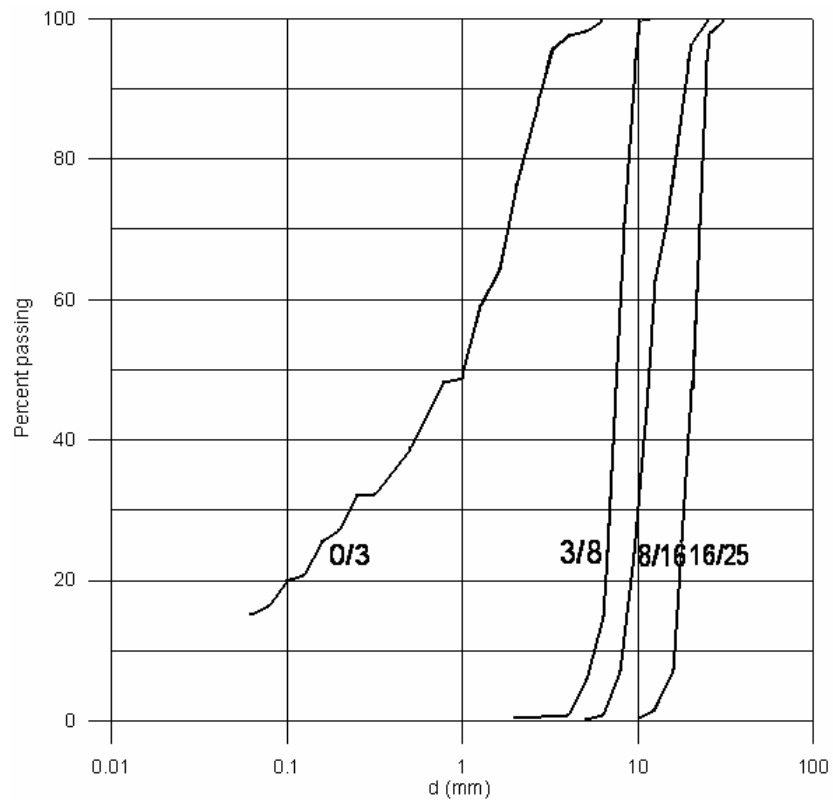
Figure (2): Grading curves of the aggregates of Dhar El Mendjel.
