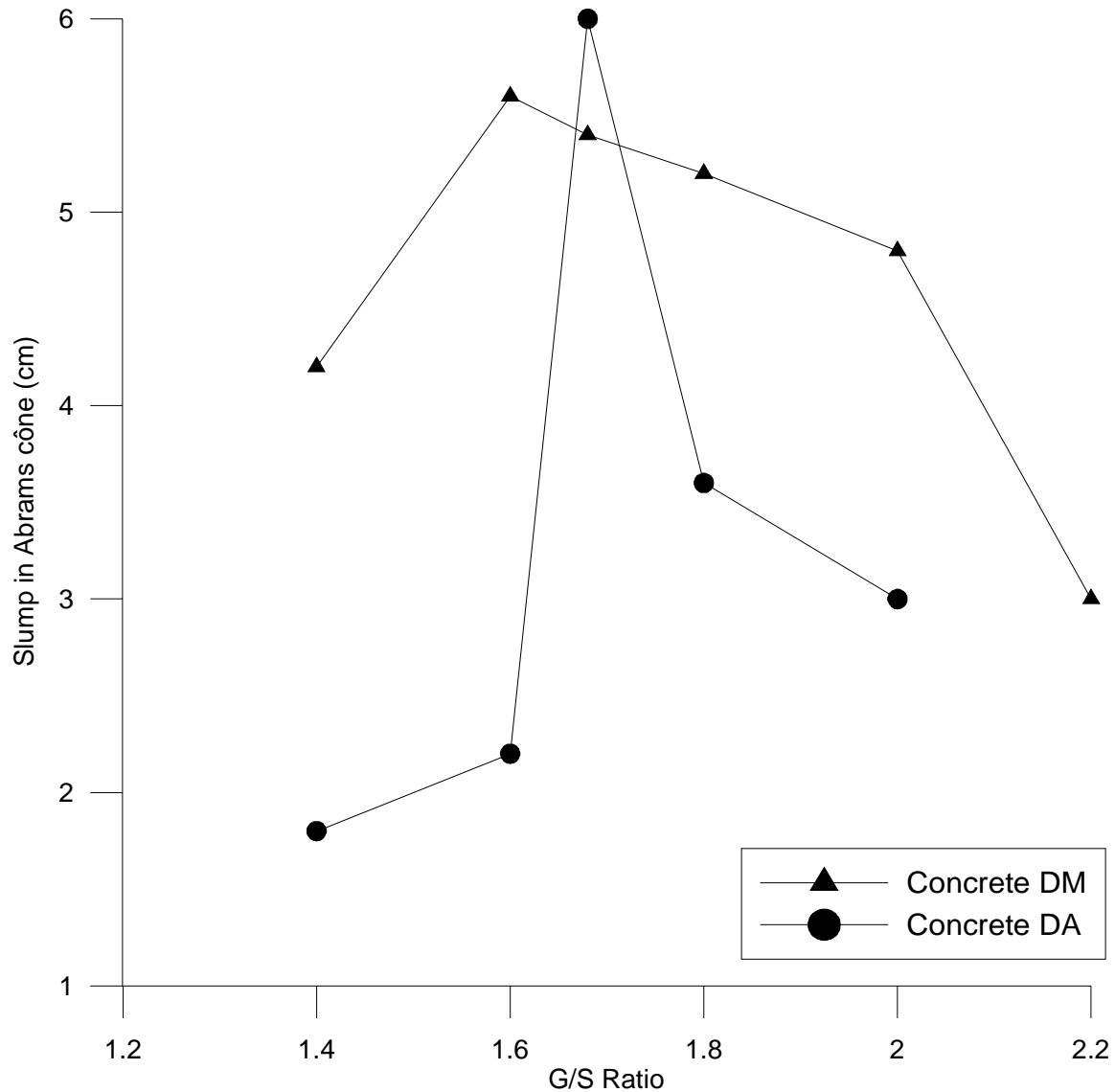
Figure (4): Optimization of ratio G/S according to slump.
