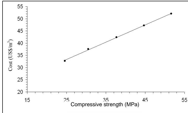
Figure (8): Cost of m 3 of concrete as function of strength.
