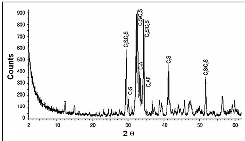
Figure (1): X-rays diffraction of anhydrous cement CEM I.
