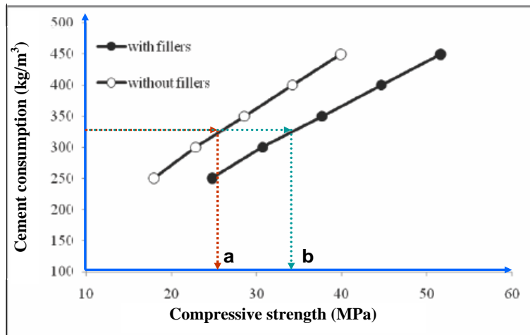
Figure (7): Cement consumption and strength.
