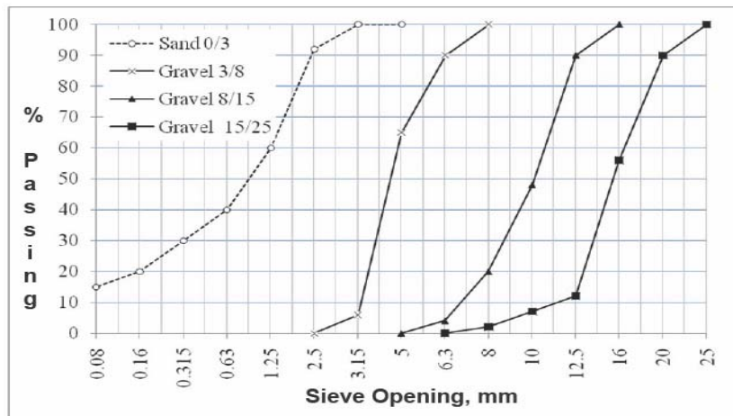
Figure (2): Aggregates gradation.
