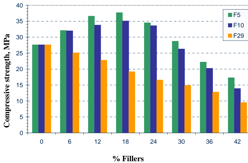
Figure (4): Influence of filler concentration on 28-day compressive strengths.
