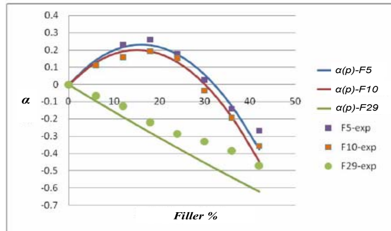
Figure (5): Evolution of \alpha(p) versus percentage of fine.
