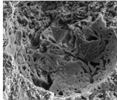
6.4: Formation of pores at 28 days (M40-F29).
