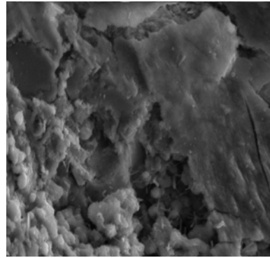
6.2: Formation of CSH in concrete M18-F5 in 28 days.
