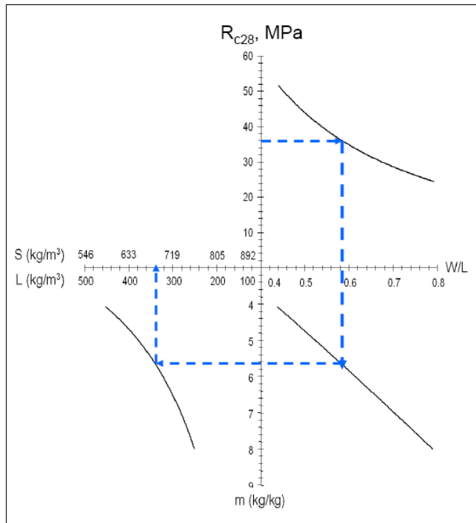
Figure (9): Mix proportioning diagram.
