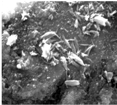
6.1: Formation of the carboaluminates crystals in concrete M18-F5 at 7 days.
