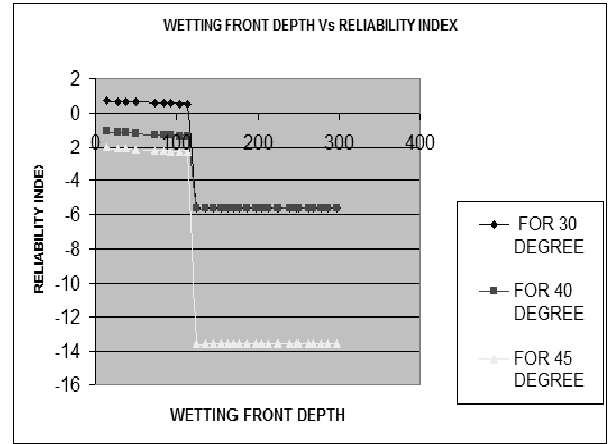
Figure (9): Variation of reliability index with wetting front depth
