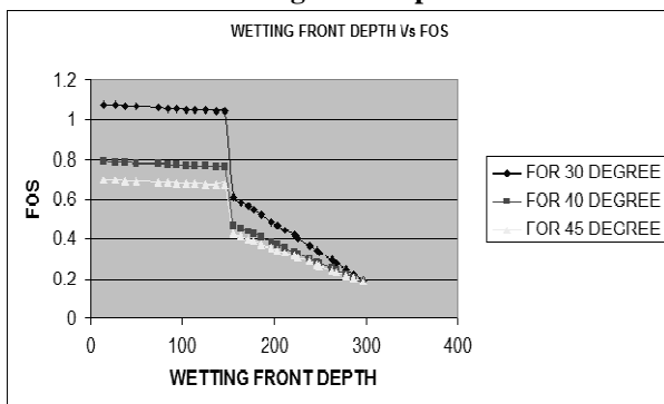
Figure (4): Variation of factor of safety with wetting front depth for steep and flat slopes
