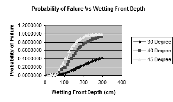
Figure (7): Variation of failure probability with wetting front depth
