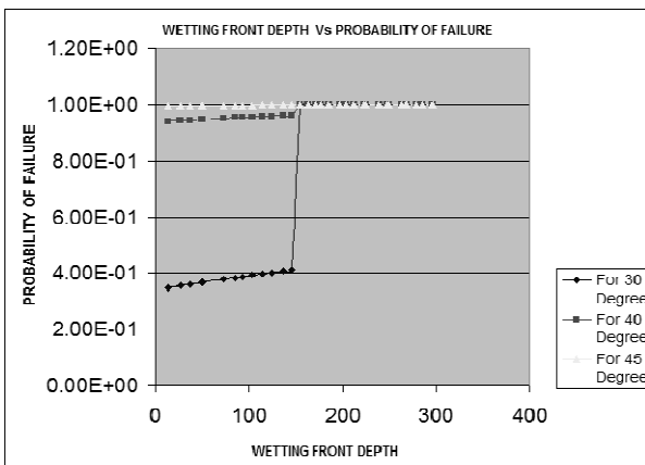
Figure (8): Variation of failure probability with wetting front depth
