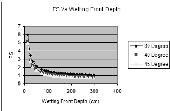
Figure (3): Variation of factor of safety with wetting front depth
