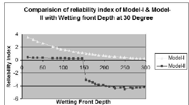
Figure (10): Variation of reliability index with wetting front depth for model-I and model-II
