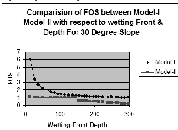
Figure (5): Variation of FOS with wetting front depth for model-I and Model-II
