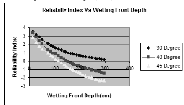
Figure (6): Variation of reliability index with wetting front depth
