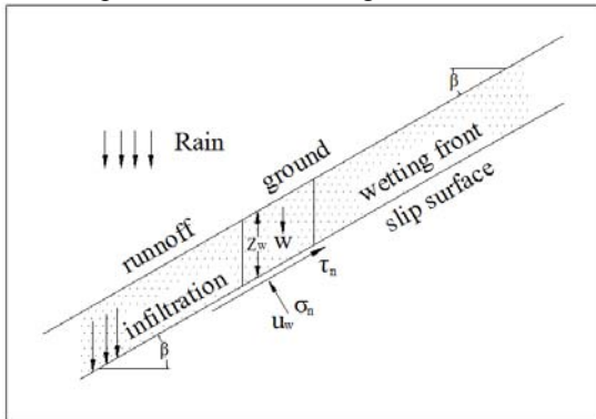
Figure (1): The ‘infinite slope’ model used in the study for Model-I
