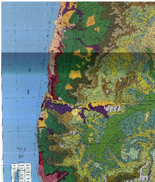
Figure 3: Geological Map (1:50000).
