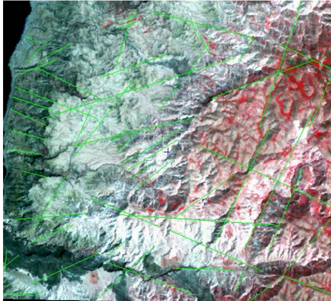
Figure (7): Image map showing faults that already existed in the published geological map.
