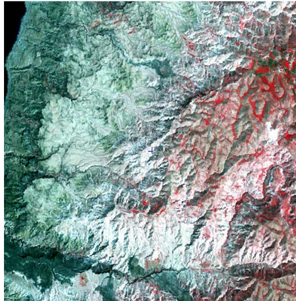
Figure (5): Sharping Edge Filter (FLSZ=7, 7).
