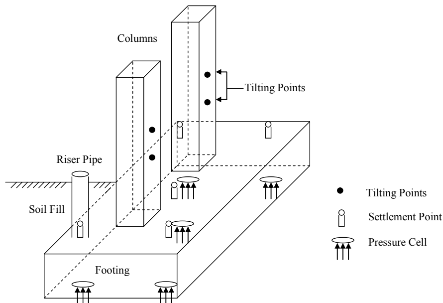
Figure 1: Overall Field Instrumentation Scheme for Spread Footing
