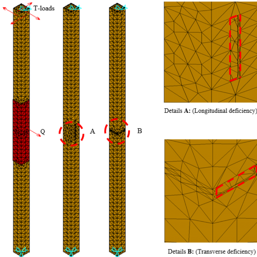
Figure (2): A view of finite element modeling of strengthened and non-strengthened specimens having deficiency in ANSYS
