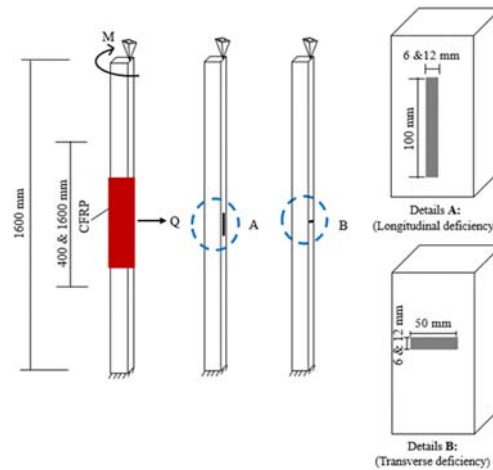
Figure (1): A schematic view (not to scale) of strengthened and non-strengthened SHS steel members having deficiency
