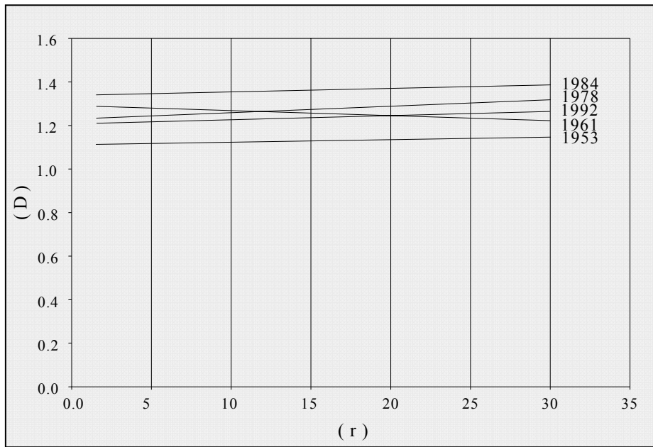
Figure 5: The direct graphical relationship between (D) and (r)
