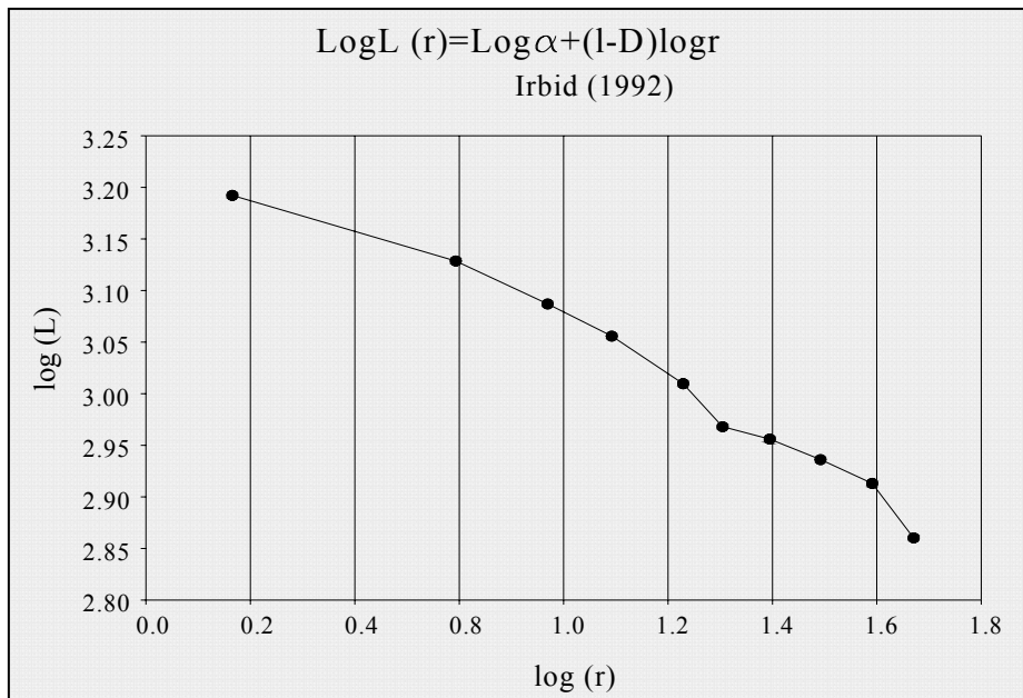
Figure 3: Logarithmic graph between log (L) and log (r), Irbid 1992
