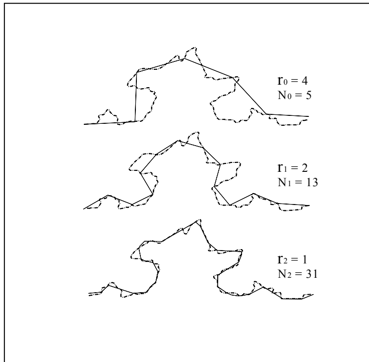
Figure 1: Approximating an irregular line and measuring perimeter length at three scales (Batty and Longley, 1994)
