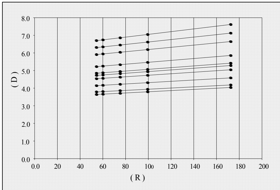
Figure 6: The direct graphical relationship between (D) and (R)
