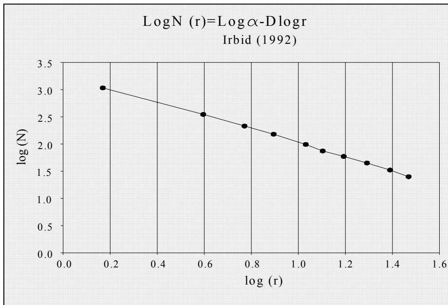
Figure 4: Logarithmic graph between log (N) and log (r), Irbid 1992
