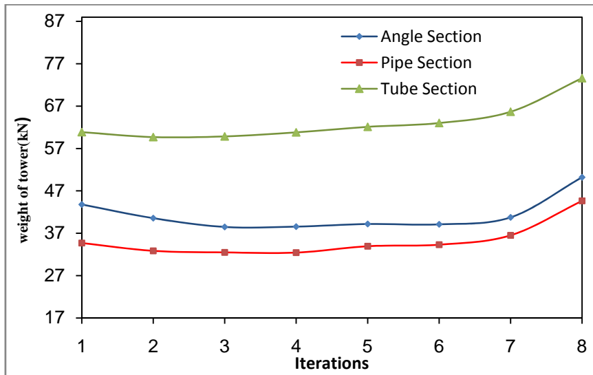
Figure 14: Comparison between Angle, Pipe and Tube Sections with X -Bracing under Anti-Cascade Loading Condition for 1S2 Tower
