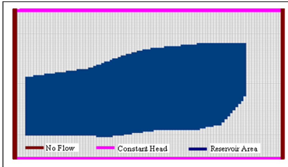
Figure 12: Boundary conditions
