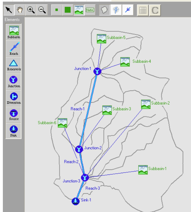
Figure 7: Wadi Bayer basin model schematic
