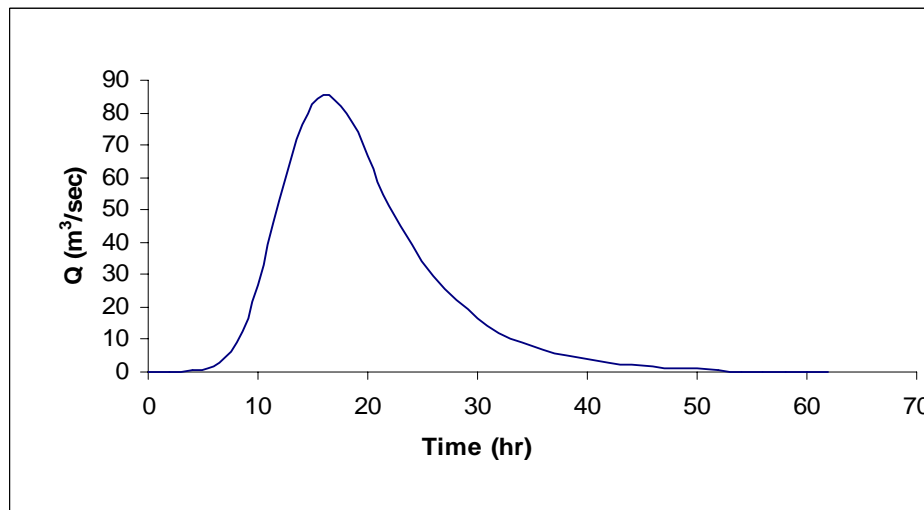
Figure 6: 50-year hydrograph
