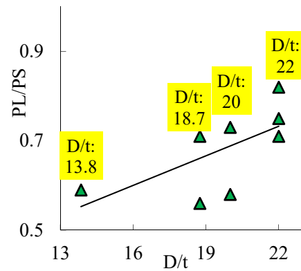
Figure (11): Effect of D/t ratio on P_L/P_S
