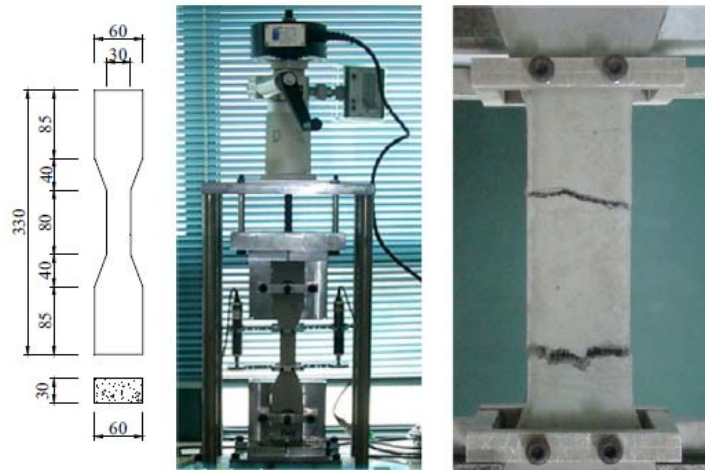
Figure (9): Details of dumbbell specimen studied in lab environment
