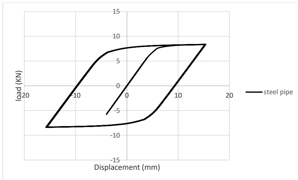
Figure (15): Hysteresis graph for pipe damper
