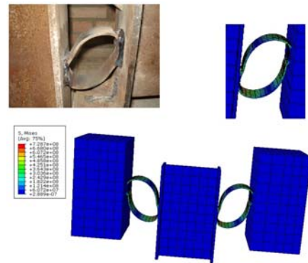
Figure (6): Compliance of lab specimen with finite element specimen
