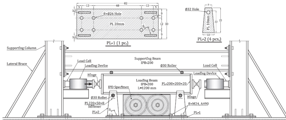
Figure (2): Test set-up for pipe dampers
