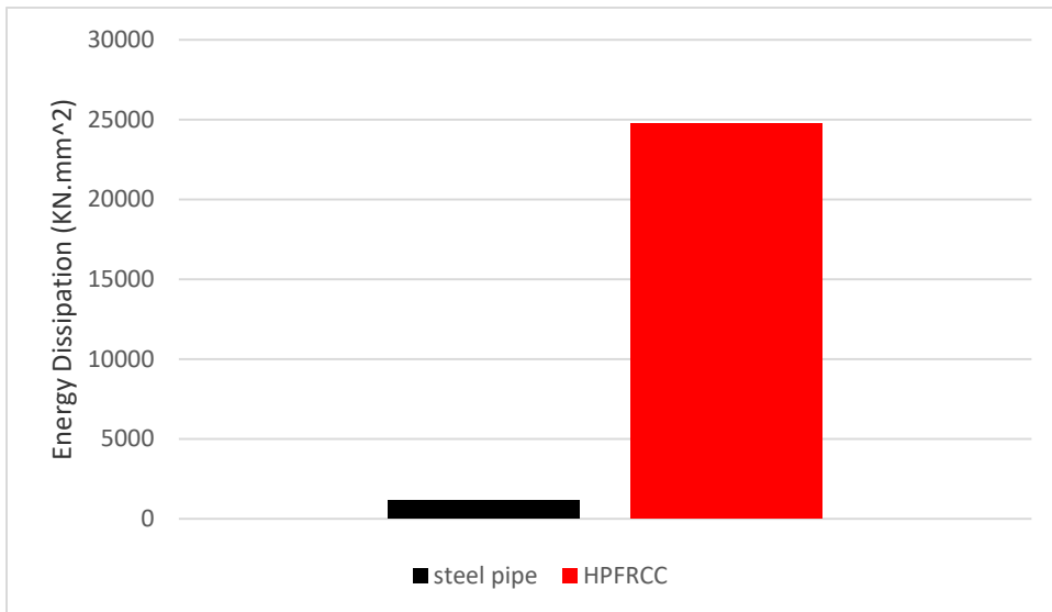
Figure (17): Comparison of depreciated energy for pipe damper and for pipe damper reinforced with HPFRCC
