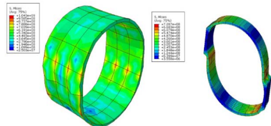
Figure (14): Von Mises tension in pipe damper (right) and pipe damper with base composite matter (left)
