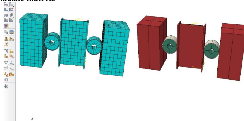
Figure (12): Schematic model of reinforced pipe element with HPFRCC and meshing of the set
