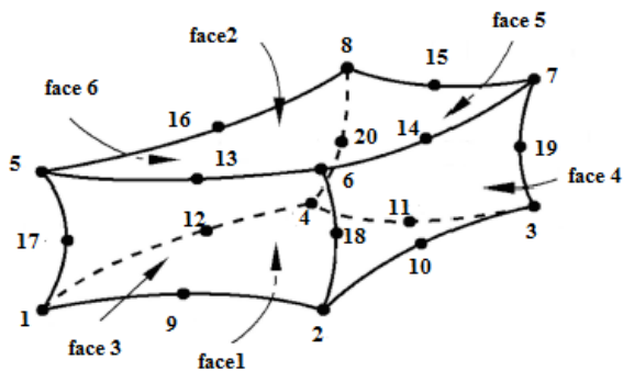
Figure (11): 20-node element utilized to simulate concrete
