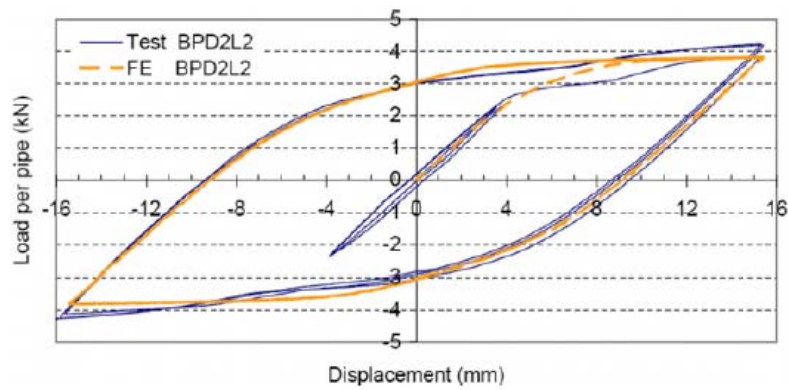
Figure (7): Simulation graph and lab specimen match
