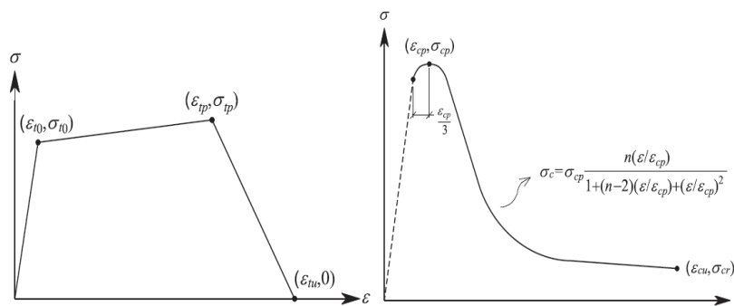
Figure (8): Tensile (a) and Compressive (b) fiber behaviour of concrete
