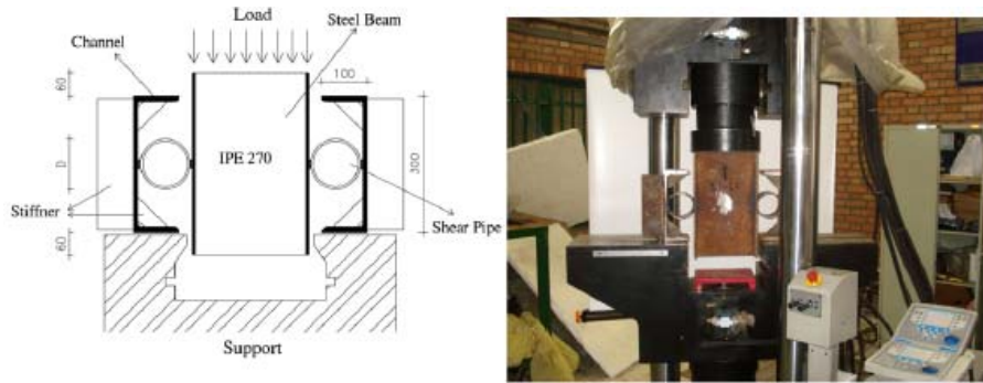
Figure (5): Details of lab-tested specimen
