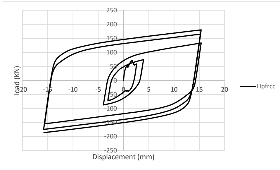
Figure (16): Hysteresis graph for pipe damper reinforced with HPFRCC
