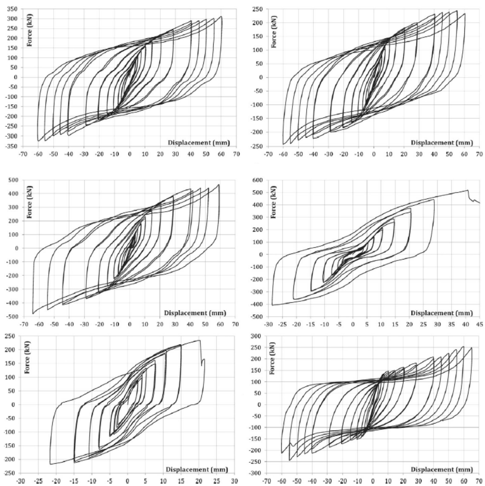
Figure (4): Hysteresis graphs for reinforced pipe dampers
