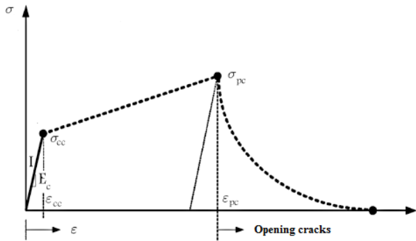
Figure (1): Relation between strain and stress in (HPFRCCs) under tensile force
