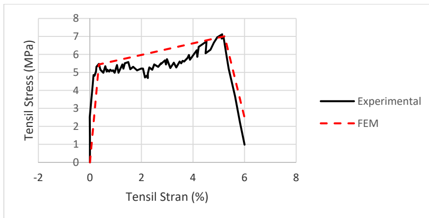
Figure (10): Compliance of lab sample and simulated specimen in software environment
