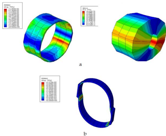
Figure (13): Index of damage a) reinforced specimen with HPFRCC b) simple specimen pipe
