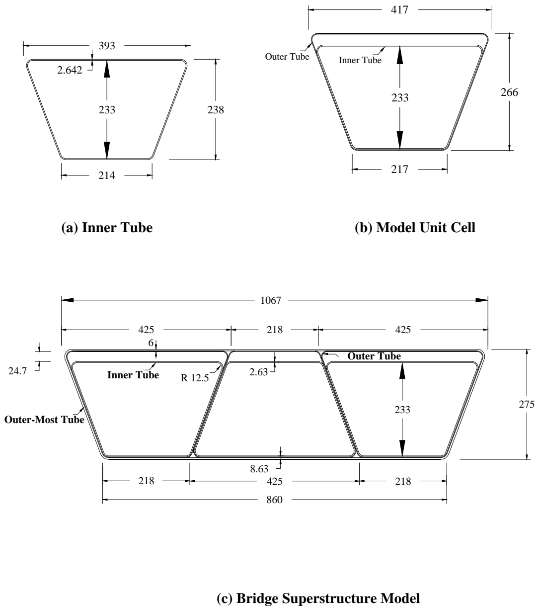
Figure (1): Cross-Section of the Hybrid FRP-Concrete Superstructure Model (Units in mm).
