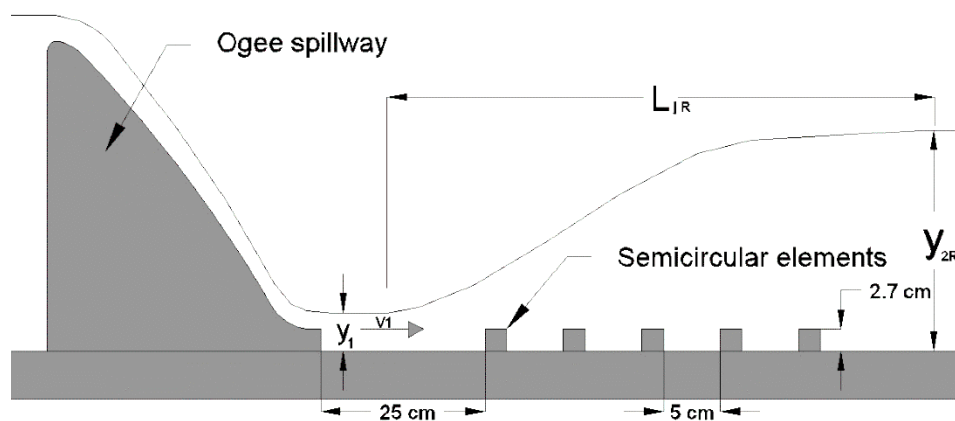
Figure (1): Longitudinal section in the region of hydraulic jump over semicircular roughness elements
