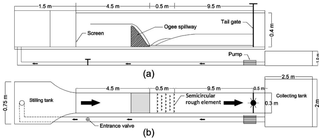
Figure (2): Experimental flume (a) longitudinal section view and (b) plan view
