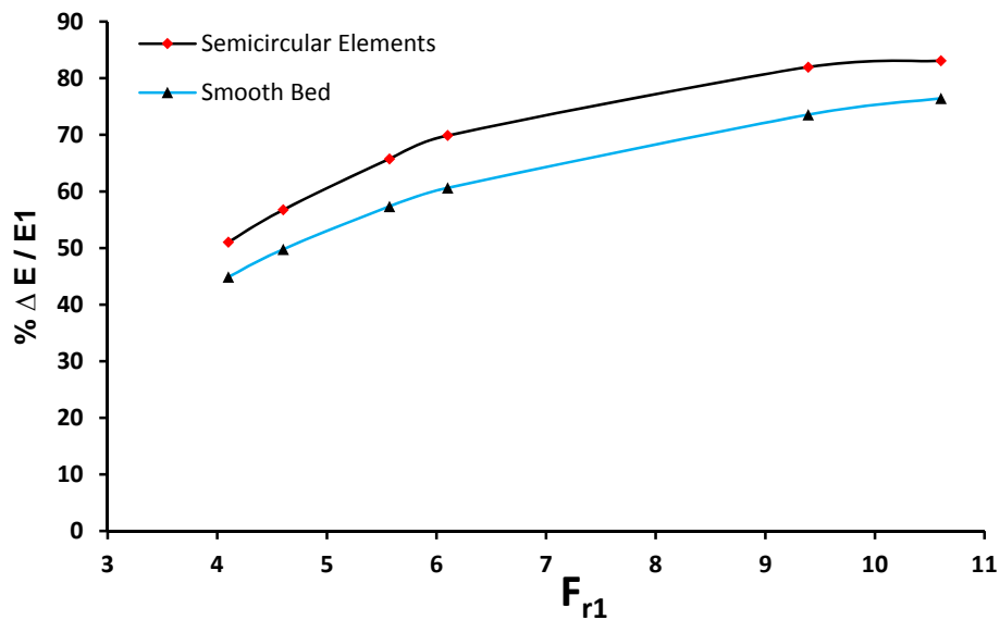
Figure (7): Variation of energy dissipation with flow rate
