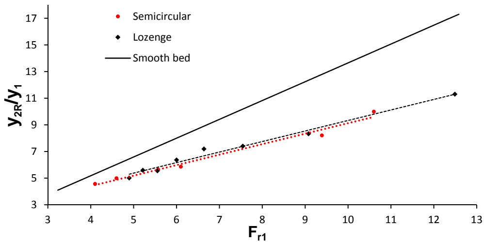
Figure (4): Sequent depth ratio versus Froude number
