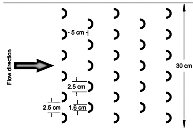
Figure (3): Arrangement of semicircular elements in this study
