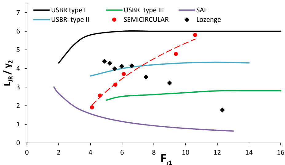
Figure (6): Length of semicircular rough element stilling basin compared to USBR, SAF and Lozenge stilling basins
