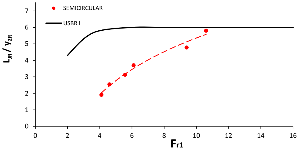
Figure (5): Stilling basin length versus Froude number
