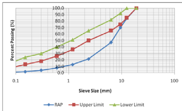
Figure (2): Particle Size Distribution Curve for RAP
