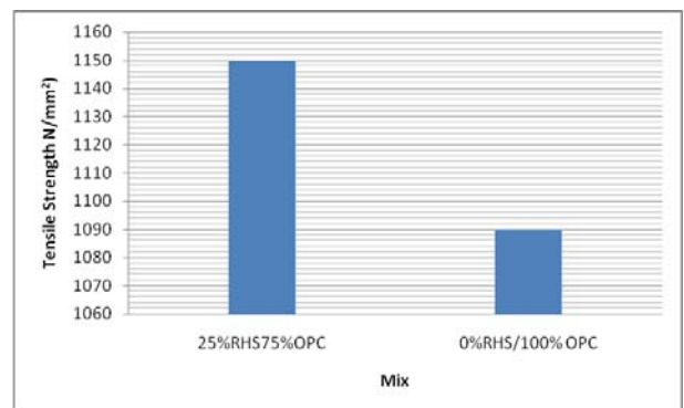
Figure (10): Indirect Tensile Strength Test Results
