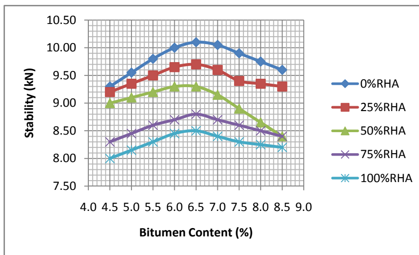
Figure (4): Stability against Binder Content
