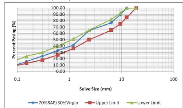
Figure (3): Particle Size Distribution Curve for RAP/Fresh Aggregate Blend
