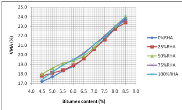
Figure (8): VMA against Binder Content
