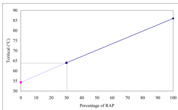
Figure (1): High Temperature Blending Chart (Imad et al., 2009)
