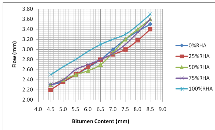
Figure (5): Flow against Binder Content
