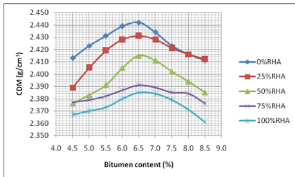
Figure (6): CDM against Binder Content
