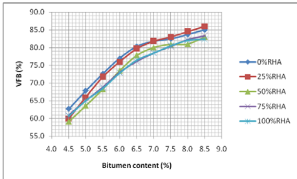
Figure (9): VFB against Binder Content
