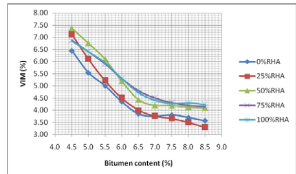
Figure (7): VIM against Binder Content
