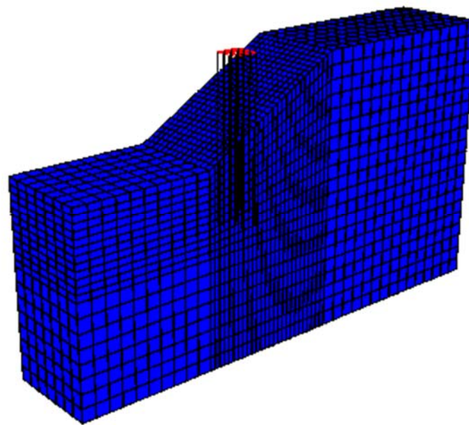
Figure (1): Model slope and finite difference mesh
