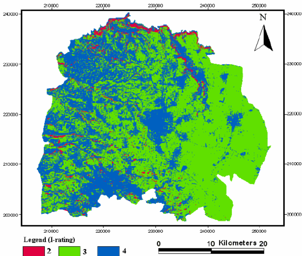
Figure (4): The rating distribution of the infiltration parameter in the study area.
