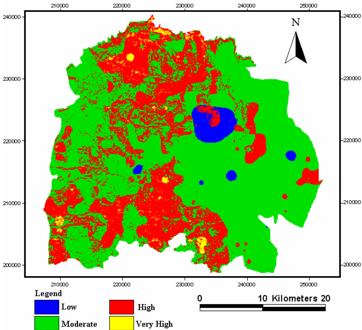
Figure (5): Groundwater vulnerability map of the study area using EPIK method.
