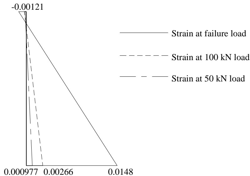
Figure 4: Strain distribution for the control beam
