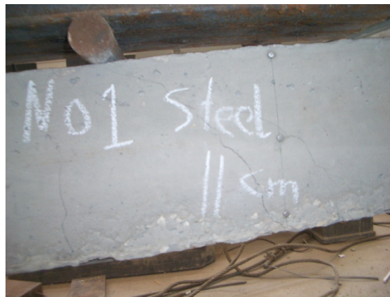
Figure 9: Failure mode of beam retrofitted with NSS plates
