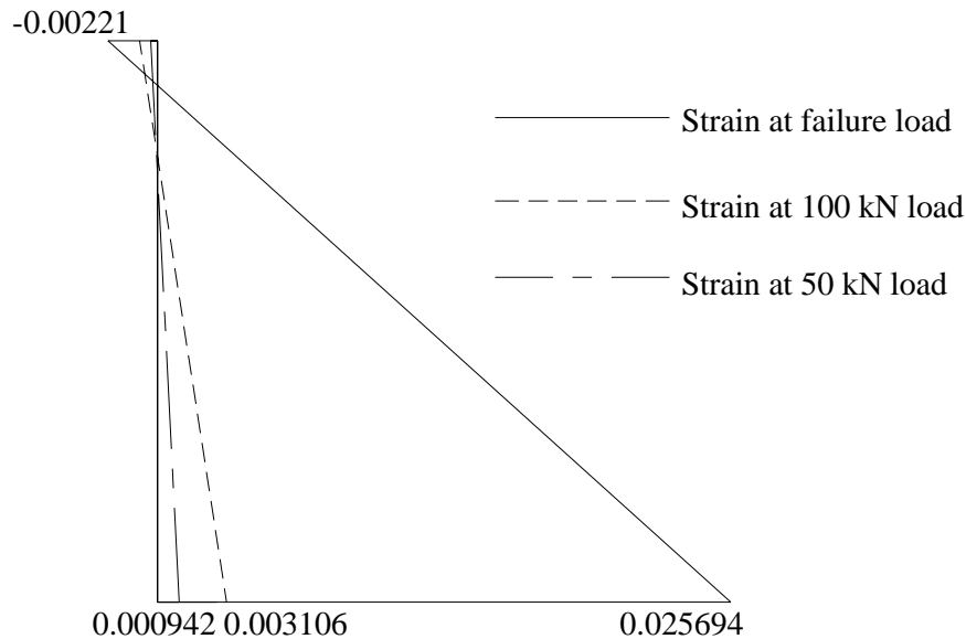
Figure 8: Strain distribution for beam retrofitted with HSGS plates
