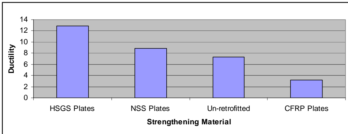
Figure 11: Ductility value of each strengthening material
