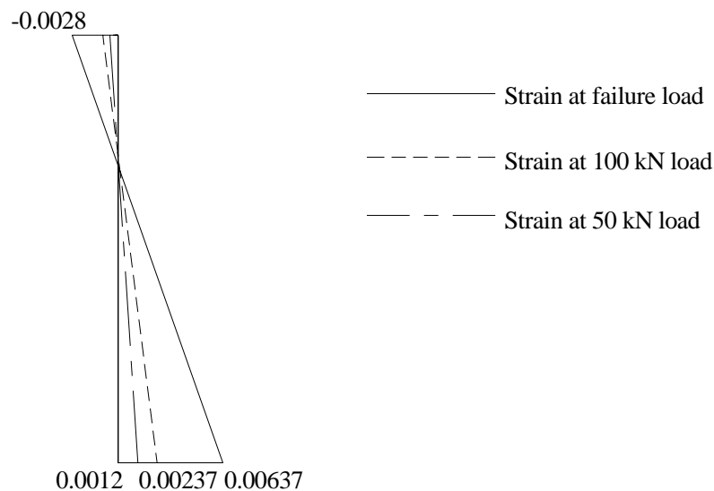
Figure 6: Strain distribution for beam retrofitted with CFRP plates
