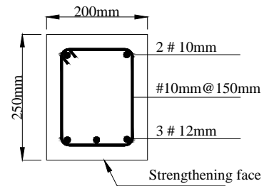
Figure 1: Details of test specimens
