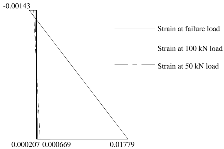
Figure 10: Strain distribution for beam retrofitted with NSS plates
