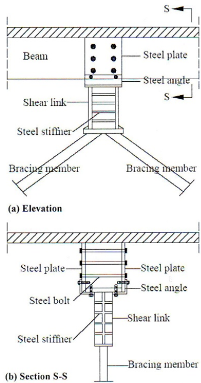
Figure 5: Connection details of the vertical steel link
