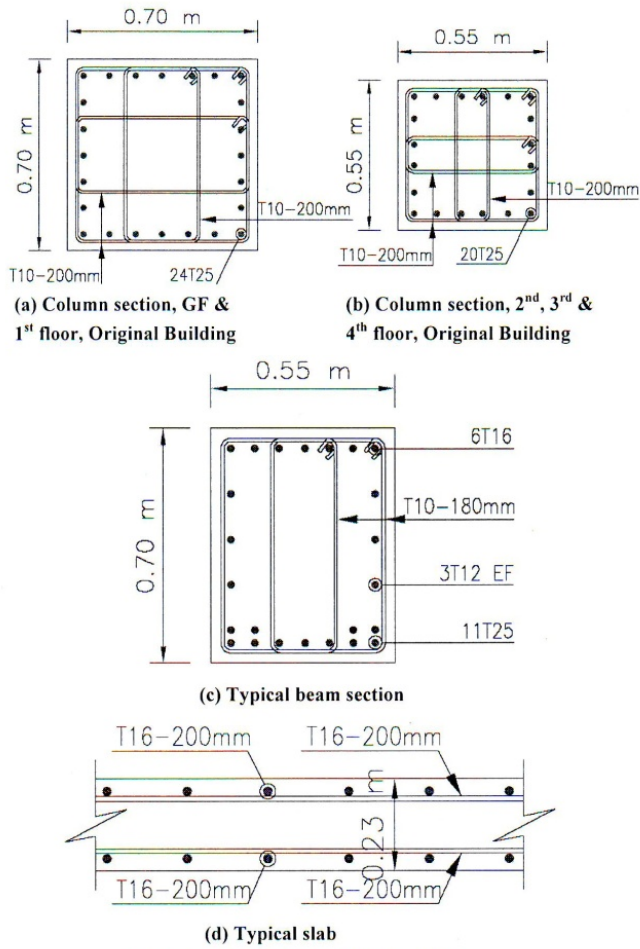
Figure 3: Original building sections details
