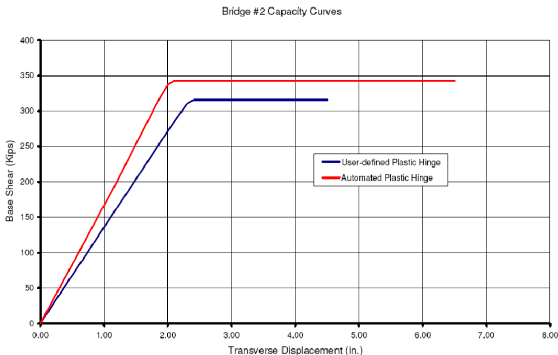
Figure 6: Transverse Pushover Curves for Bridge #2
