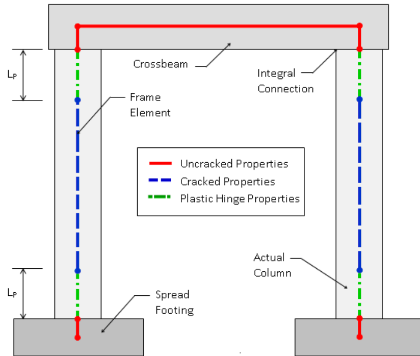
Figure 3: Locations of Section Properties in a Typical Pier (LP: Equivalent Plastic Hinge Length)
