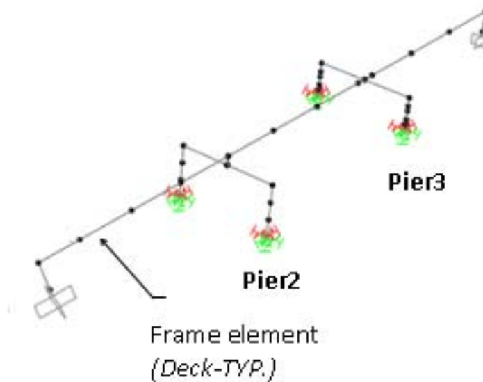
Figure 2: Three-dimensional Model of the Bridge
