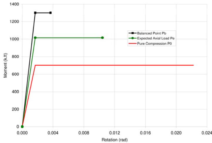
Figure 1: Typical Moment-Rotation Relationship for a Plastic Hinge at Different Axial Load Levels
