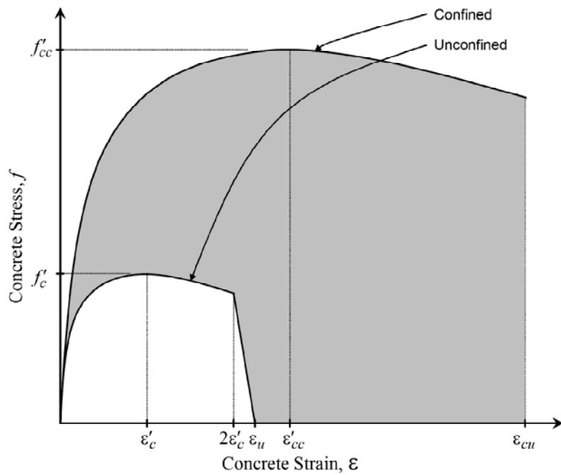
Figure 4: Mander Confined and Unconfined Stress-Strain Curves (Mander et al., 1988)
