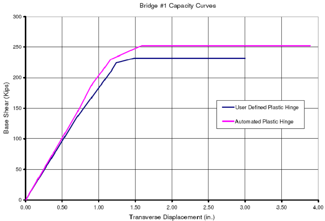
Figure 5: Transverse Pushover Curves for Bridge #1
