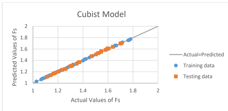
Figure (2): Actual vs. predicted values of training and testing data using cubist model
