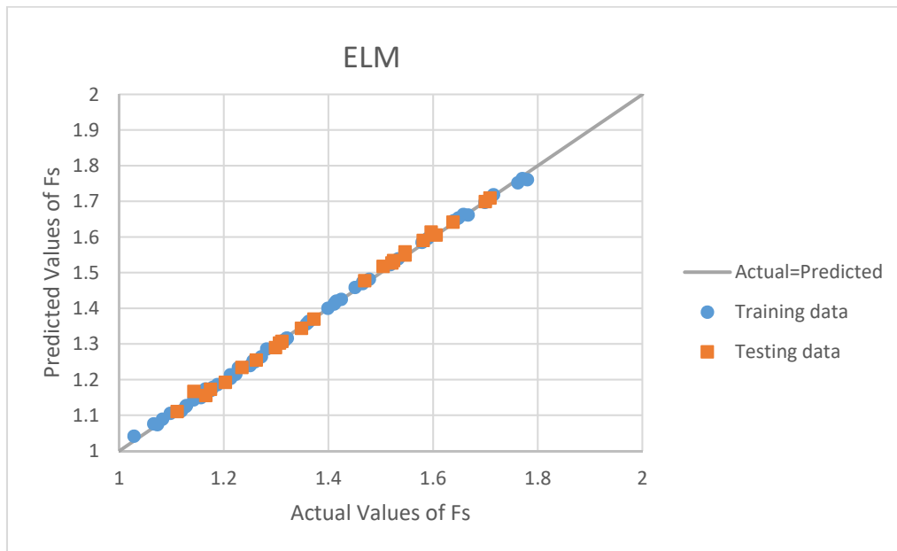
Figure (3): Actual vs. predicted values of training and testing data using ELM model
