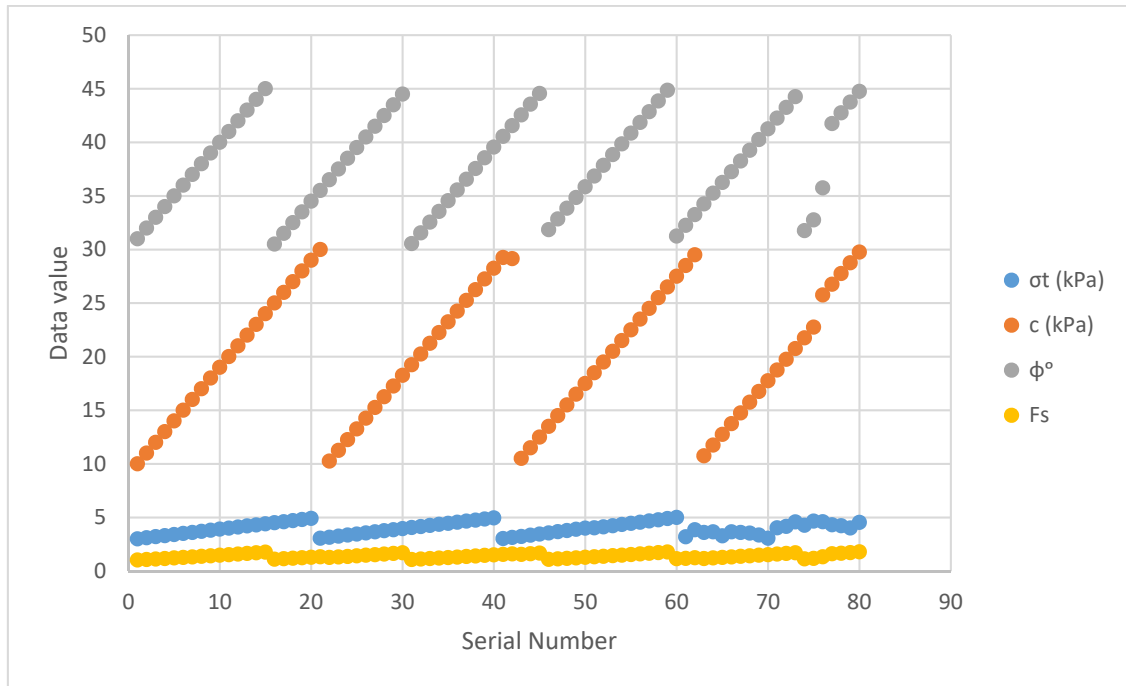
Figure (1): Graph representing datasets of \sigma_t (kPa), c (kPa), \phi^o and F_s
