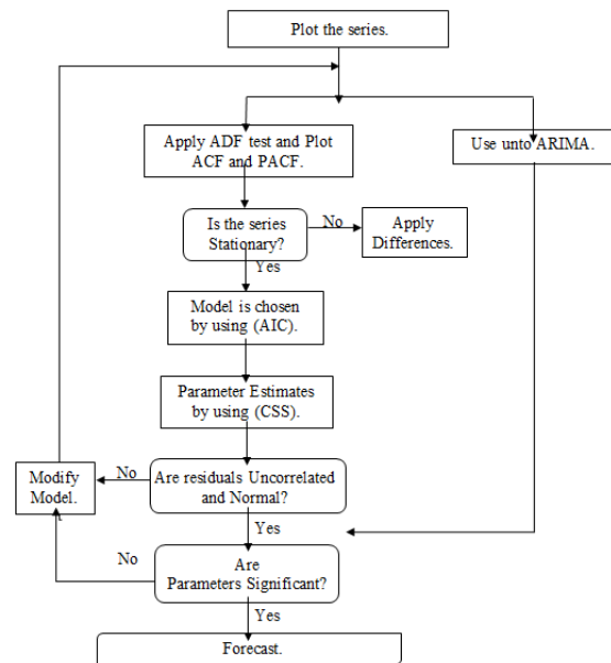
Figure (1): Box-Jenkins modeling steps
