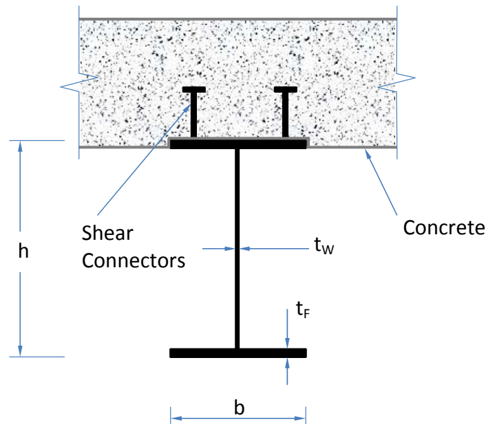
Figure (8): Cross-section through composite bridge girder
