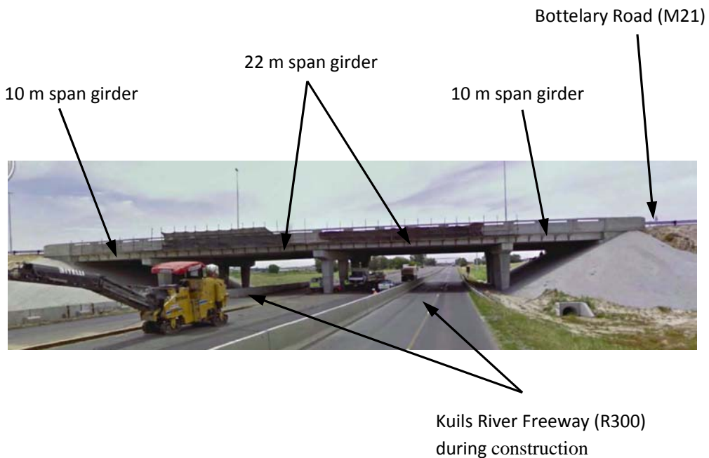
Figure (1): Widening of the M21 and the R300 during construction
