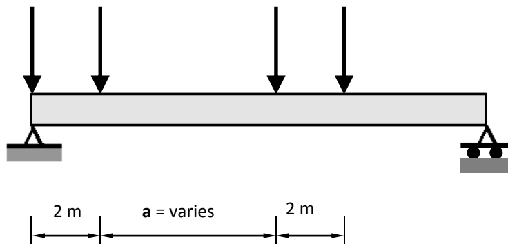
Figure (6): NB loading configuration
