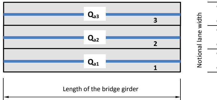
Figure (4): Effective length of each notional lane
