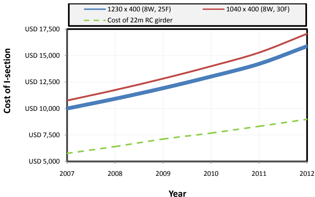
Figure (10): Cost of 22 m girders
