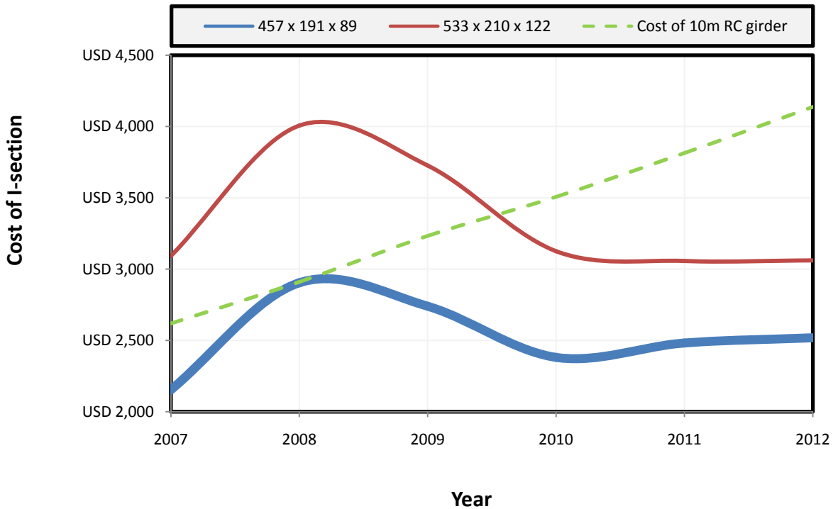
Figure (9): Cost of 10 m girders
