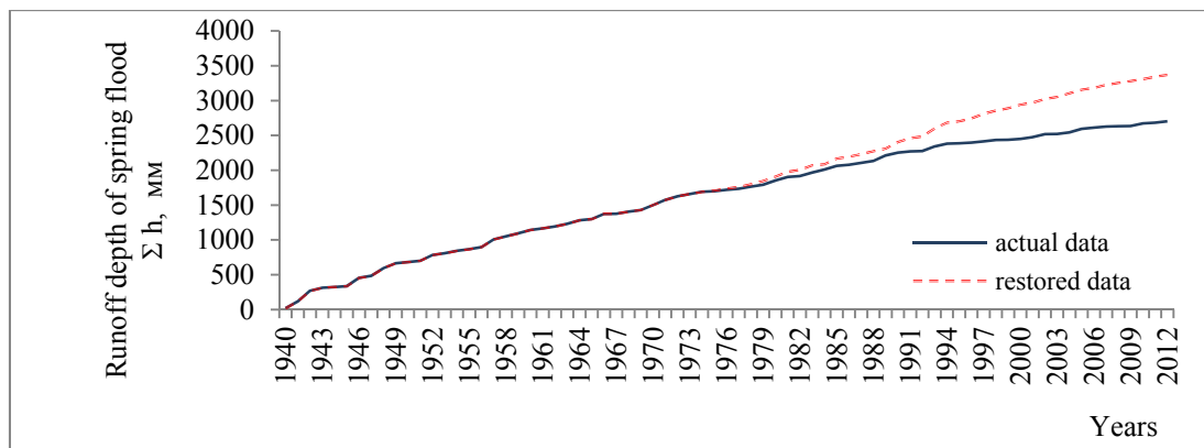
Figure (3): Total integral curve of runoff depth of the spring flood (h, mm): river Ilek in Aktobe
