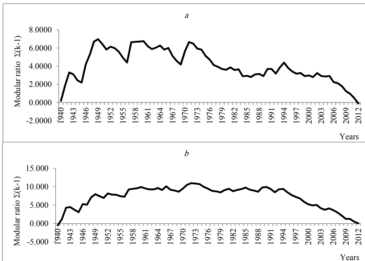
Figure (2): Integral curve of the runoff depth of the spring flood: a - river Zhayyk in Kushum village; b - river Ilek in Aktobe
