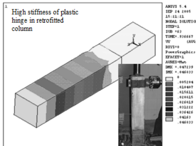
Figure (11): Contours of deformation on SP-C6 at 46.8 mm lateral displacement
