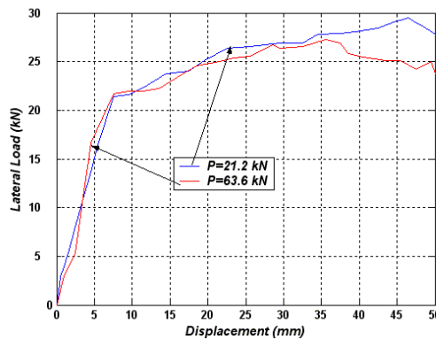
Figure (9): Capacity curves for columns designed according to ACI (318-02)
