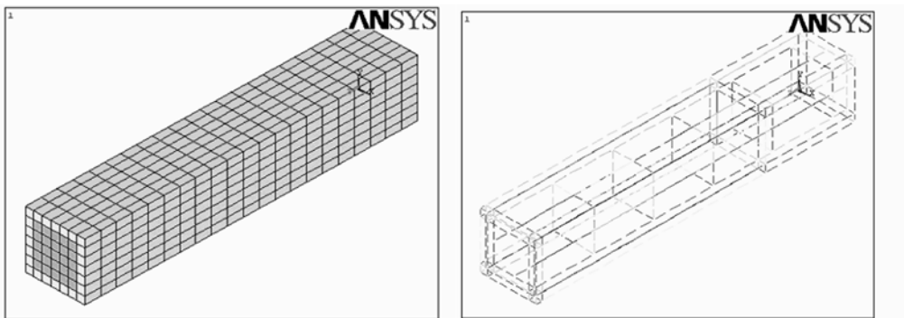
Figure (5): FE mesh of a column without FRP jacket
