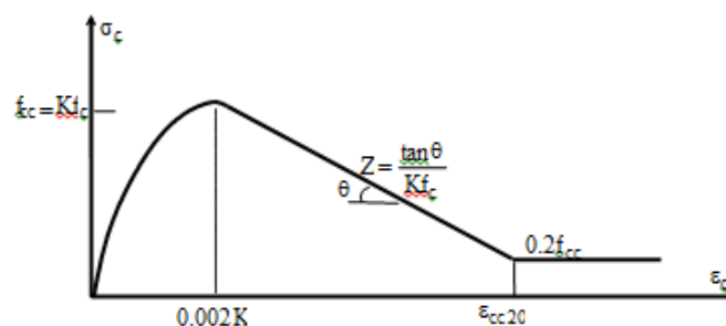
Figure (4): Stress-strain curve of confinement model for stirrup (Park et al., 1988)
