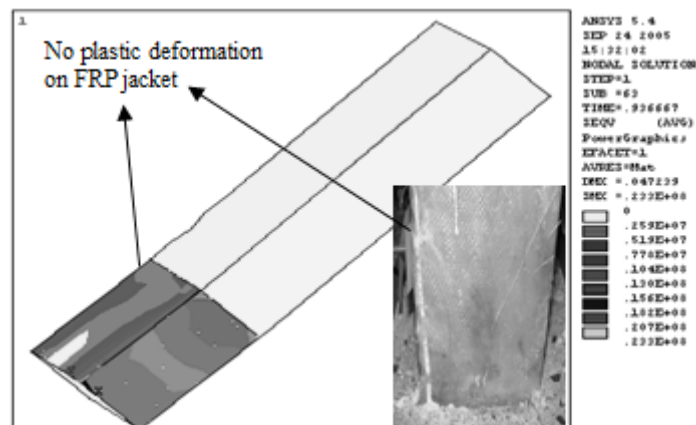
Figure (13): Contours of stress on SP-C7 based on Tsai-Wu criterion at 46.8 mm lateral displacement
