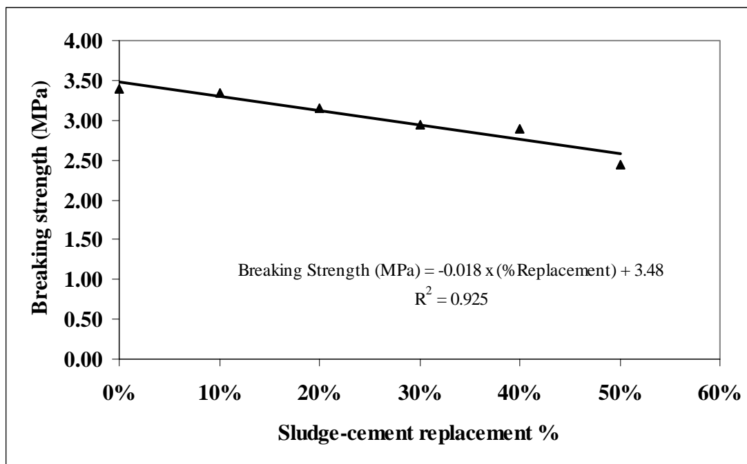
Figure 6: Average 28-day breaking strength of tiles versus percent sludge-cement replacements
