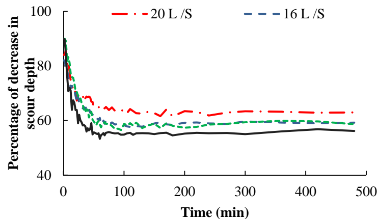
Figure (8): Time variation regarding the percentage of decrease in scour depth using nano-clays in unsteady flow
