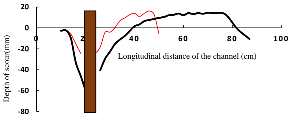
Figure (11): Comparison between scour depth profiles in control and original experiments at A flow rate of 20 L/s
