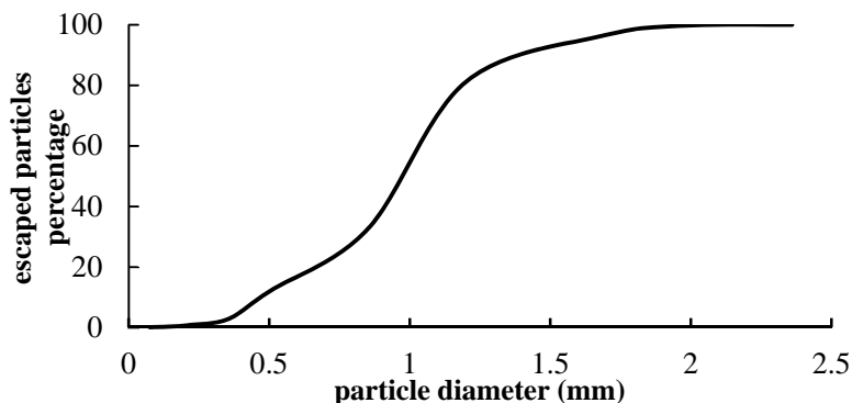
Figure (5): Sediment size curve
