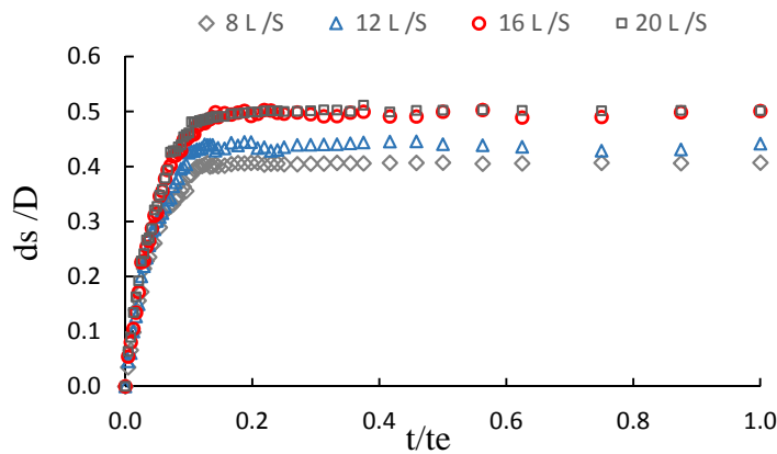
Figure (10): Time variation of scour depth in the vicinity of bridge piers in original experiments and unsteady flow condition
