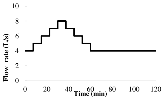
Figure (4): Triangular stepped hydrograph with peak flow rate of 8 l/s, a peak time of 30 min and a time step of 7.5 min
