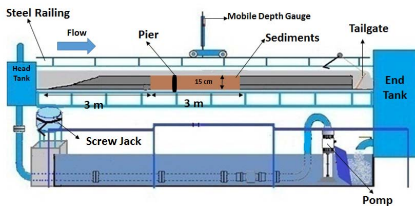
Figure (1): Sketch of the flume and its components
