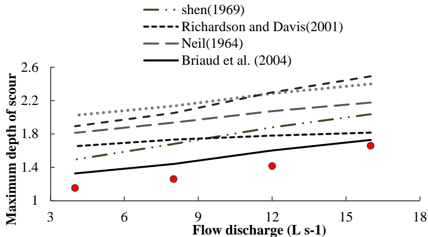
Figure (7): Comparison of scour maximum depth estimation between the formulae and experimental data in steady flow condition in control experiments
