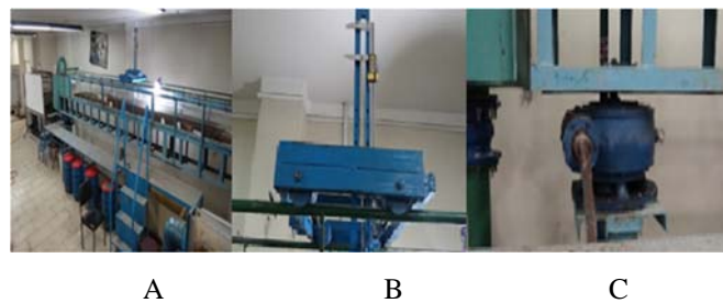
Figure (3): A. Channel used in experiment; B. Digital level gauge; C. Hydraulic jack
