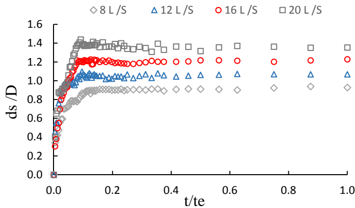
Figure (9): Time variation of scour depth in the vicinity of bridge piers in control experiments and unsteady flow condition
