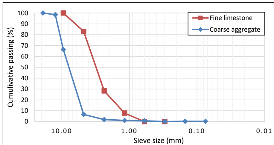
Figure (1): The coarse and fine aggregate gradients
