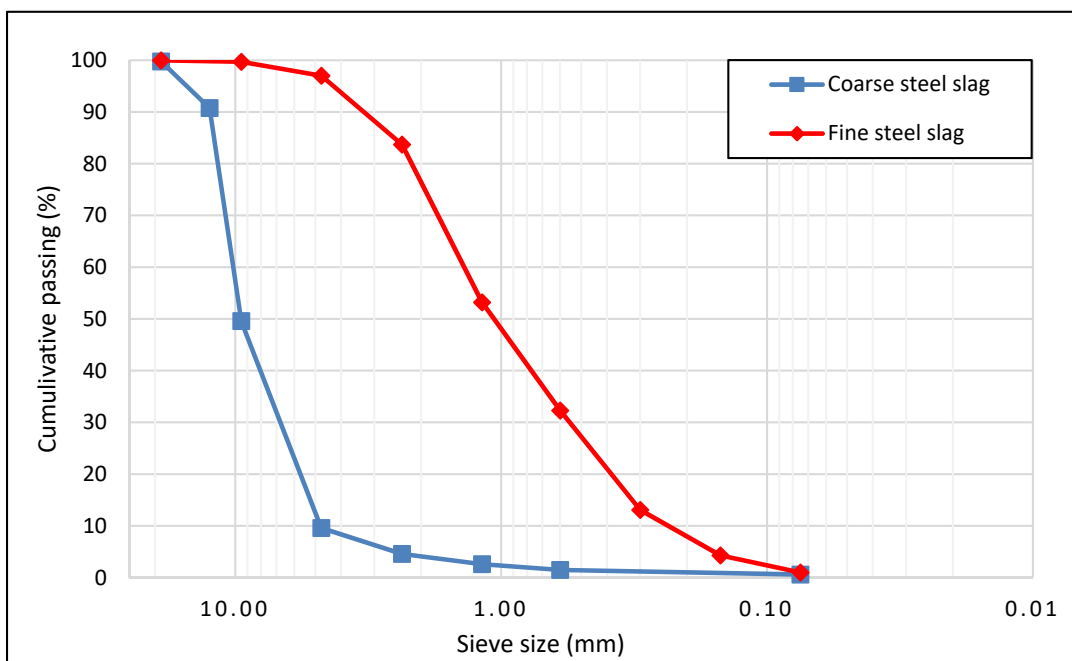
Figure (3): The SSA size analysis
