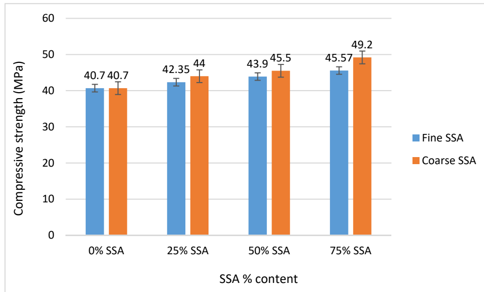
Figure (4): Average compressive strength results for concrete mixtures incorporating different SSA%
