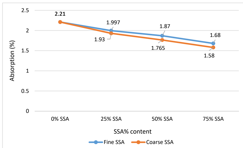
Figure (6): Water absorption results for concrete mixtures incorporating different SSA%
