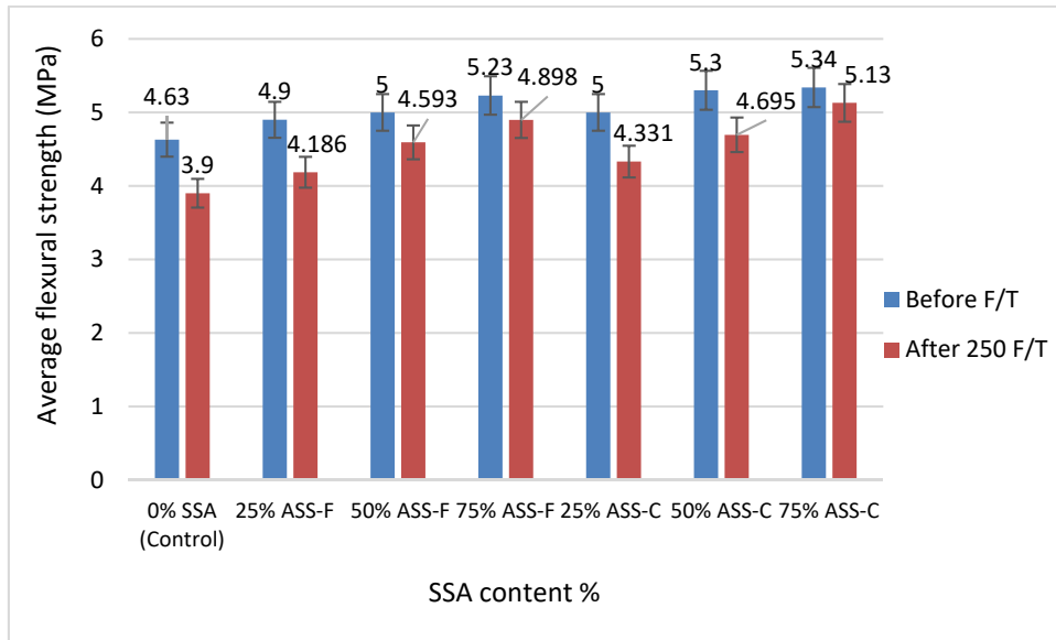
Figure (9): Average flexural strength of concrete specimens containing SSA% before and after 250 F/T cycles
