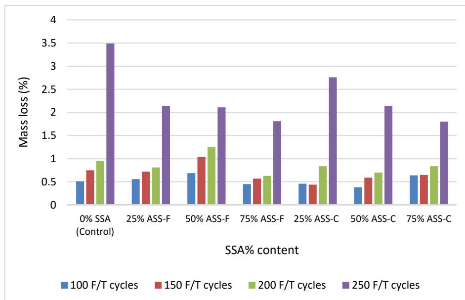
Figure (8): Average mass loss of concrete specimens containing SSA exposed to different F/T cycles
