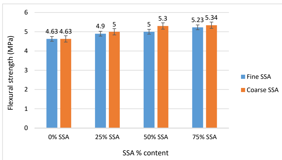
Figure (5): Average flexural strength results for concrete mixtures incorporating different SSA%
