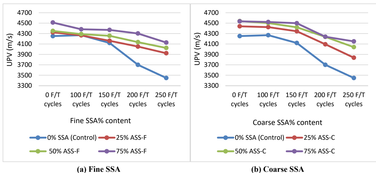
Figure (10): UPV of concrete specimens with different SSA% and under action of different F/T cycles: (a) Fine SSA; (b) Coarse SSA
