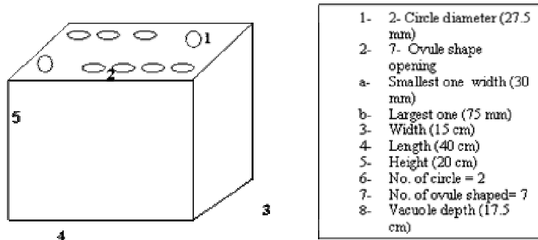
Figure (2): Produced 15 cm - building block features as referred to templates or mould matrix (weight 14.5 kg).
