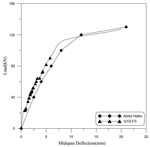
Figure (7): Load-deflection curve for beam BS2
