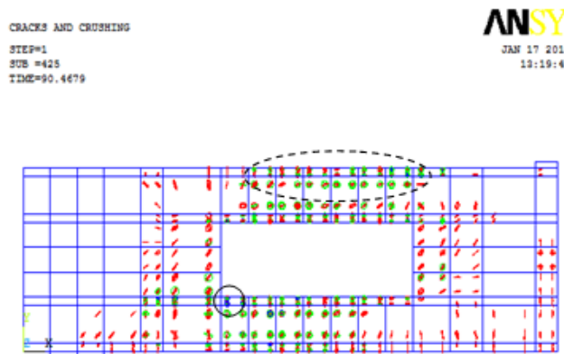
Figure (20): Crack pattern at a load of 90 kN for beam BS9
