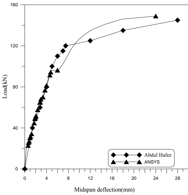
Figure (6): Load-deflection curve for beam BS1
