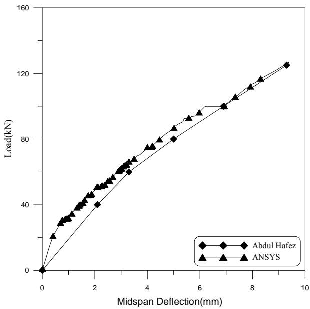
Figure (12): Load-deflection curve for beam BS9
