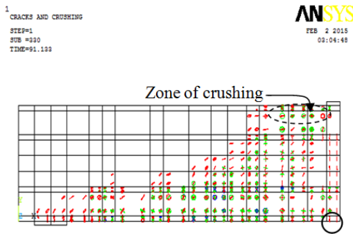
Figure (14): Crack pattern at a load of 90 kN for beam BS1
