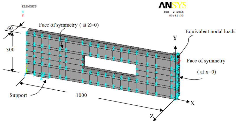
Figure (5): Finite element model adopted in the present work
