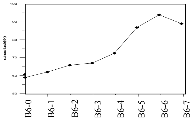
Figure (22): Effect of longitudinal steel configuration on ultimate load
