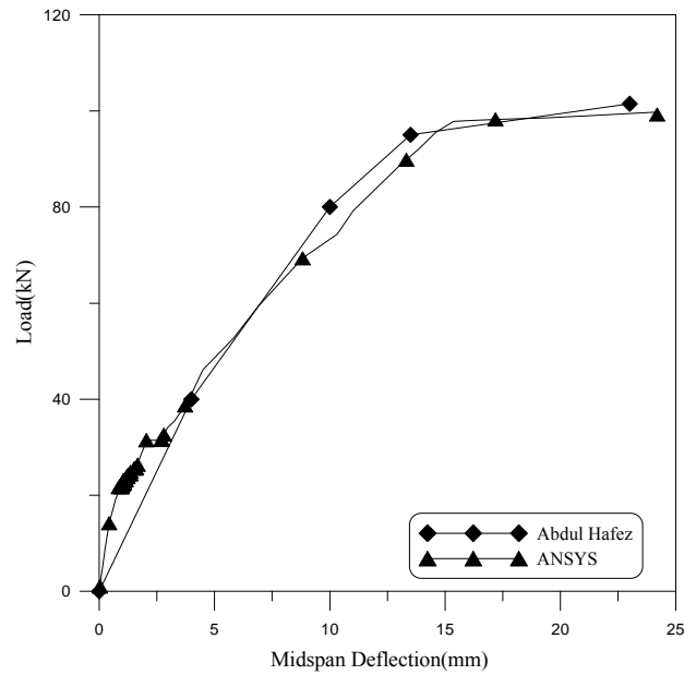
Figure (9): Load-deflection curve for beam BS4
