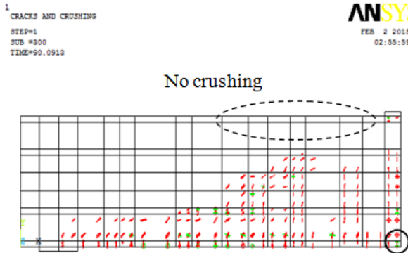
Figure (18): Crack pattern at a load of 90 kN for beam BS7
