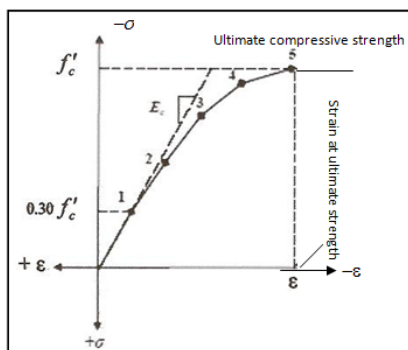
Figure (1): Uniaxial stress-strain curve for concrete
