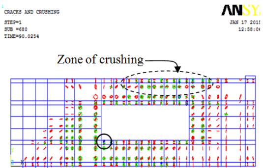
Figure (16) Crack pattern at a load of 90 kN for beam BS3
