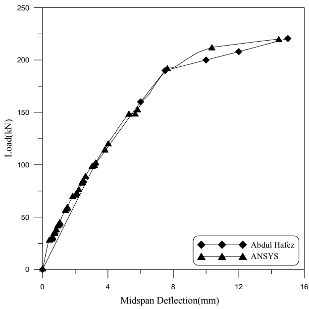
Figure (10): Load-deflection curve for beam BS7
