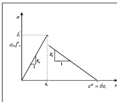
Figure (2): Tension stiffening model
