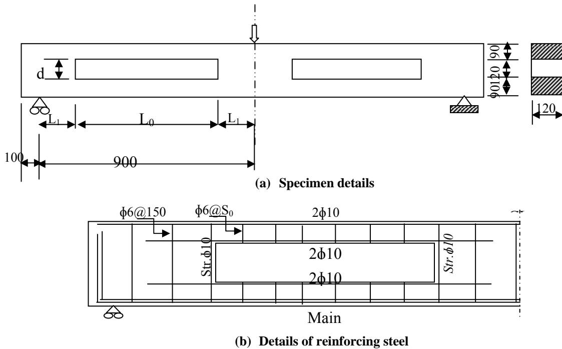
Figure (4): Specimen and reinforcing steel details (Abdul Hafez, 2009)
