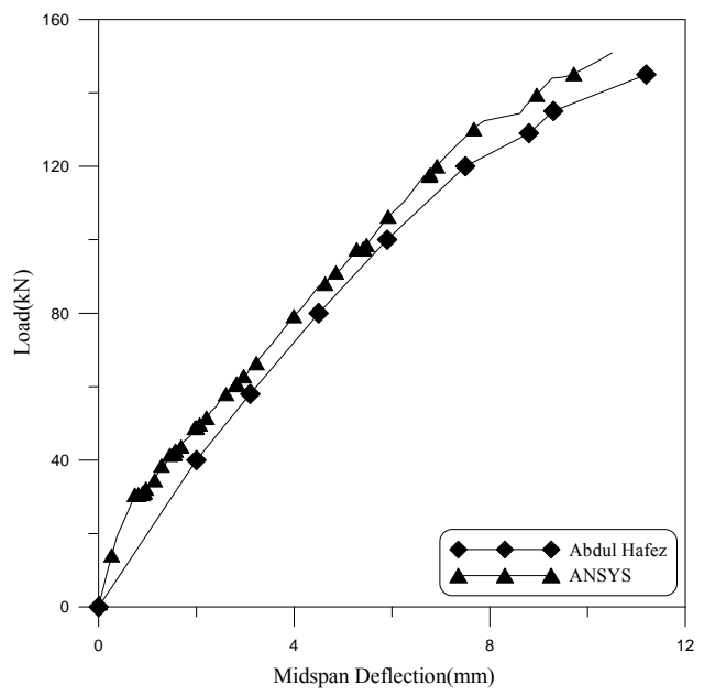
Figure (11): Load-deflection curve for beam BS8
