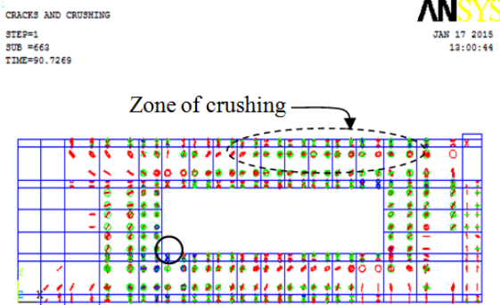
Figure (17): Crack pattern at a load of 90 kN for beam BS4
