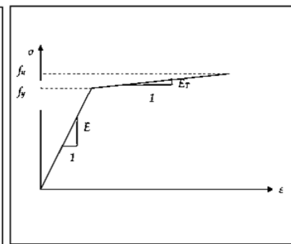
Figure (3): Uniaxial stress-strain relation for steel
