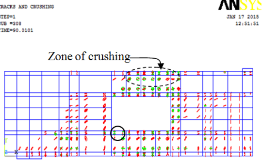
Figure (15): Crack pattern at a load of 90 kN for beam BS2
