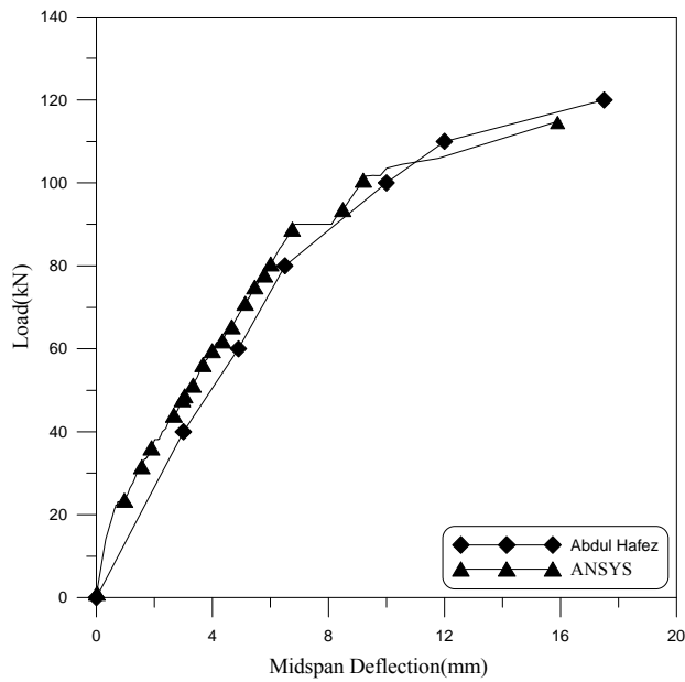
Figure (8): Load-deflection curve for beam BS3
