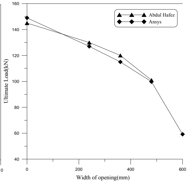
Figure (13): Effect of opening width on ultimate load capacity
