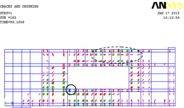
Figure (19): Crack pattern at a load of 90 kN for beam BS8
