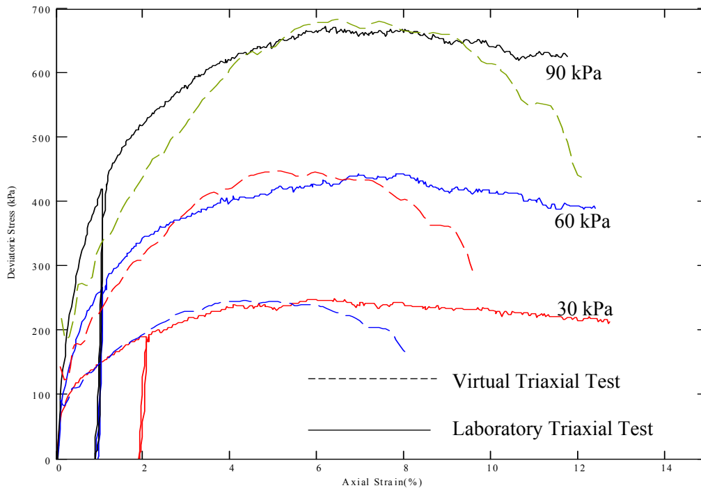
Figure 4: Comparison between Predicted and Measured Deviatoric Stresses for Crushed Limestone
