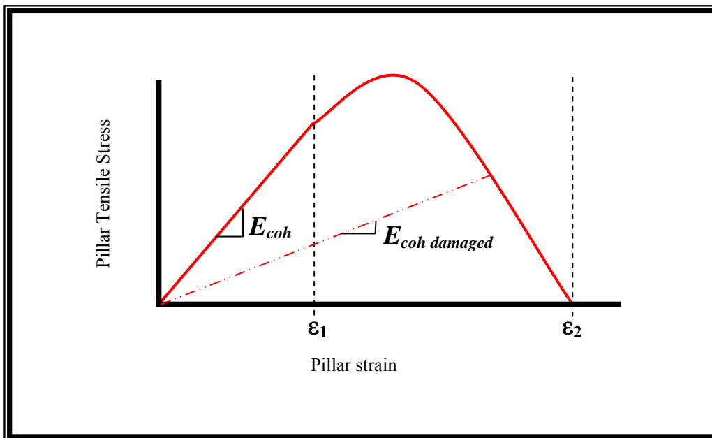
(b) Pillar Tensile Strength
