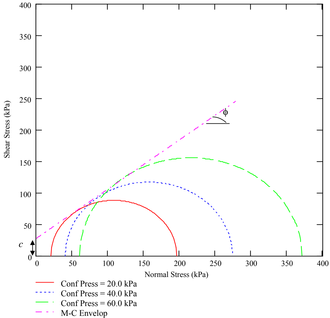
Figure 1: Classical M-C Failure Envelope Using Lab Triaxial Test on Silty Clay
