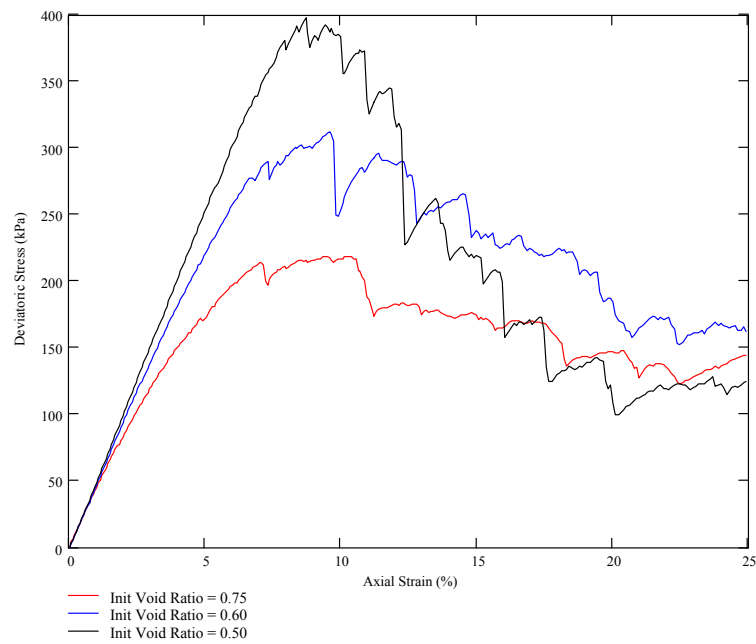
(a) Deviatoric Stress
