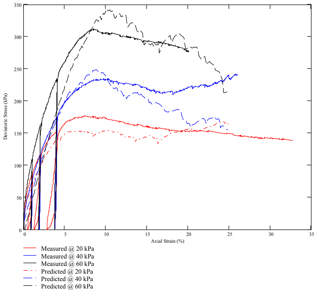
Figure 7: Comparison between Predicted and Measured Deviatoric Stresses for Silty Clay Using Friction and Cohesion Parameters
