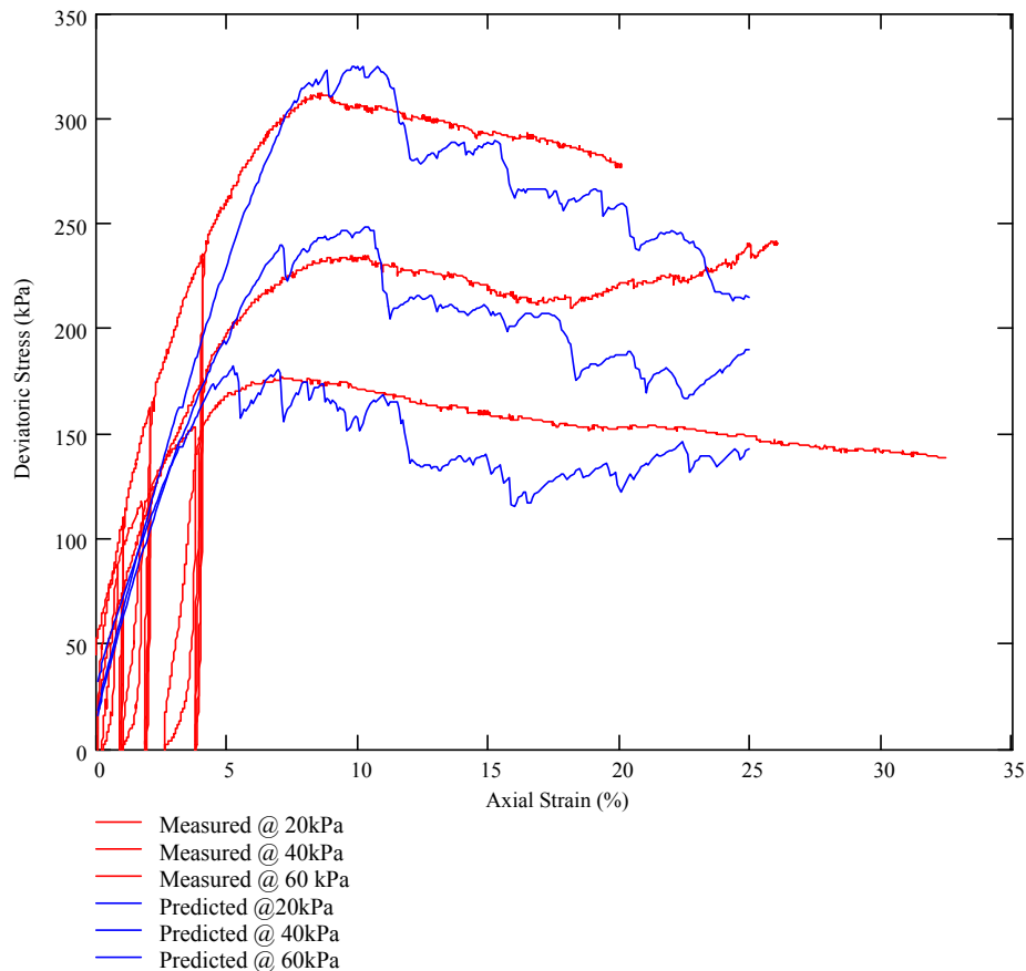
Figure 8: Comparison between Predicted and Measured Deviatoric Stresses for Silty Clay Using Zero-cohesion theory
