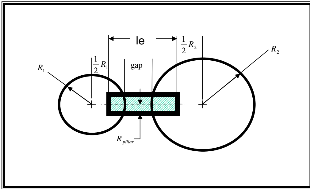
(a) Tensile Stress Pillar between Two Particles
