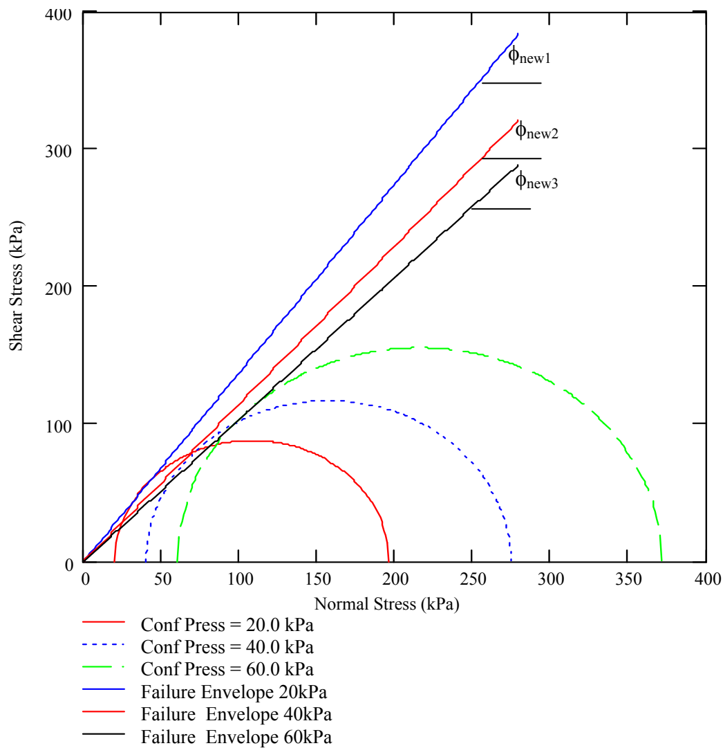
Figure 2: Confining Stress-Dependent Failure Envelope and Friction Angles for Silty Clay Using the Same Triaxial Tests
