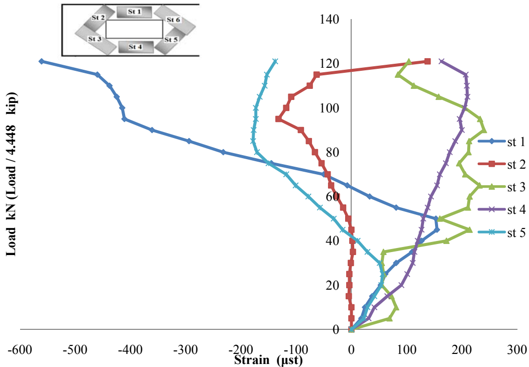
Figure (12): Load vs. strain curves of externally bonded steel plates for beam B3
