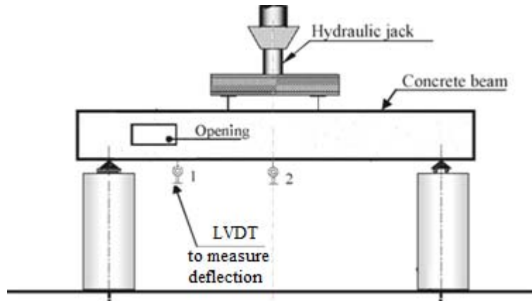
Figure (1): Test setup
