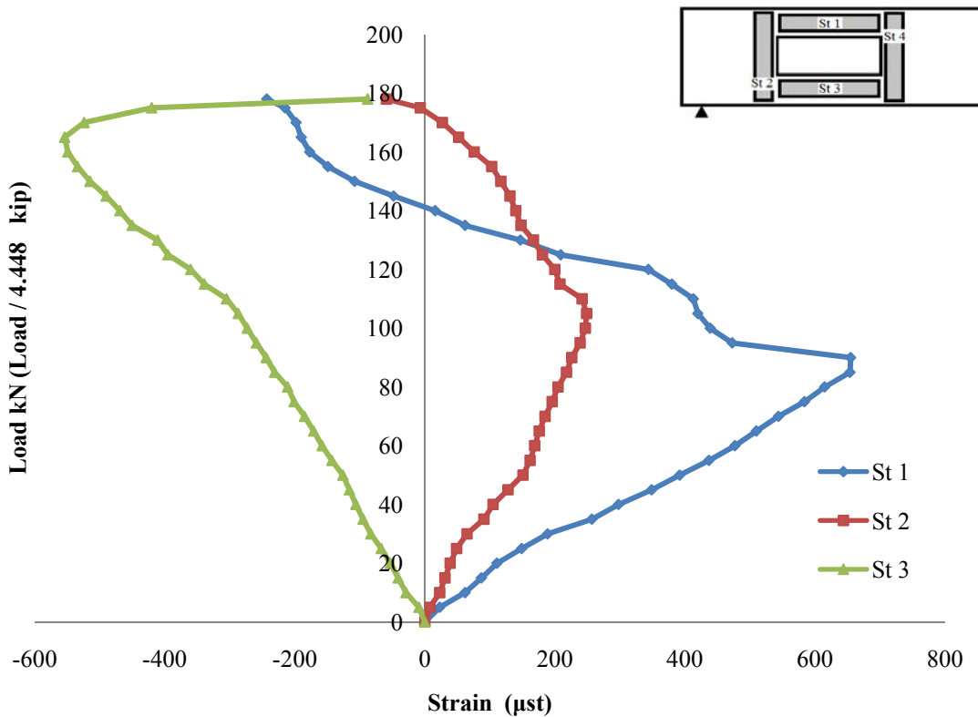
Figure (11): Load vs. strain curves of externally bonded CFRP plates for beam B2
