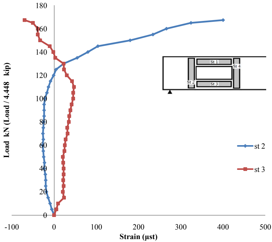
Figure (13): Load vs. strain curves of externally bonded steel plates for beam B4
