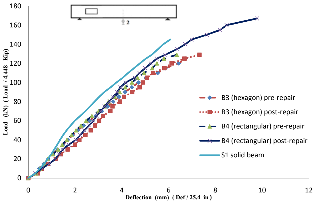
Figure (7): Load vs. deflection curves at the mid-span for beams repaired by steel plates
