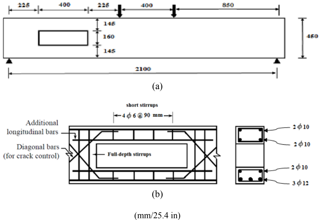
Figure (3): Beam description (a) Opening location (b) Steel reinforcement at the opening
