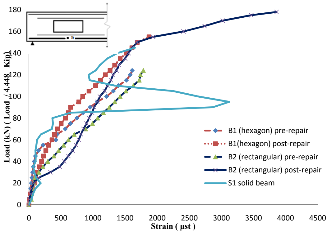
Figure (8): Load vs. steel bar strain curves at St for beams repaired by CFRP
