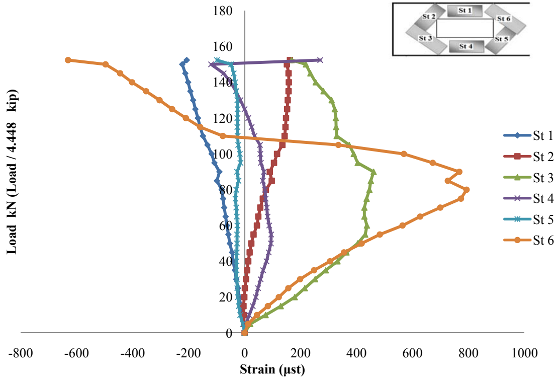
Figure (10): Load vs. strain curves of externally bonded CFRP plates for beam B1
