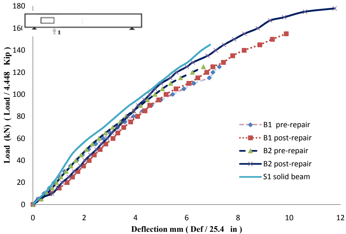
Figure (4): Load vs. deflection curves at the edge of the opening for beams repaired by CFRP
