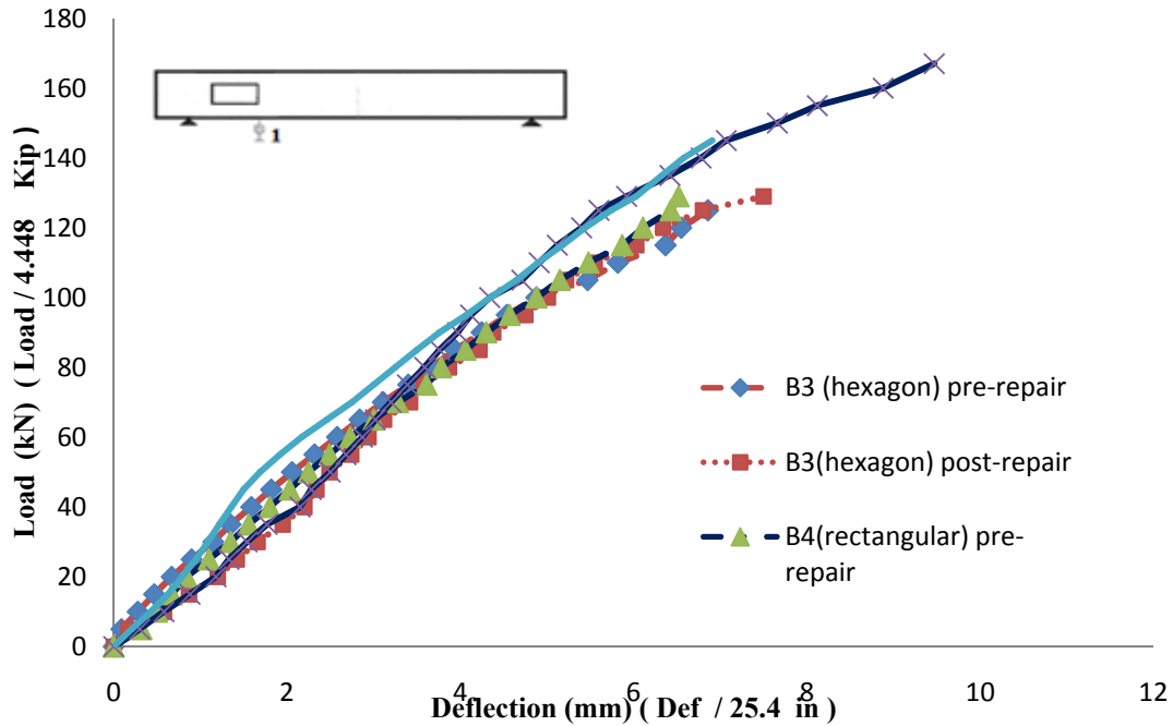
Figure (5): Load vs. deflection curves at the edge of the opening for beams repaired by steel plates
