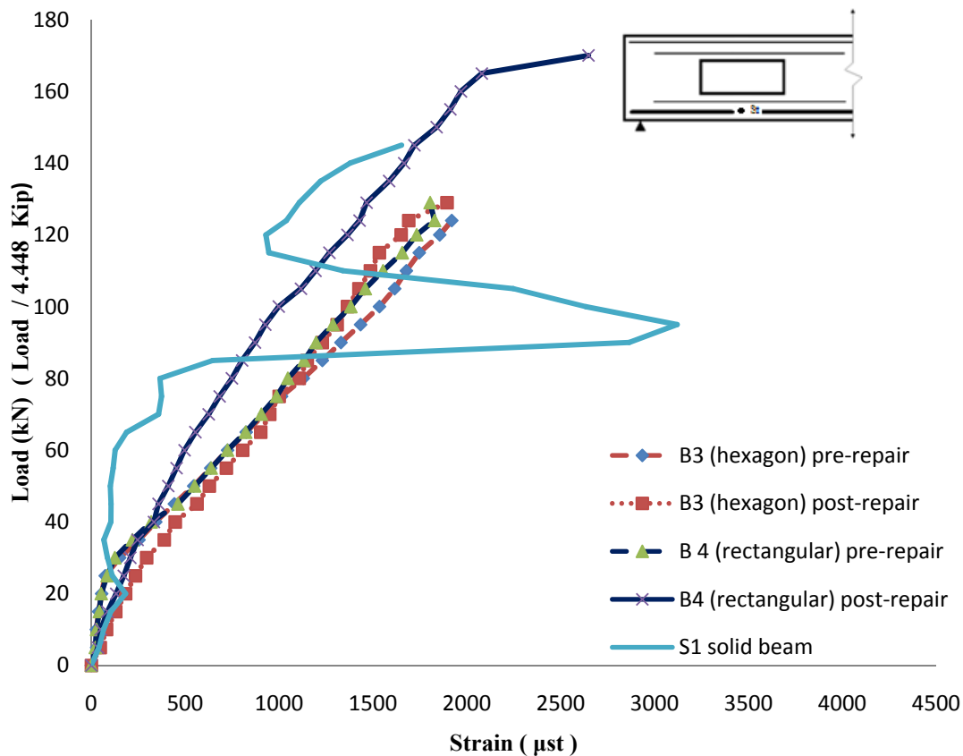
Figure (9): Load vs. steel bar strain curves at St for beams repaired by steel plates
