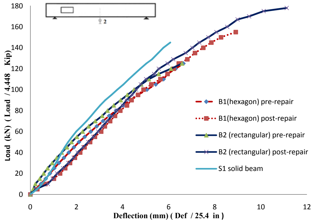
Figure (6): Load vs. deflection curves at the mid-span for beams repaired by CFRP
