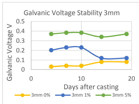
Figure (10): Galvanic voltage measurements on a number of days; electrode diameter = 3mm
