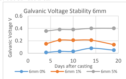
Figure (9): Galvanic voltage measurements on a number of days; electrode diameter = 6mm
