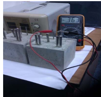
Figure (5): Electrical testing photos showing galvanic voltage measurement
