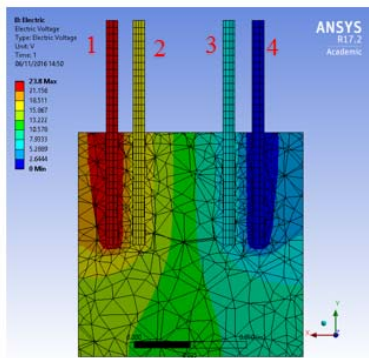
Figure (7): FEA cross-section showing the voltage contours in the 0% sodium chloride specimen
