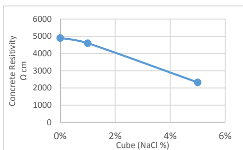
Figure (8): Concrete resistivity dropping with increase in sodium chloride concentration
