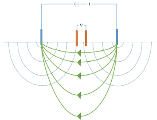
Figure (1): Four-electrode configuration following the Schlumberger- Palmer model. The solid green lines show the flow of current. Dashed blue lines show the electrical potential contours; blue electrodes-current; brown electrodes-voltage
