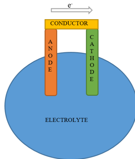
Figure (2): Requirements to form a galvanic pair
