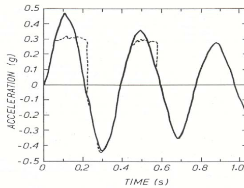
(b) Response after failure developed
