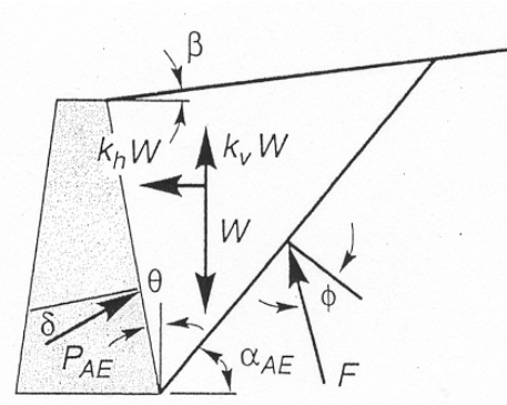
Figure (1): Forces acting on active wedge in Mononobe-Okabe analysis (Kramer, 1996)
