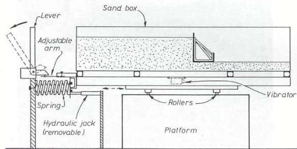
Figure (2): Experimental set-up for verification of the sliding block theory (Elms and Richards, 1990)
