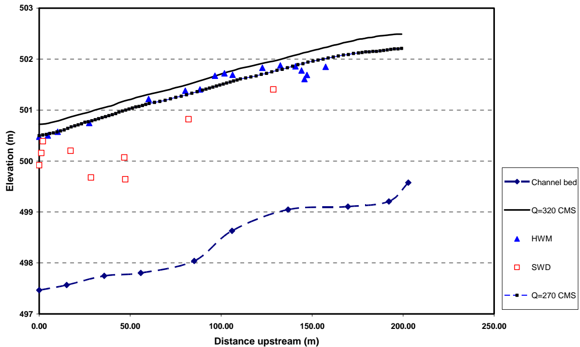
Figure 5: Paleoflood discharge estimates based on the high-watermarks of the February 2006 in Wadi Ouhadah subcatchment. Water-surface profiles were calculated using the HEC-RAS 4 open channel-flow model
