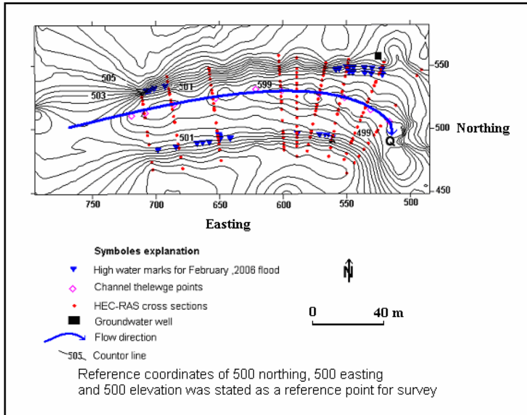
Figure 4: High-resolution topographic map of Wadi Ouhadah used for flood model estimation showing cross-section locations, high water marks and flow direction
