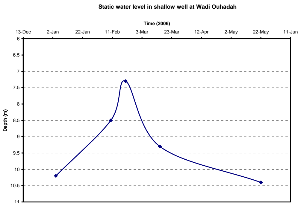
Figure 6: Depth from surface to water level at the shallow well in the lower reach of Wadi Ouhadah
