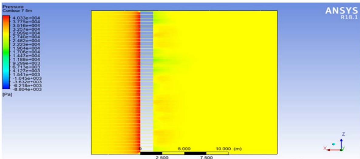
Figure (9): Pressure contour for a circular pier with an inlet rate of 5 m/s
