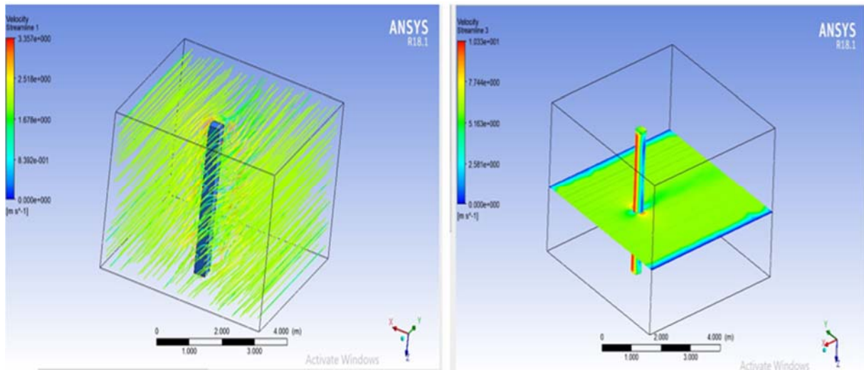
Figure (10): Velocity streamline for a square pier and a circular pier
