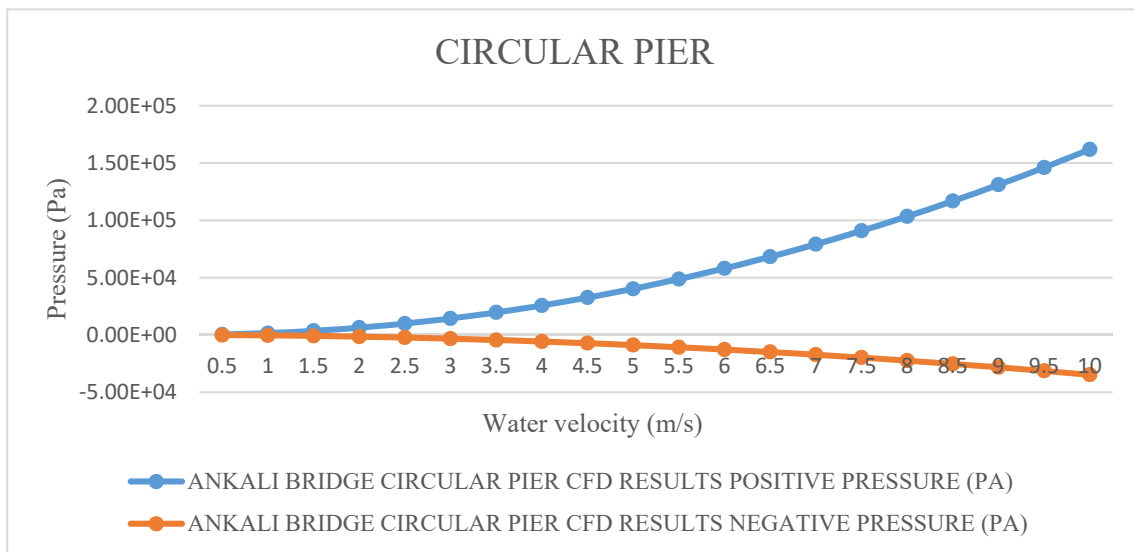
Figure (12): Circular pier C.F.D. positive pressure and negative pressure results
