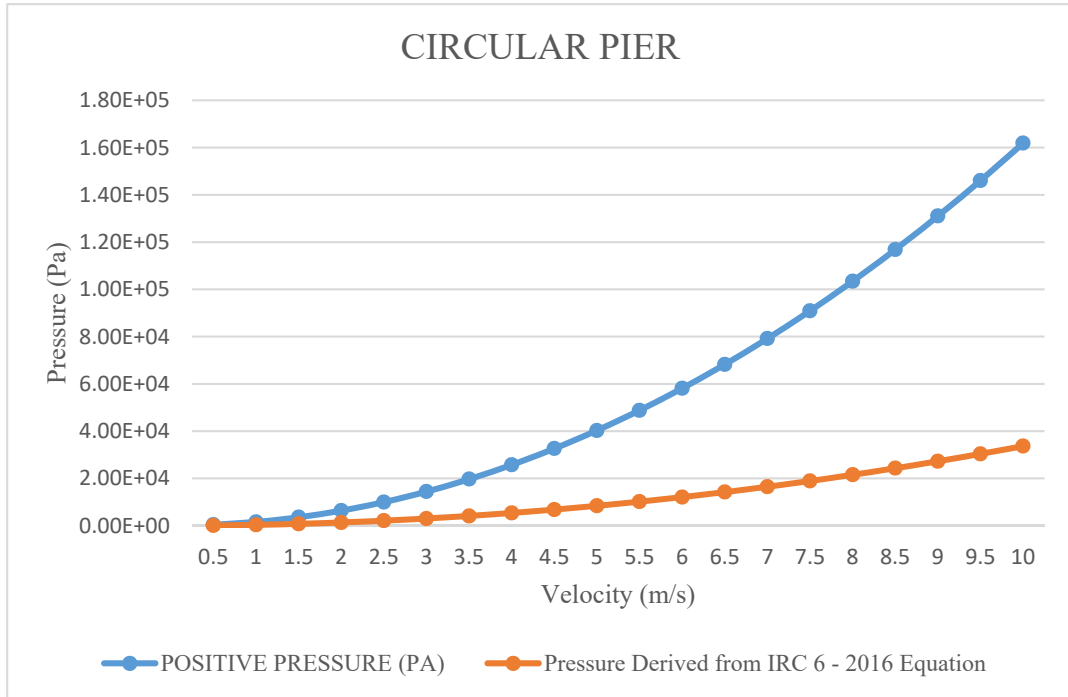
Figure (15): Comparison of circular pier C.F.D. positive pressure results with I.R.C. 6 code equation
