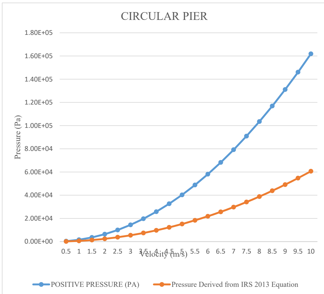
Figure (16): Comparison of circular pier C.F.D. positive pressure results with I.R.S. code equation
