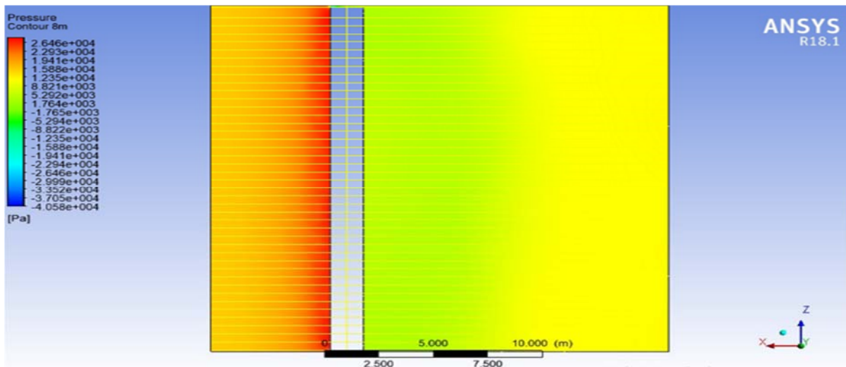
Figure (11): Pressure contour for a square pier with an inlet rate of 5 m/s
