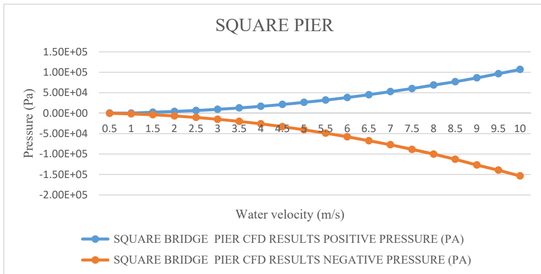
Figure (13): Square pier C.F.D. positive pressure and negative pressure results
