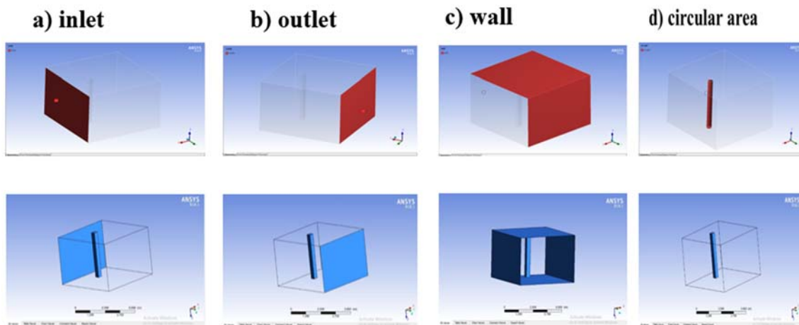
Figure (5): (a), (b), (c) and (d) represent the setup for boundary conditions in circular and square-shaped bridge piers
