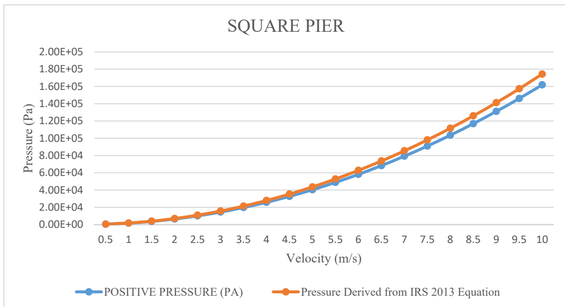
Figure (20): Comparison of square pier C.F.D. positive pressure results with I.R.S. code equation
