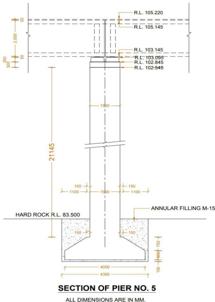
Figure (3): Section of newly constructed Ankali bridge pier no. 5 (P.W.D., Miraj)
