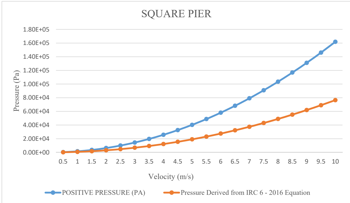
Figure (19): Comparison of square pier C.F.D. positive pressure results with I.R.C. 6 code equation
