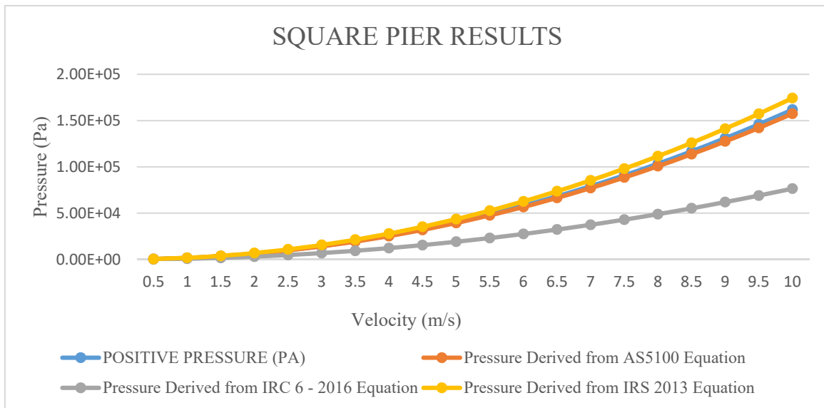
Figure (21): Comparison of square pier C.F.D. positive pressure results with various code equations
