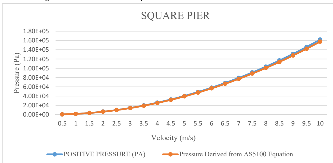
Figure (18): Comparison of square pier C.F.D. positive pressure results with AS5100 code equation
