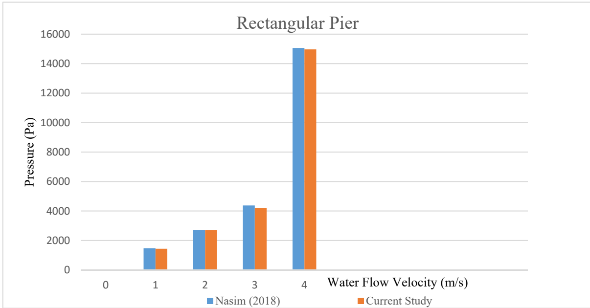
Figure (8): Pressure at the pier with the rectangular section vs. Maryam Nasim (2018) rectangular section pressure
