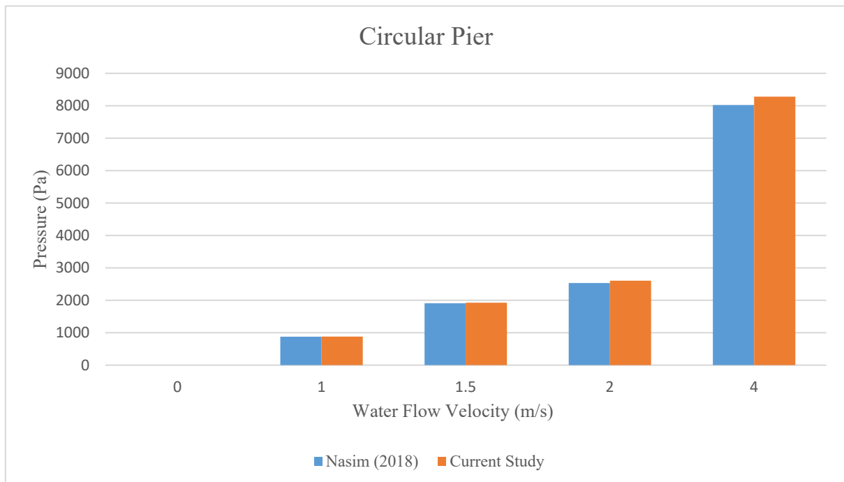
Figure (7): Pressure at the pier with the circular section vs. Maryam Nasim (2018) circular section pressure
