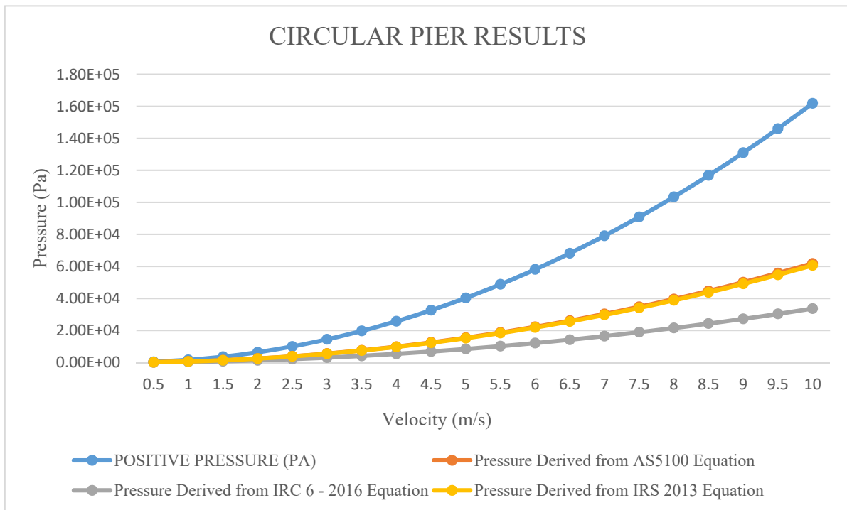
Figure (17): Comparison of circular pier C.F.D. positive pressure results with various code equations
