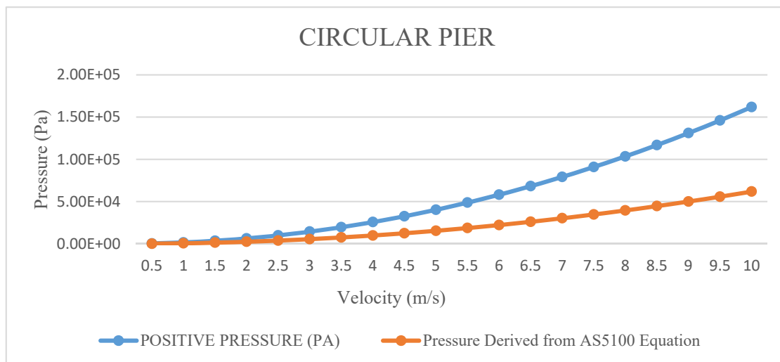
Figure (14): Comparison of circular pier C.F.D. positive pressure results with AS5100 code equation
