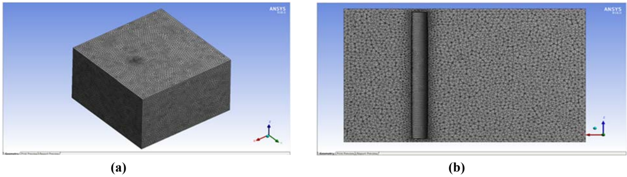
Figure (6): (a) Meshing setup for model pier (b) Meshing section of the circular pier
